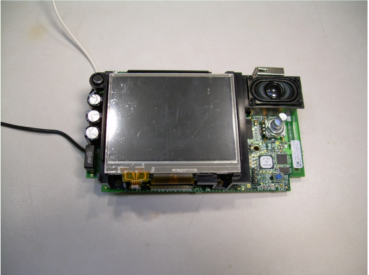
Front View of the TSG-3.8C2-x
