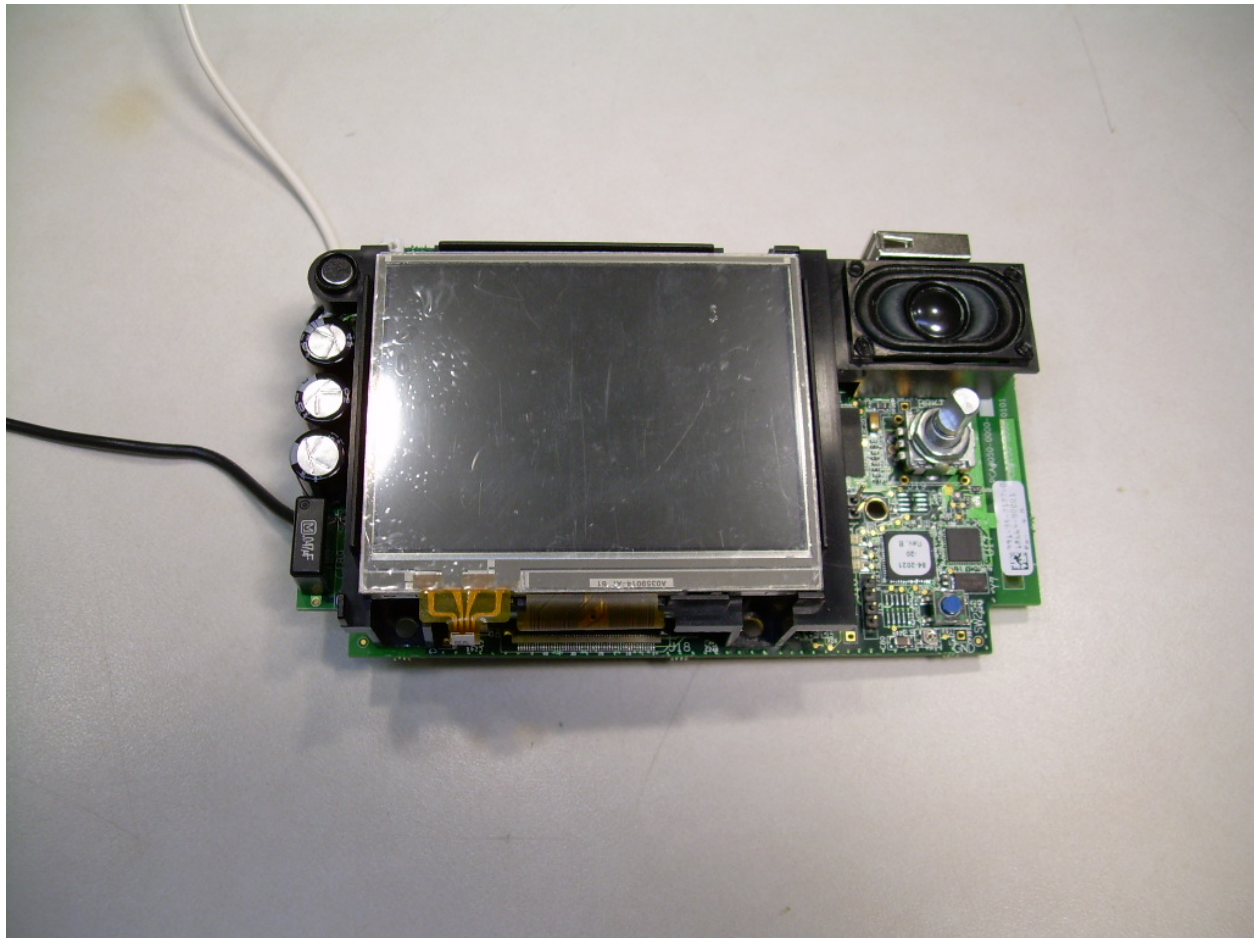
Photograph 5 - Front View of the TSG-3.8C2-x
