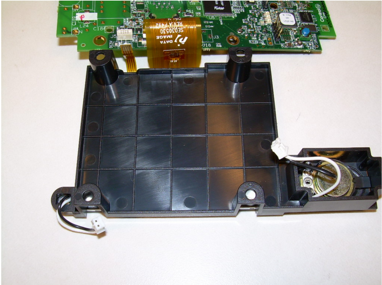
Photograph 13 - Back View of the Touchscreen
