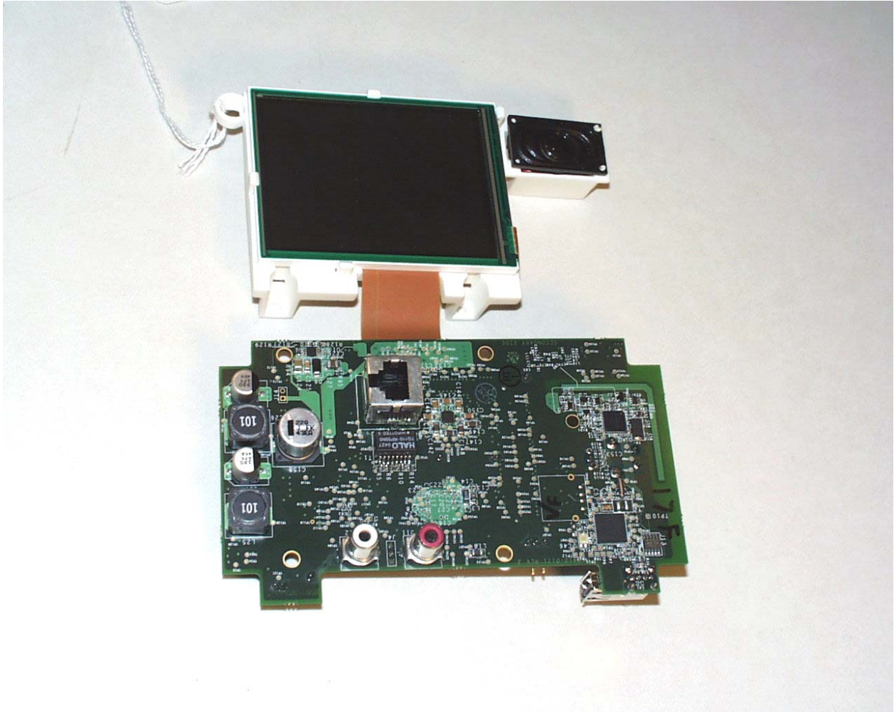
Photograph 4 - View of the Display and the Main Card
