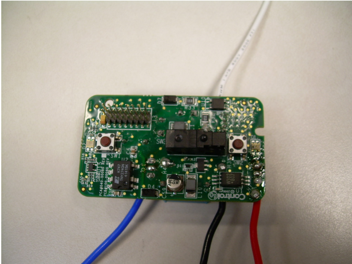
Photograph 8 - View of the Front Side of the C4-TDIM1-Z PCB
