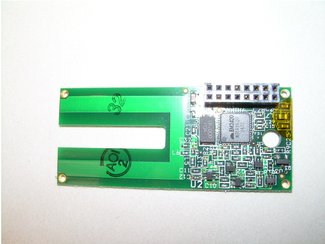
Photograph 11 - View of the Back Side of the Transceiver PCB
