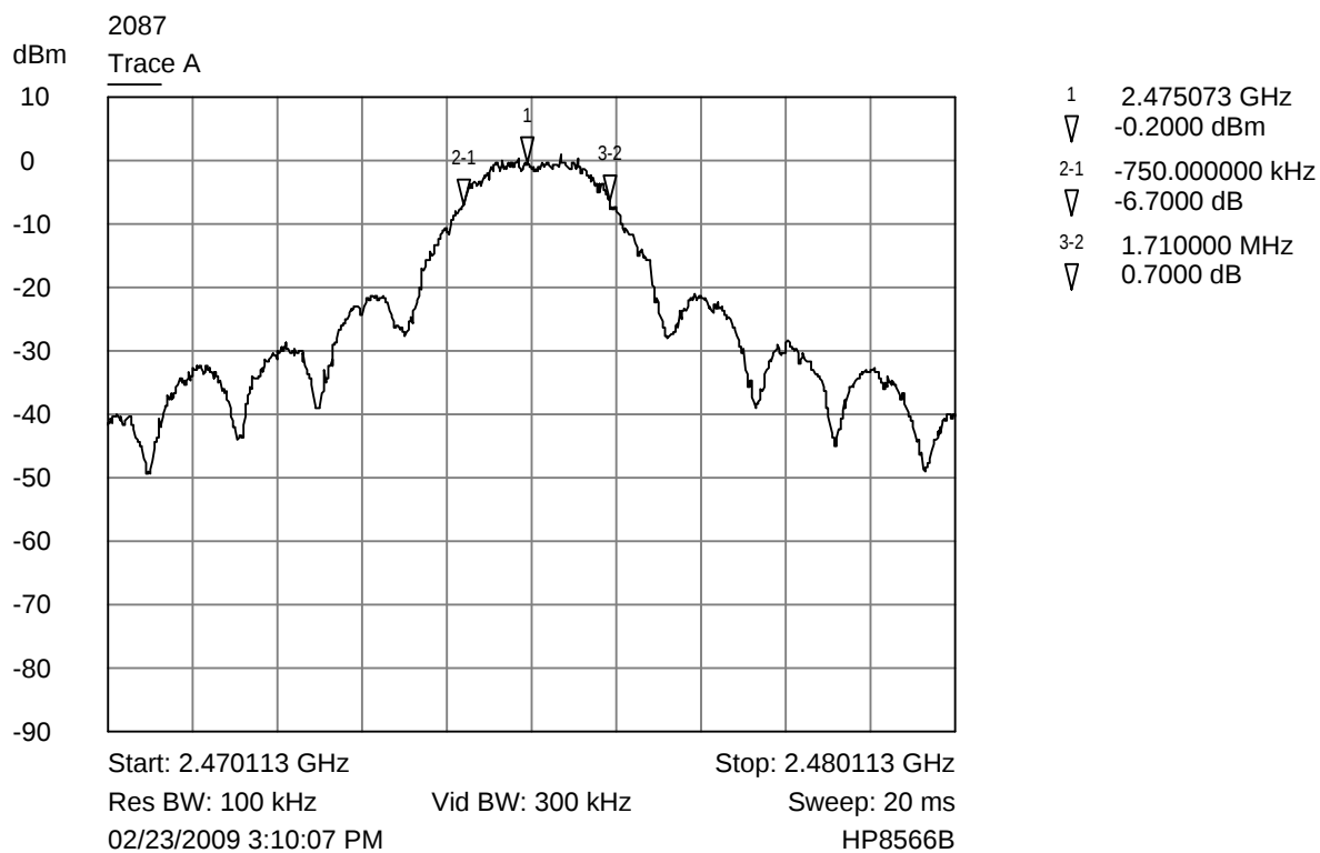
Trace A upper channel bandwidth plot
