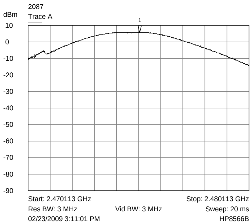
Trace A upper channel output power plot
