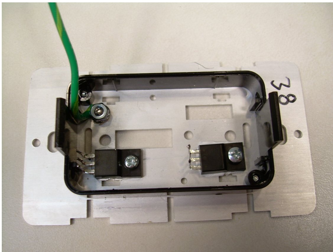
Photograph 9 - View of the MOSFETs of the EUT
