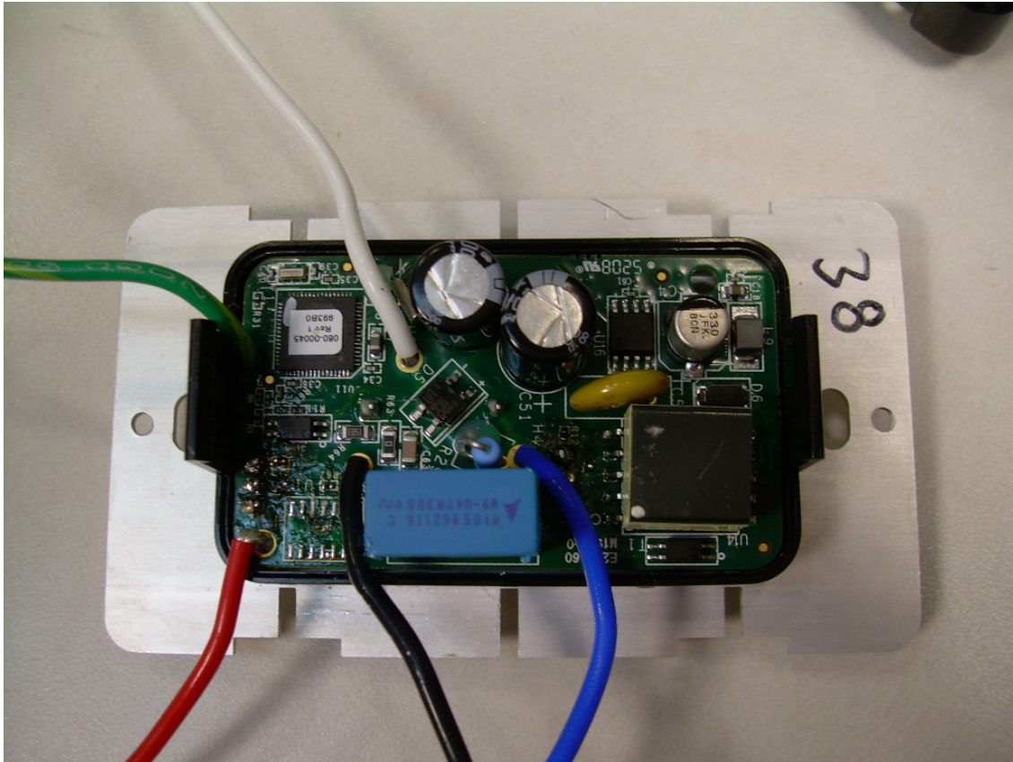
Photograph 7 - View of the Back Side of the C4-TDIM1-Z PCB
