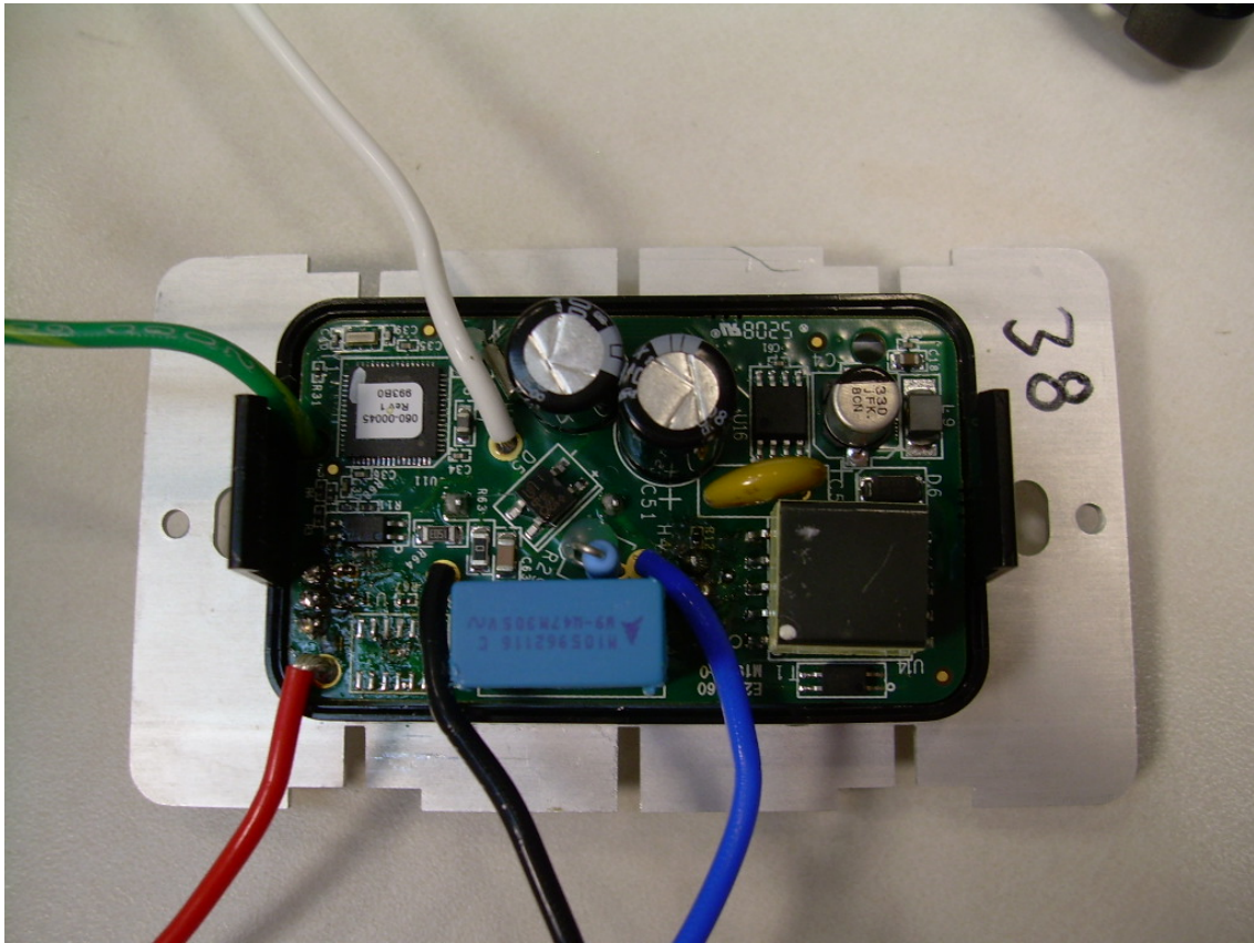
View of the Back Side of the C4-TDIM1-Z PCB
