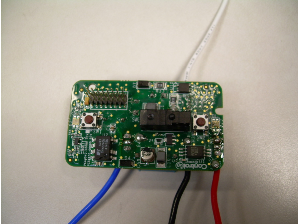
View of the Front Side of the C4-TDIM1-Z PCB
