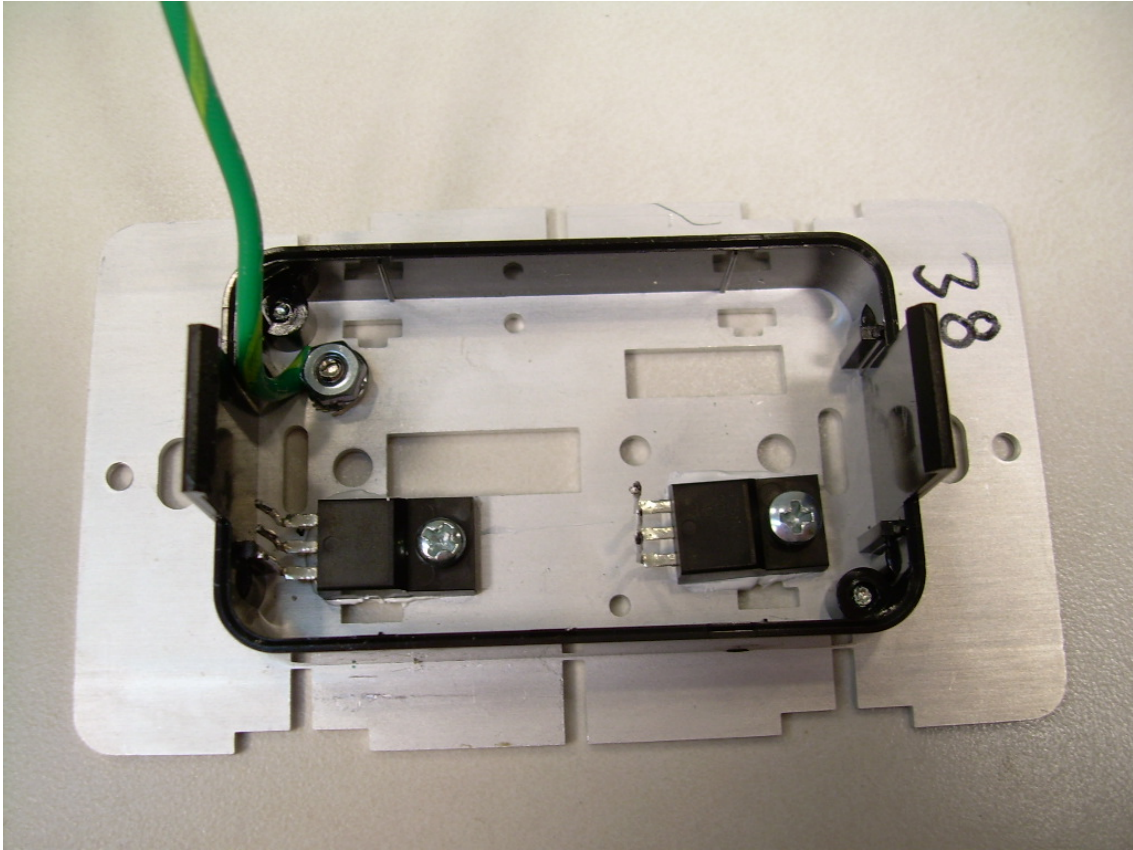
View of the MOSFETs of the EUT
