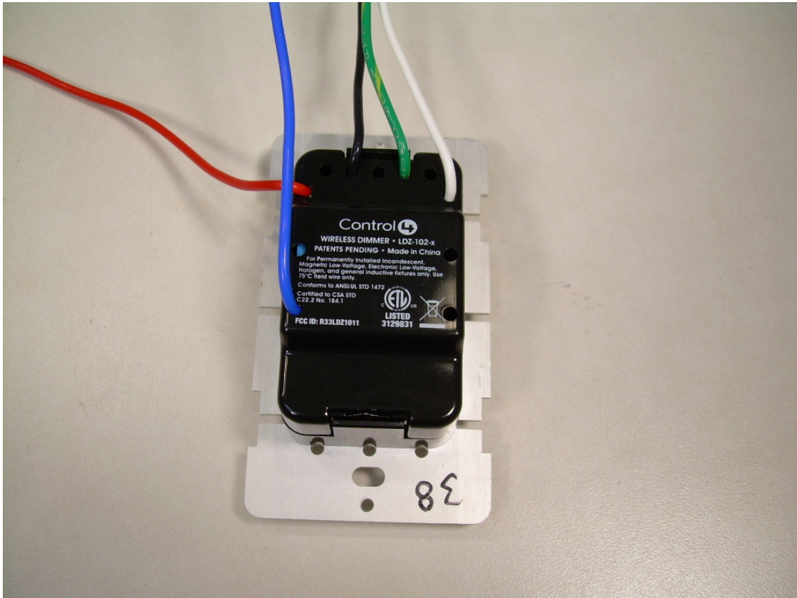
Back View of the C4-TDIM1-Z
