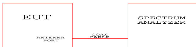
Test Configuration Block Diagram
