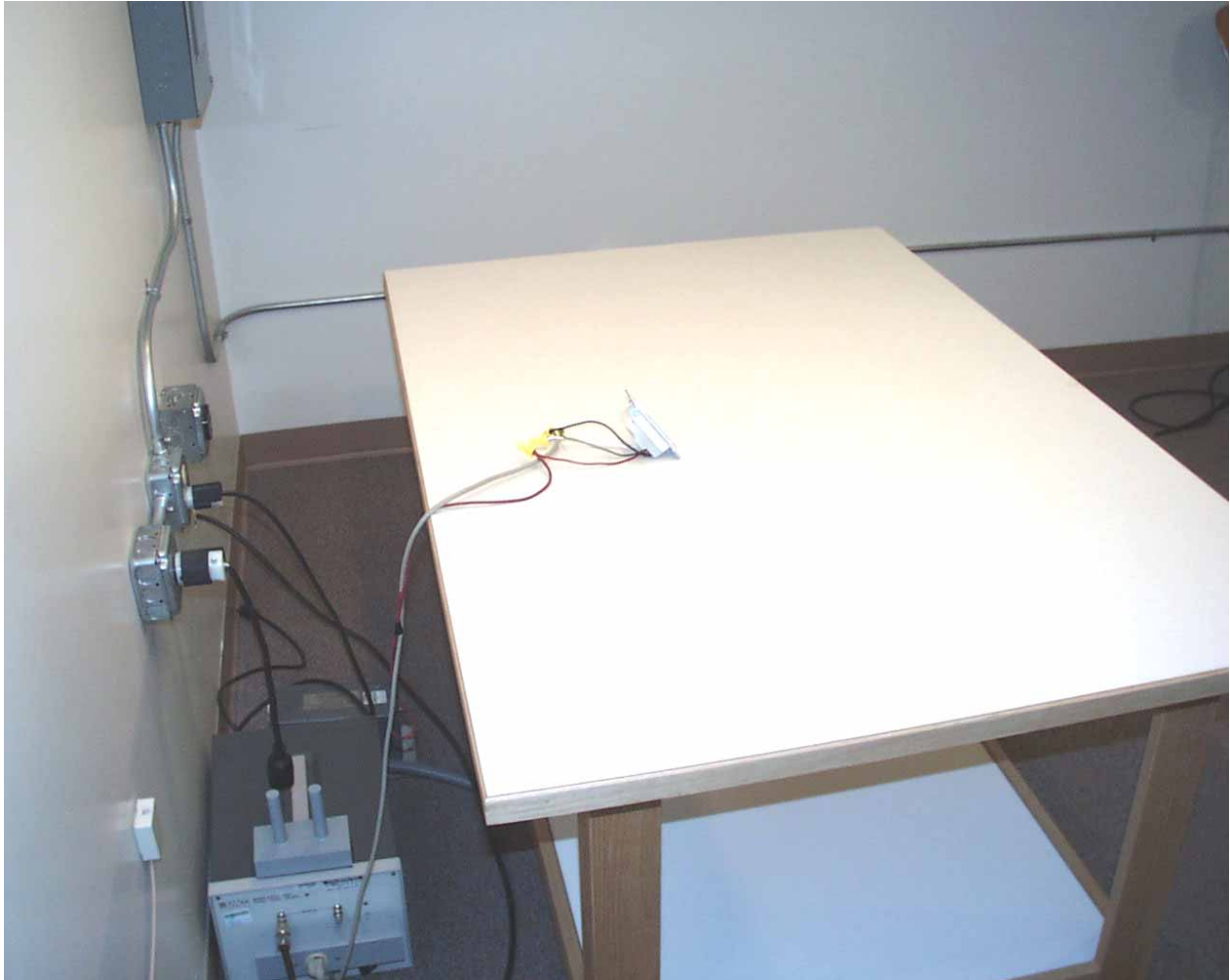
Photograph 6 - Back View Conducted Disturbance Worst Case Configuration
