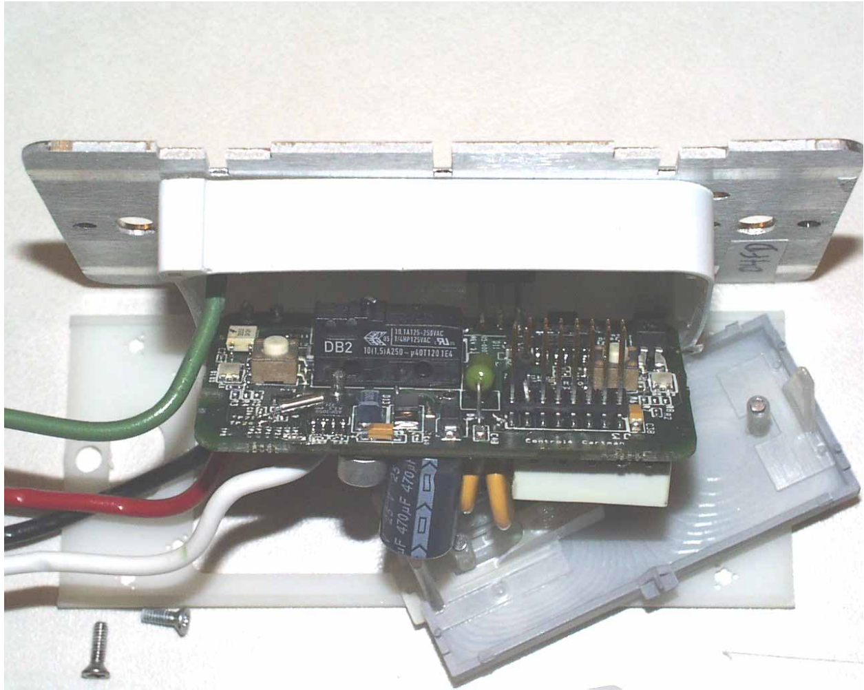
Photograph 10 - View of Side B of the Host Card
