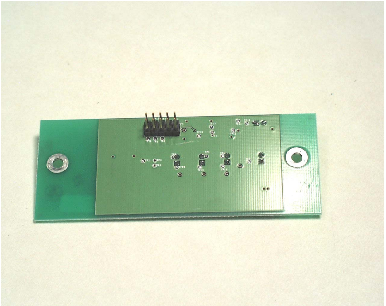
View of the Trace Side of the Front Panel PCB
