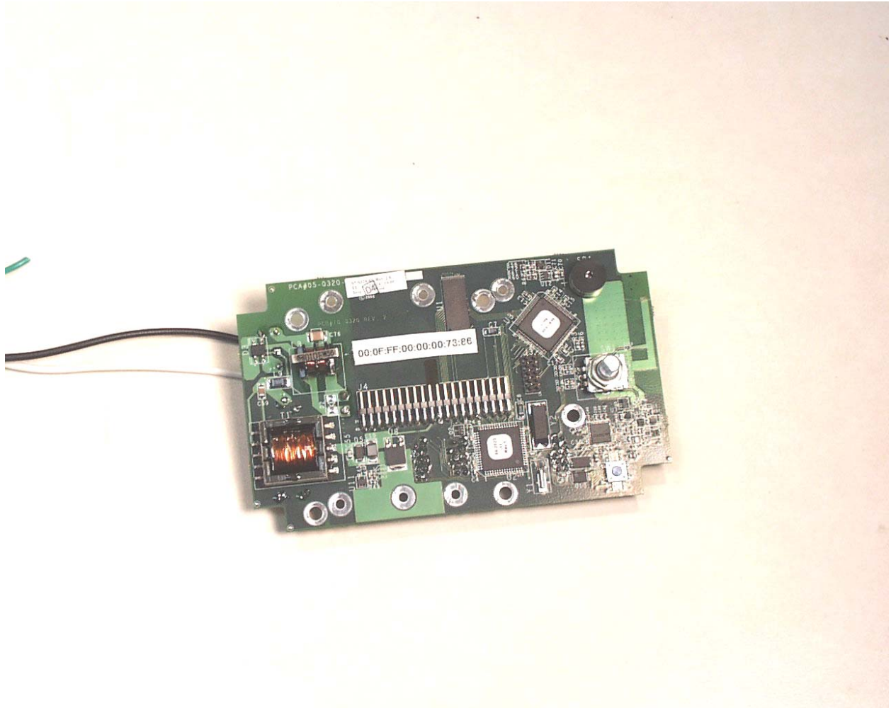
Photograph 9 - Front View of the Main PCB
