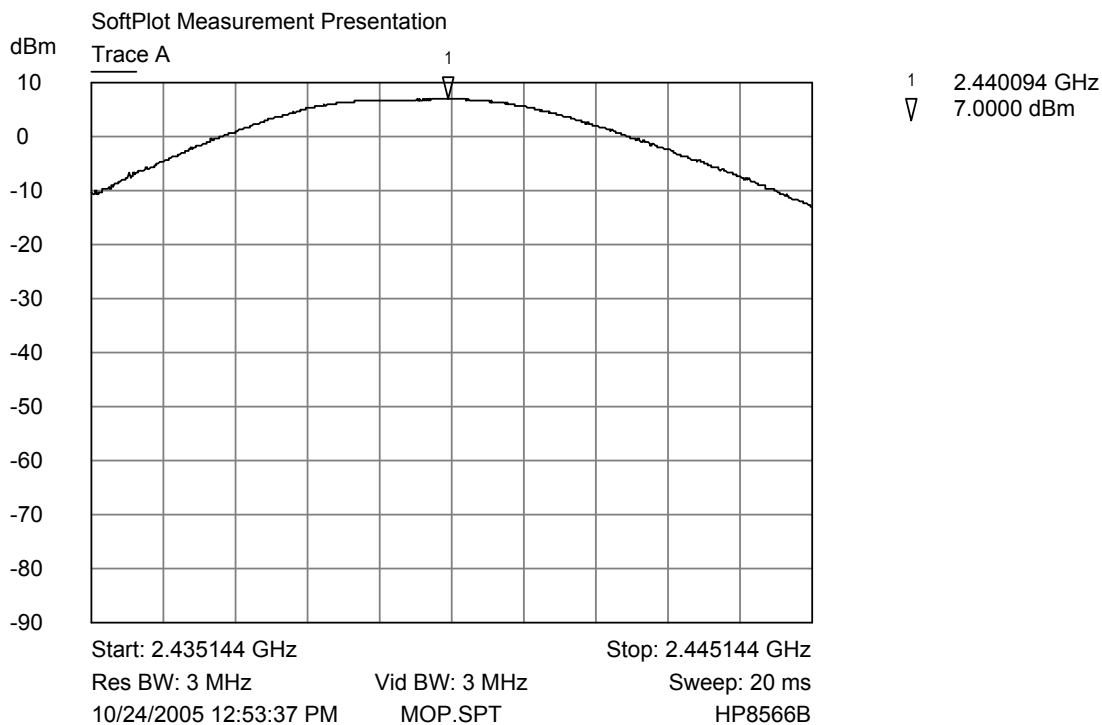
Trace A Middle channel output power plot
