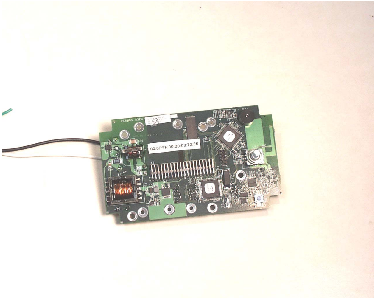
Front View of the Main PCB
