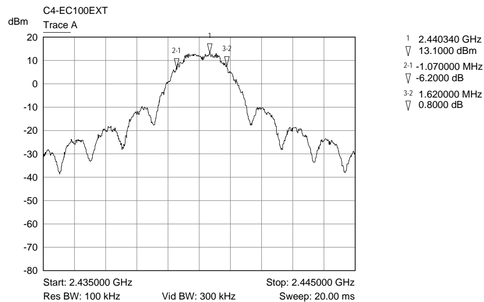
Trace A middle channel band width plot
