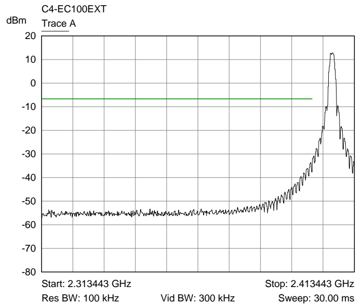
Trace A lower channel lower band edge plot
