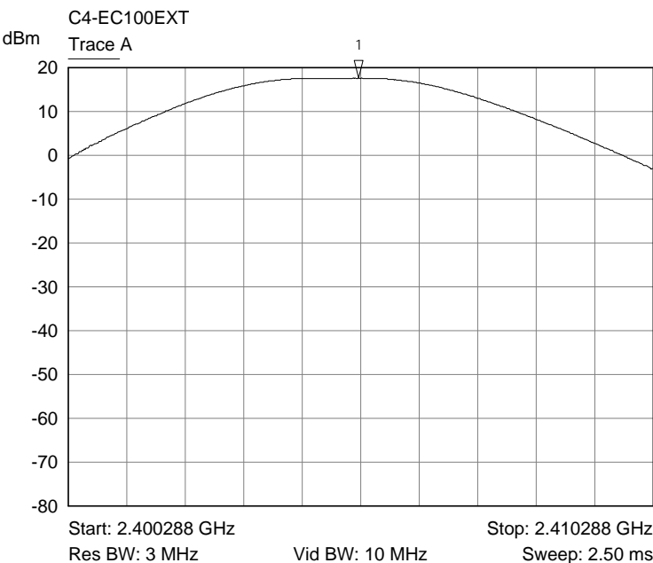
Trace A Lower channel output power plot
