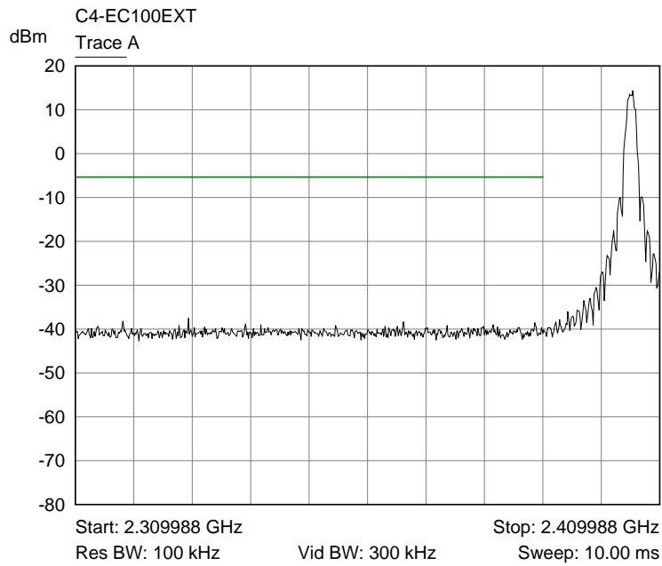
Trace A Lower channel band edge plot
