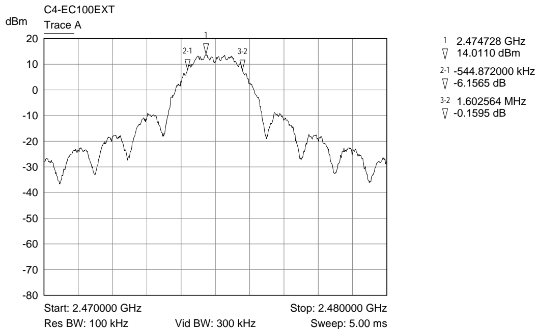
Trace A Upper channel band width plot
