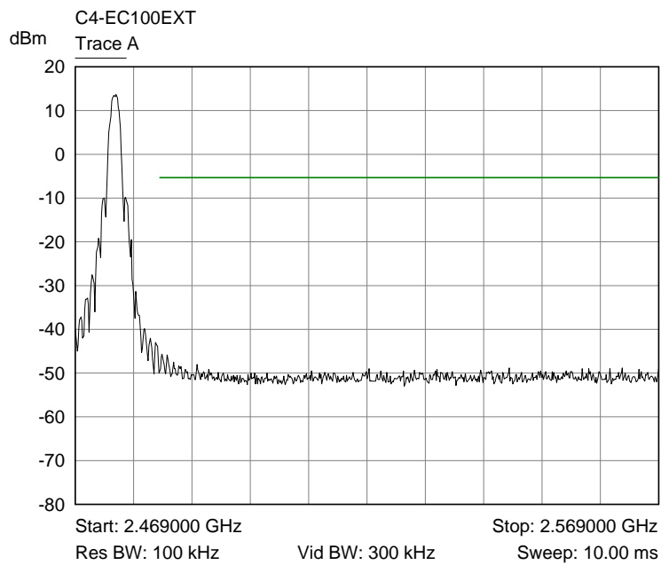
Trace A Upper channel band edge plot
