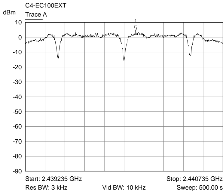
Trace A Middle channel 3 kHz power spectral density plot
