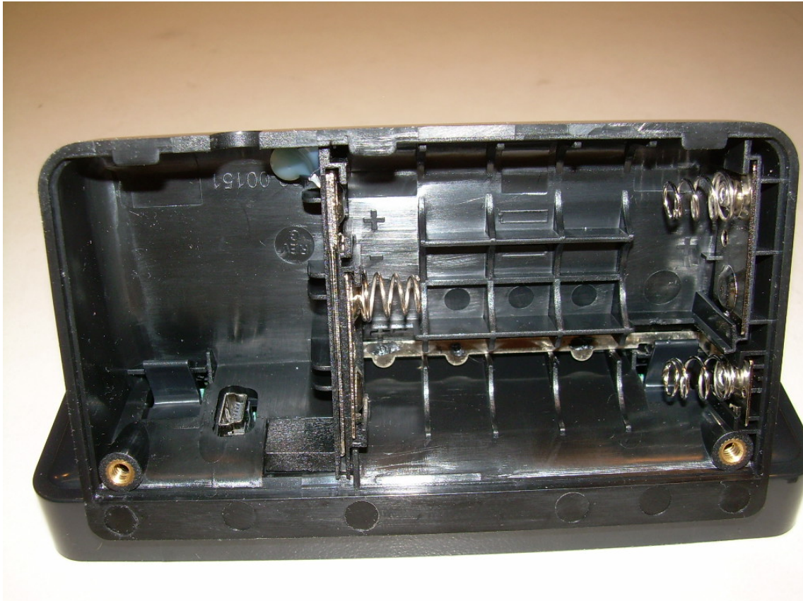
Photograph 7 – View of the EUT with the Bottom/Battery Cover Removed
