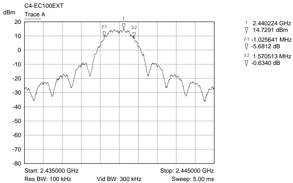
Trace A Middle channel band width plot
