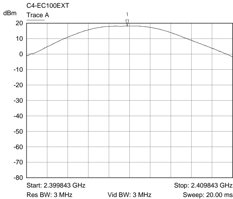
Trace A lower channel output power plot
