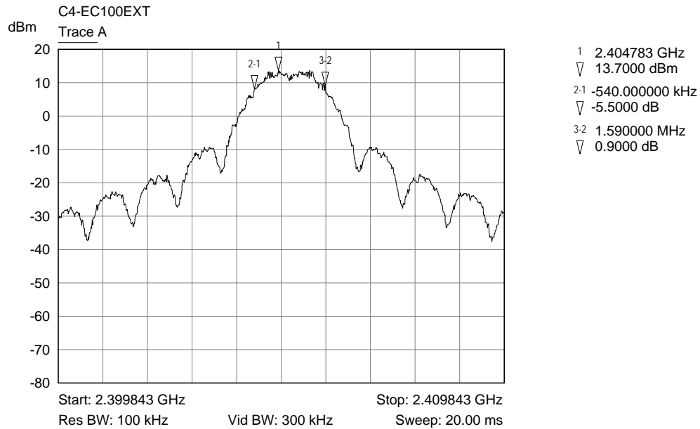
Trace A lower channel bandwidth plot
