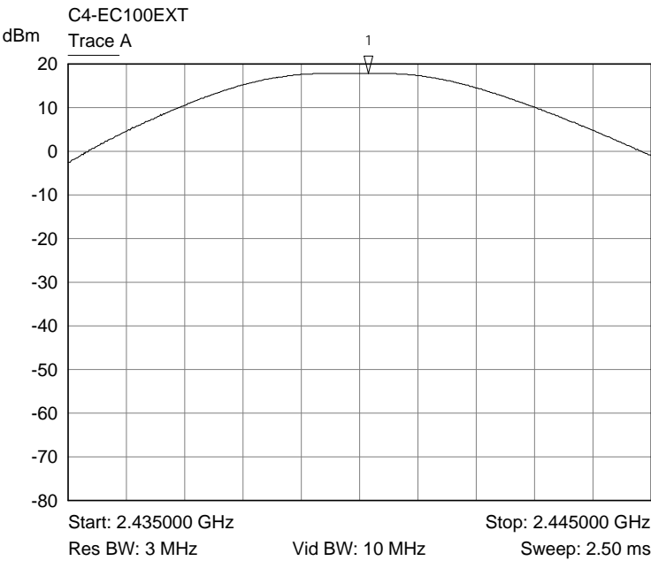
Trace A Middle channel output power plot
