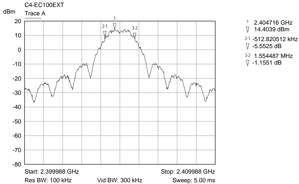
Trace A Lower channel band width plot
