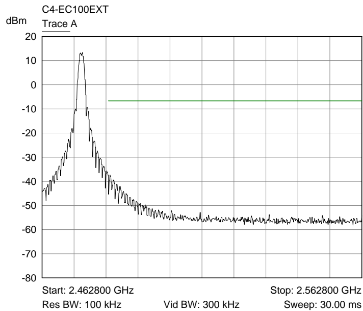
Trace A upper channel band edge plot
