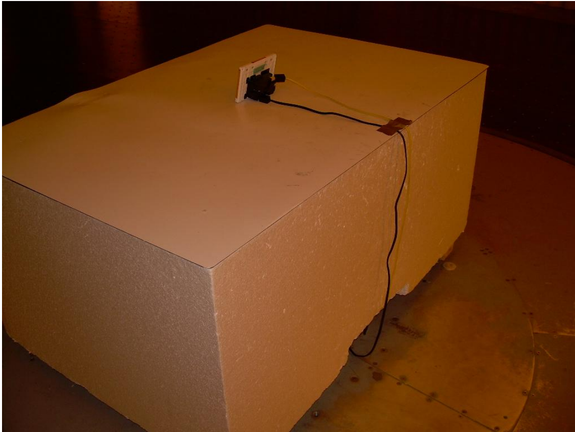
Back View Radiated Disturbance/ AC Powered Configuration
