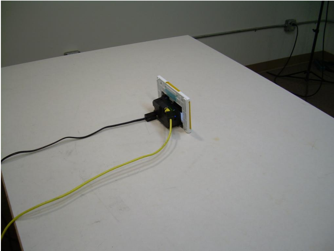
Back View Conducted Disturbance/AC Powered Configuration
