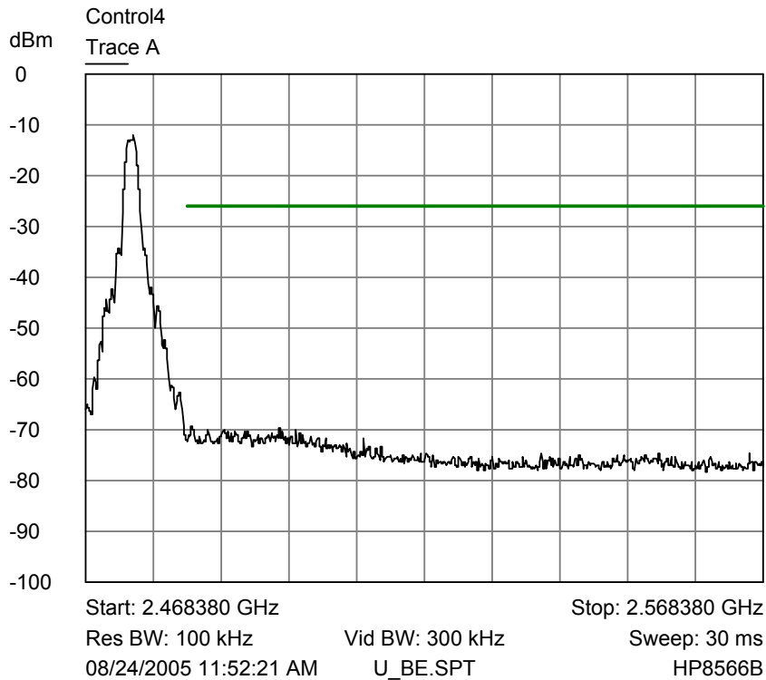
Upper Band Edge - Antenna Port Conducted Plot
