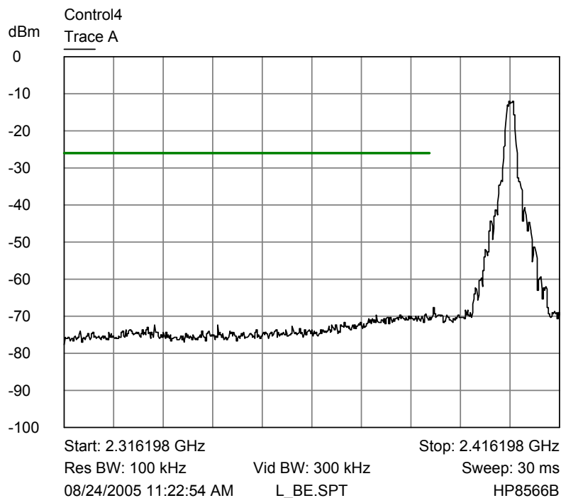
Lower Channel - Lower Band Edge - Antenna Port Conducted Plot
