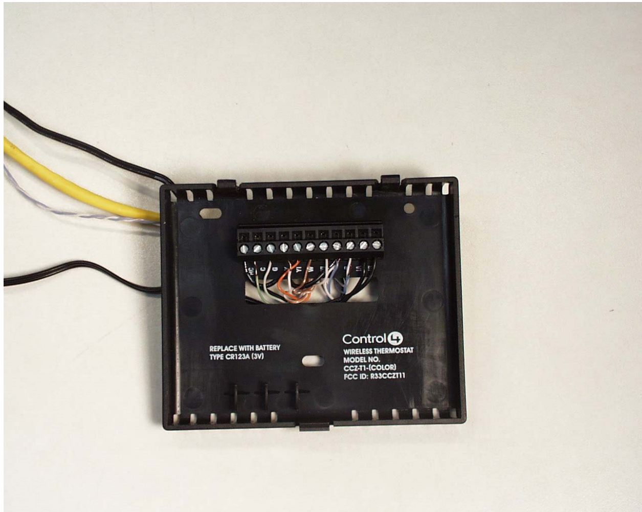
Photograph 5 - View of the Mounting Plate and Screw Terminals
