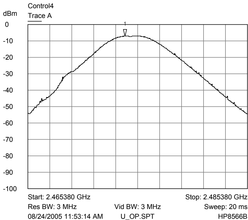
Upper Channel - Output Power Plot
