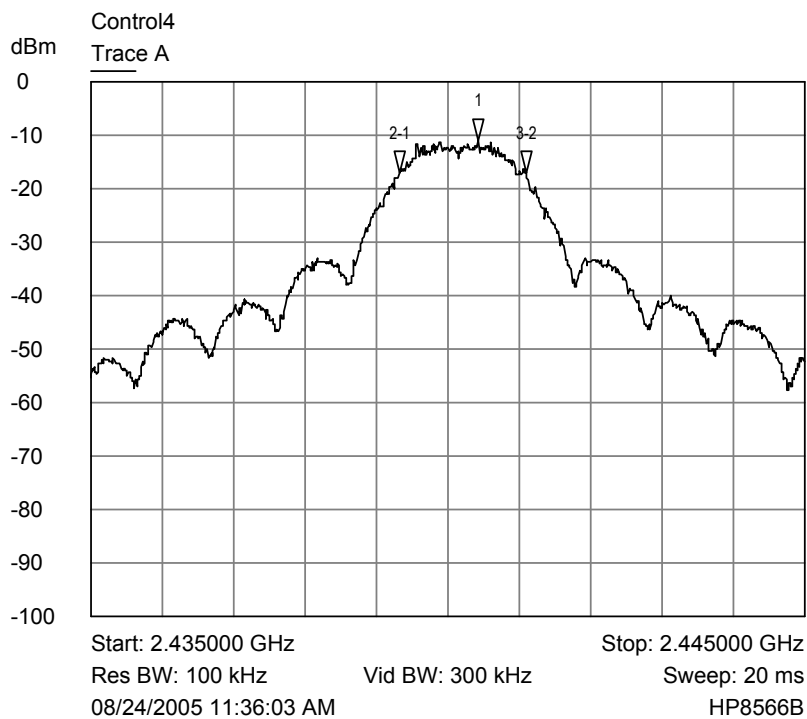
Middle Channel - Bandwidth Plot
