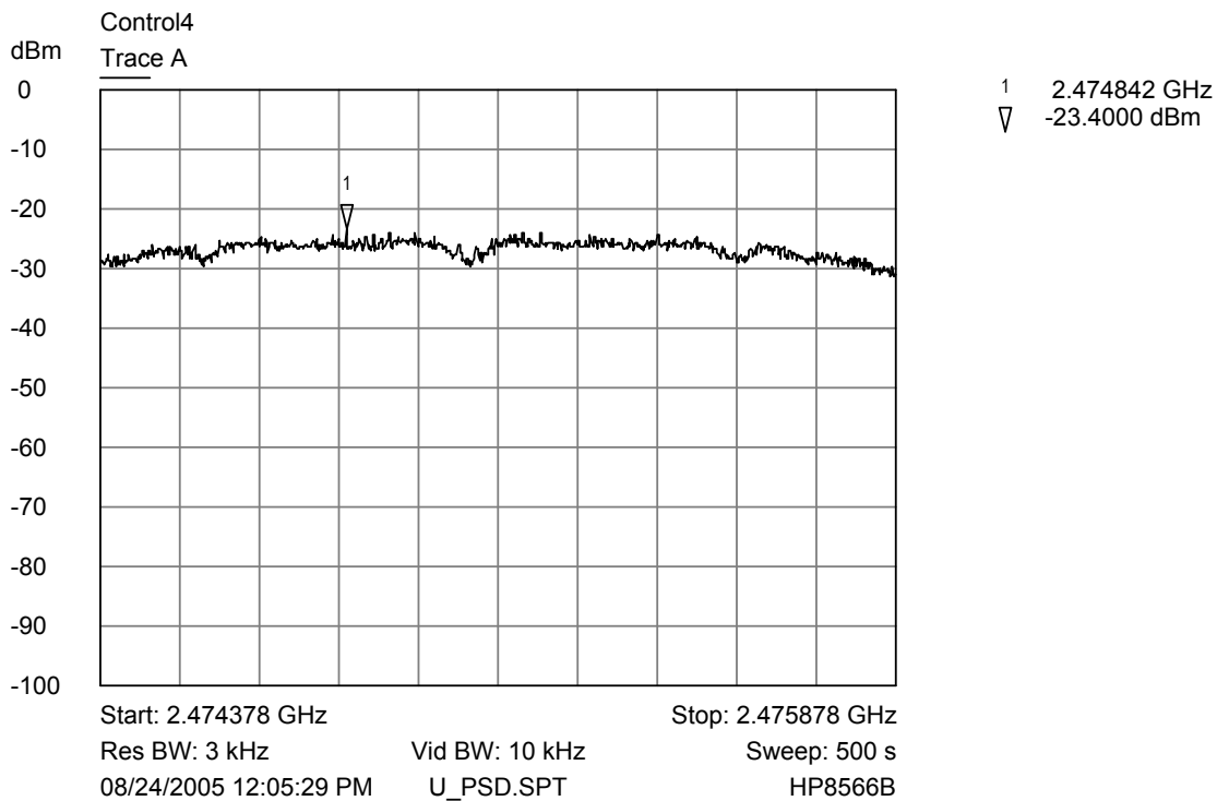
Upper Channel - Power Spectral Density Plot
