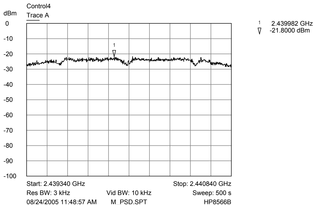
Middle Channel - 3kHz Power Spectral Density Plot
