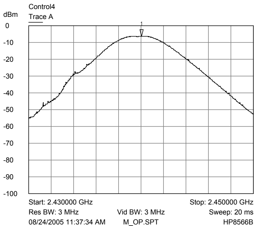
Middle Channel - Output Power Plot
