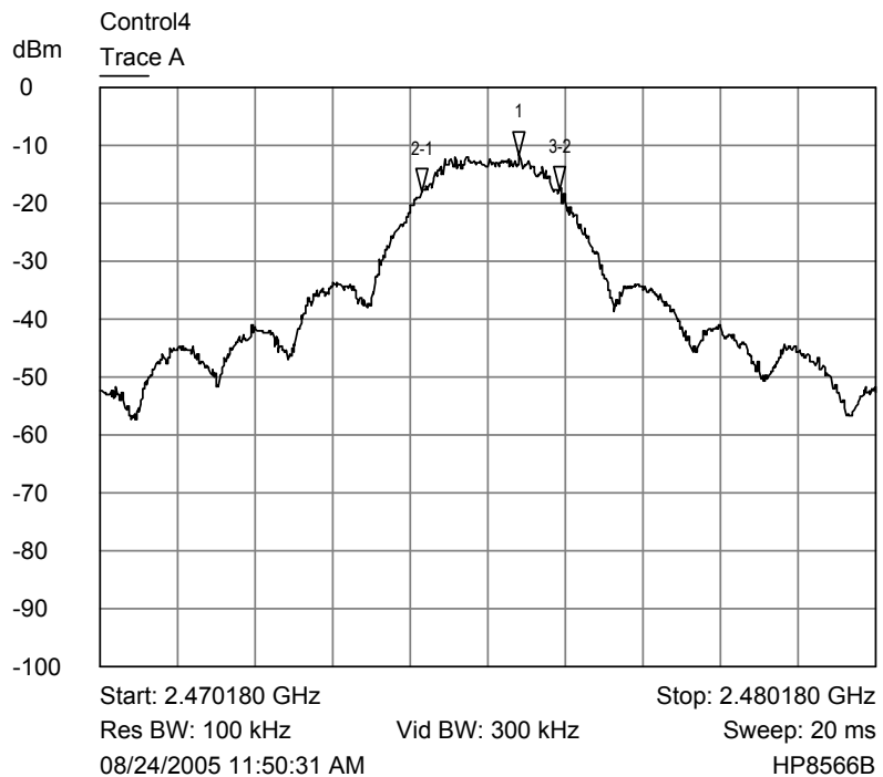
Upper Channel - Bandwidth Plot
