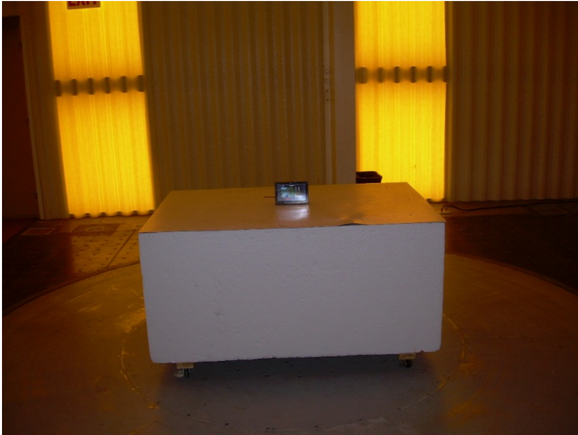
Front View Radiated Spurious Emissions – POE Configuration
