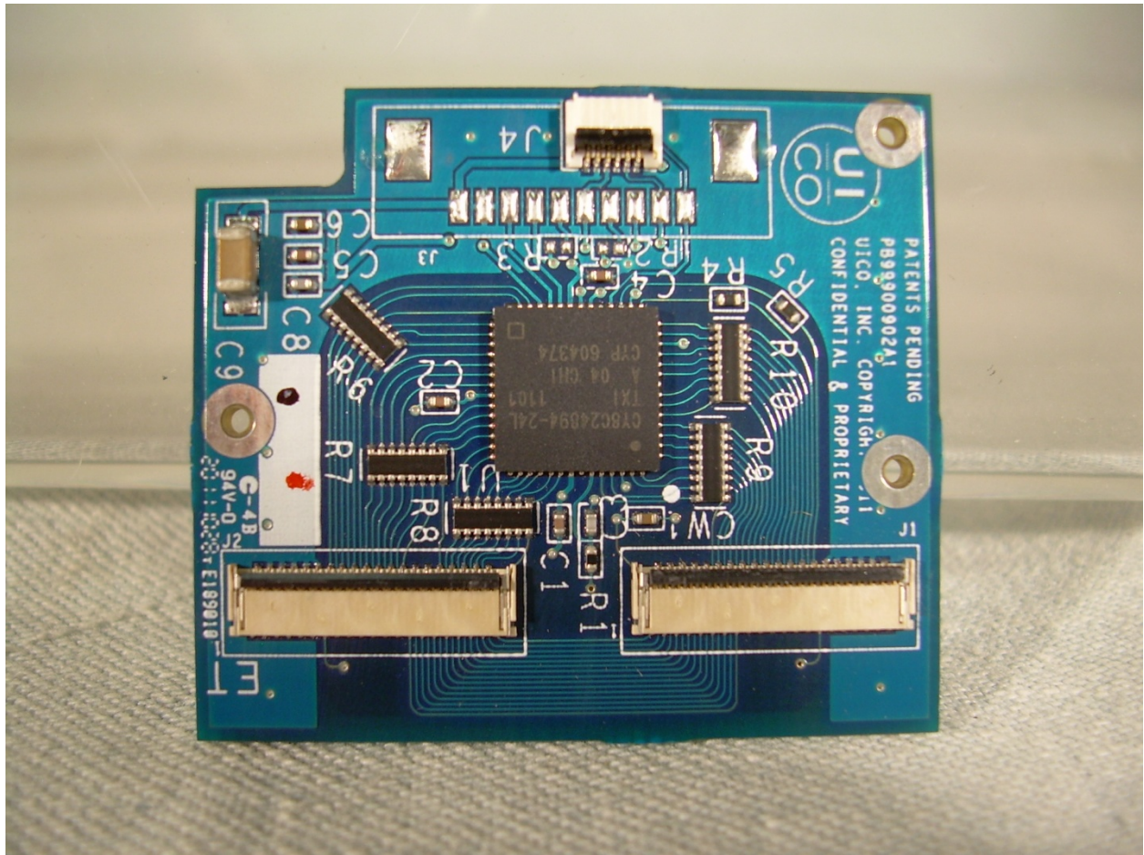
View of the Component Side of the Touch Interface PCB
