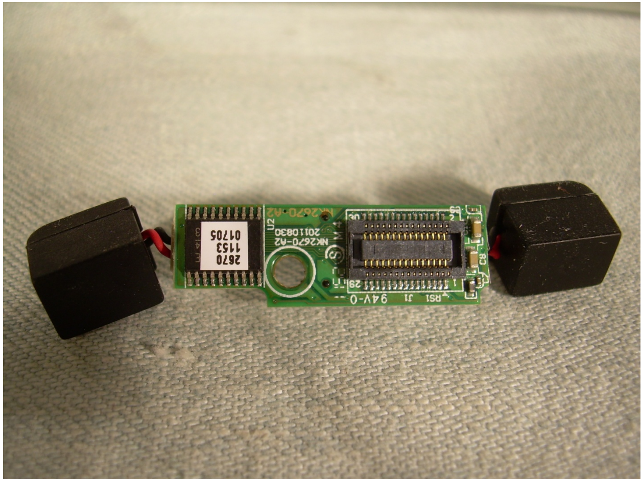
View of the Back Side of the Camera/Microphone PCB
