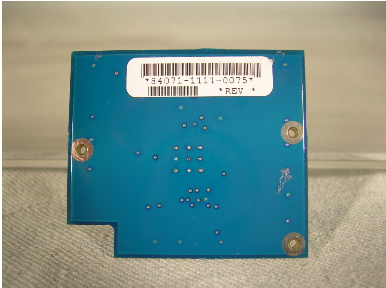
View of the Trace Side of the Touch Interface PCB
