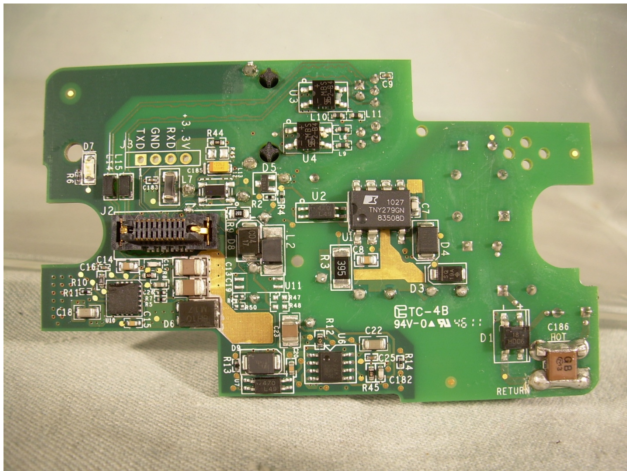
View of Component Side of Back Box PCB with Heatsink Removed
