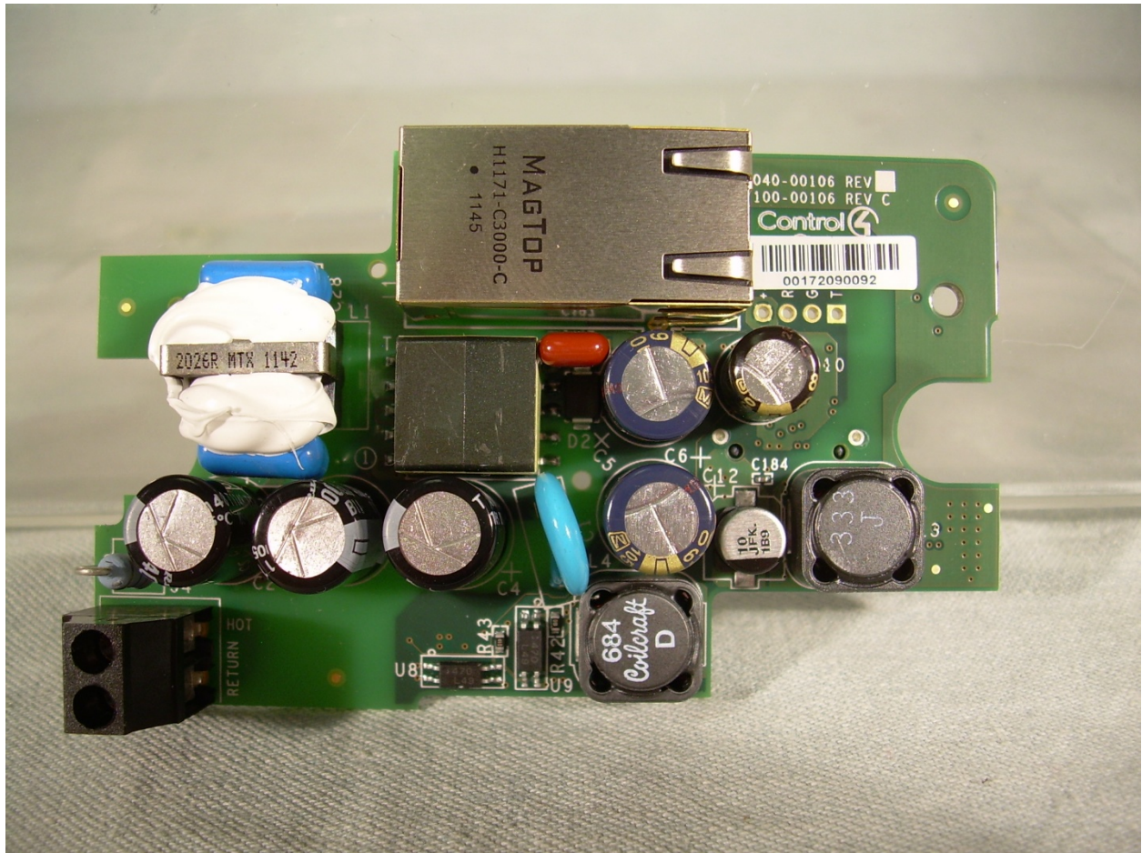
View of Trace Side of Back Box PCB with Heatsink Removed
