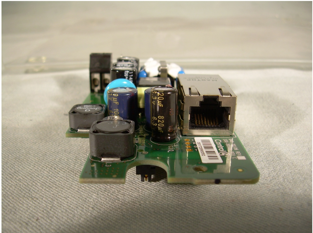
View of Side of Back Box PCB
