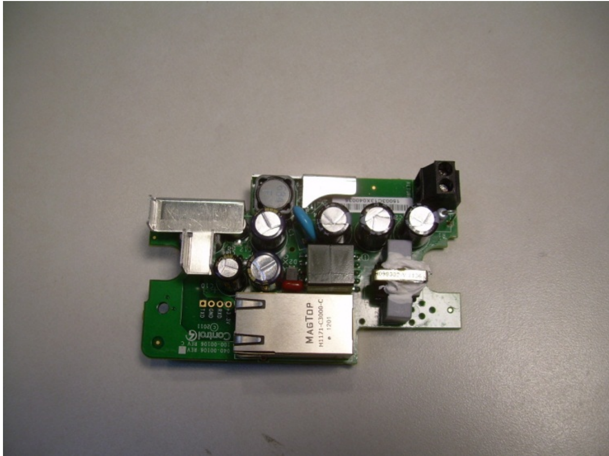
View of Component Side of Back Box PCB
