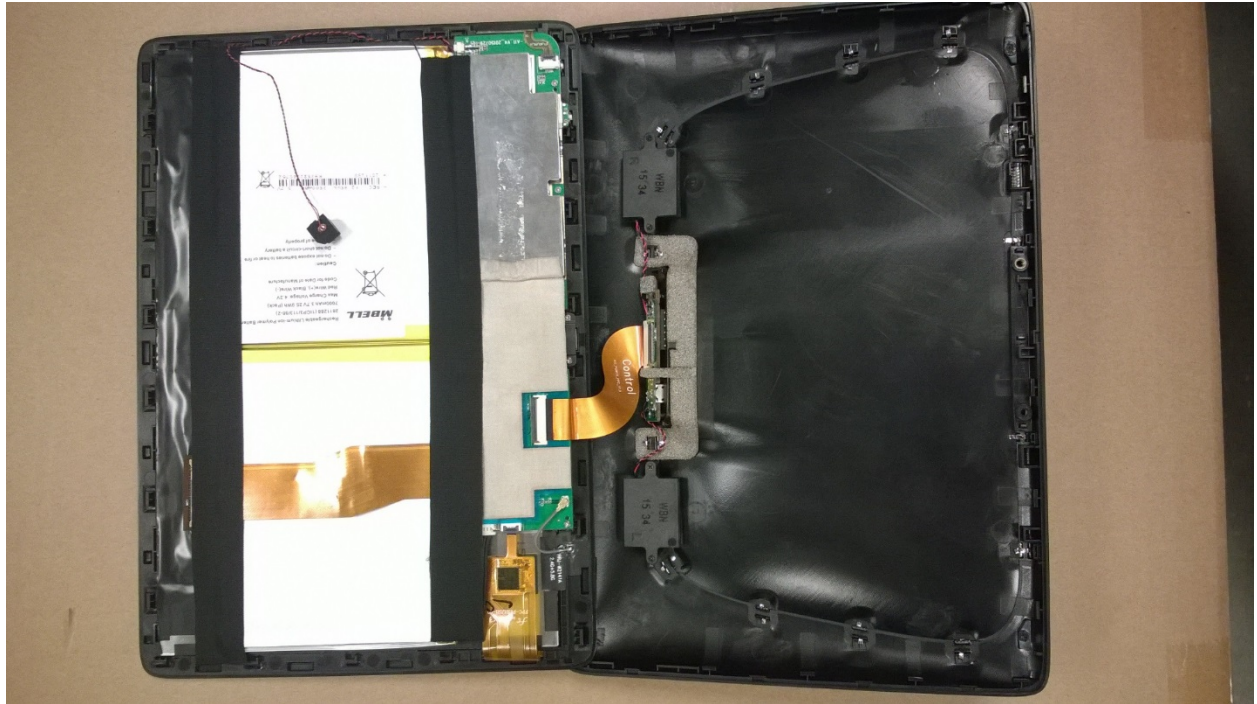
View of the Touchscreen with Housing Open
