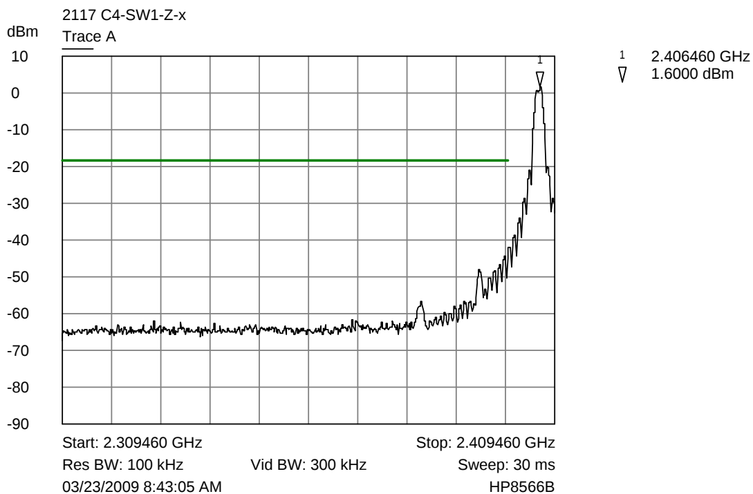
Trace A Lower channel band edge
