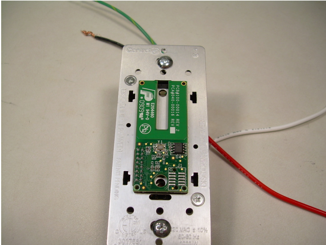
Photograph 7 - View of the EUT with the Plastic Cover Removed
