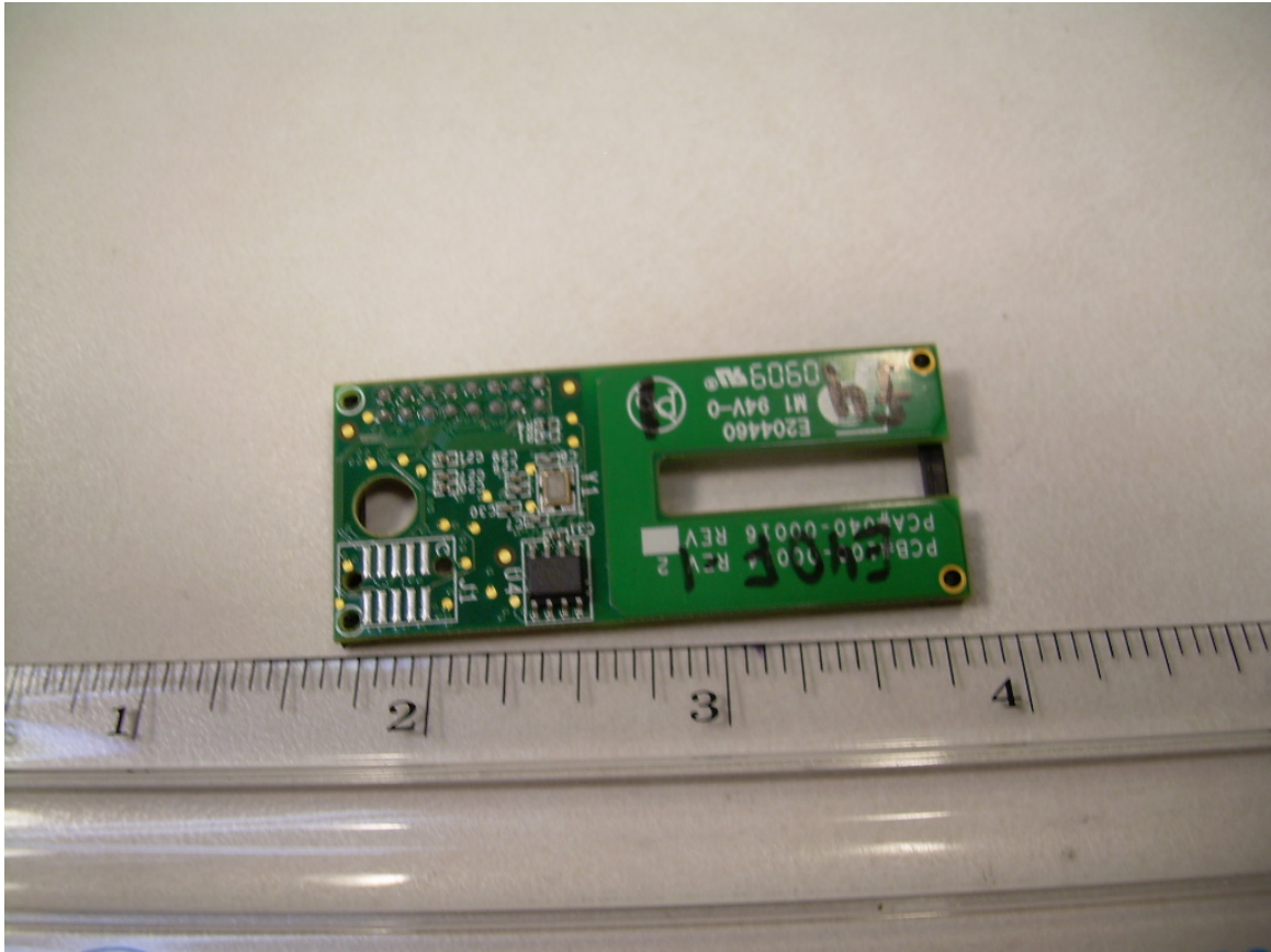
Photograph 8 - Front View of the Transceiver PCB
