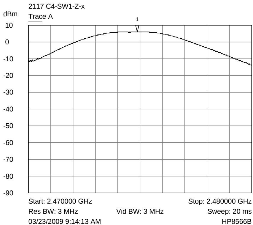
Trace A Upper channel output power
