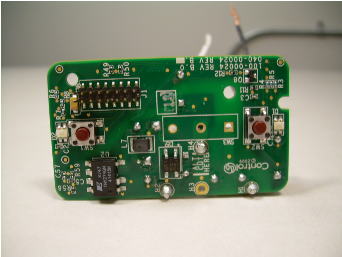
Photograph 11 - View of the Front of the Main PCB
