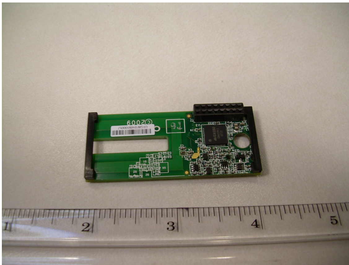
Photograph 9 - Back View of the Transceiver PCB
