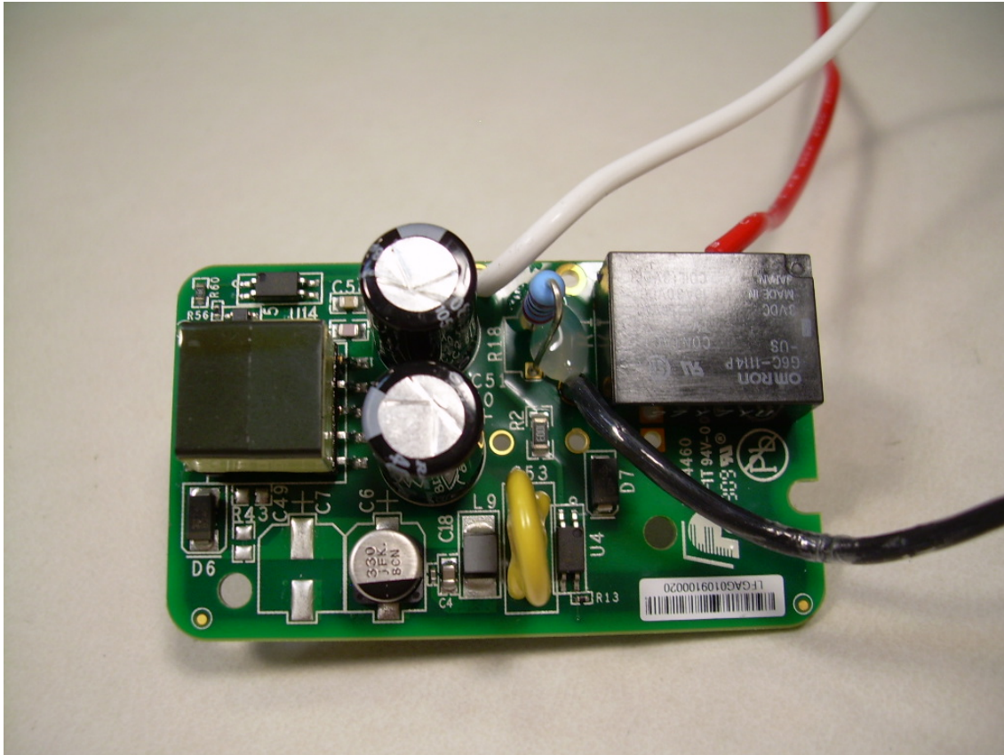
Photograph 10 - View of the Back of the Main PCB
