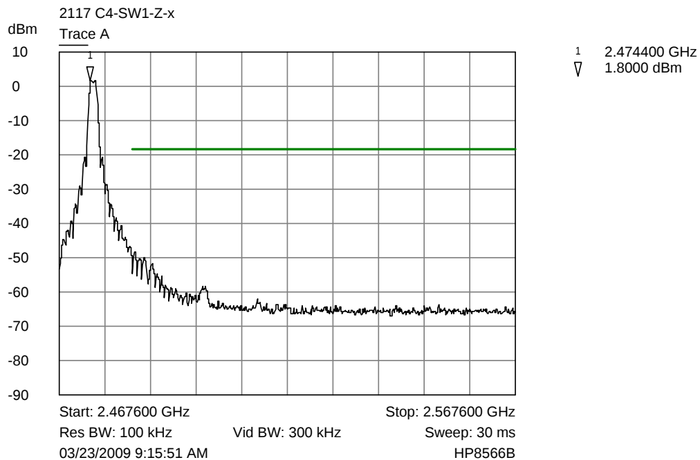
Trace A Upper channel band edge
