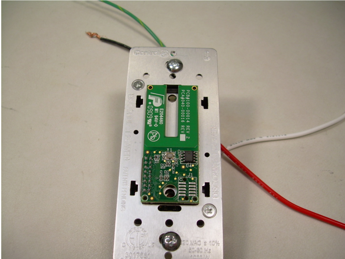
View of the EUT with the Plastic Cover Removed
