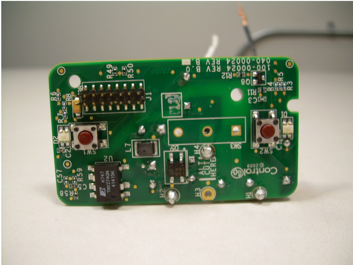
View of the Front of the Main PCB
