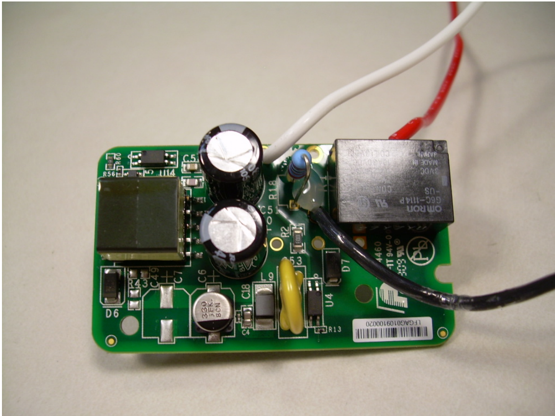
View of the Back of the Main PCB
