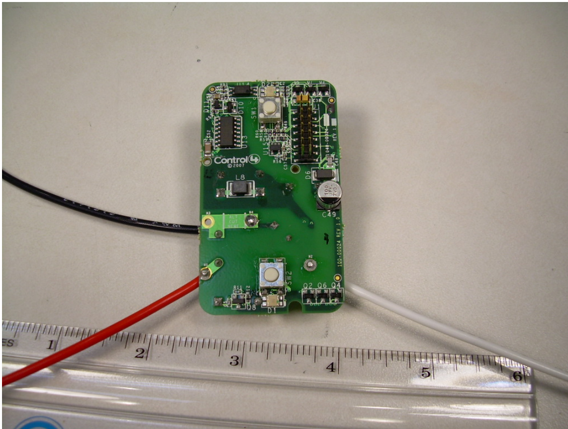
Front View of the C4-SW101-Z-x PCB
