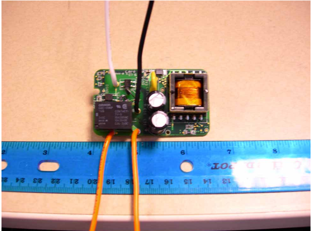
Back Side of the C4-FS101-Z-x PCB
