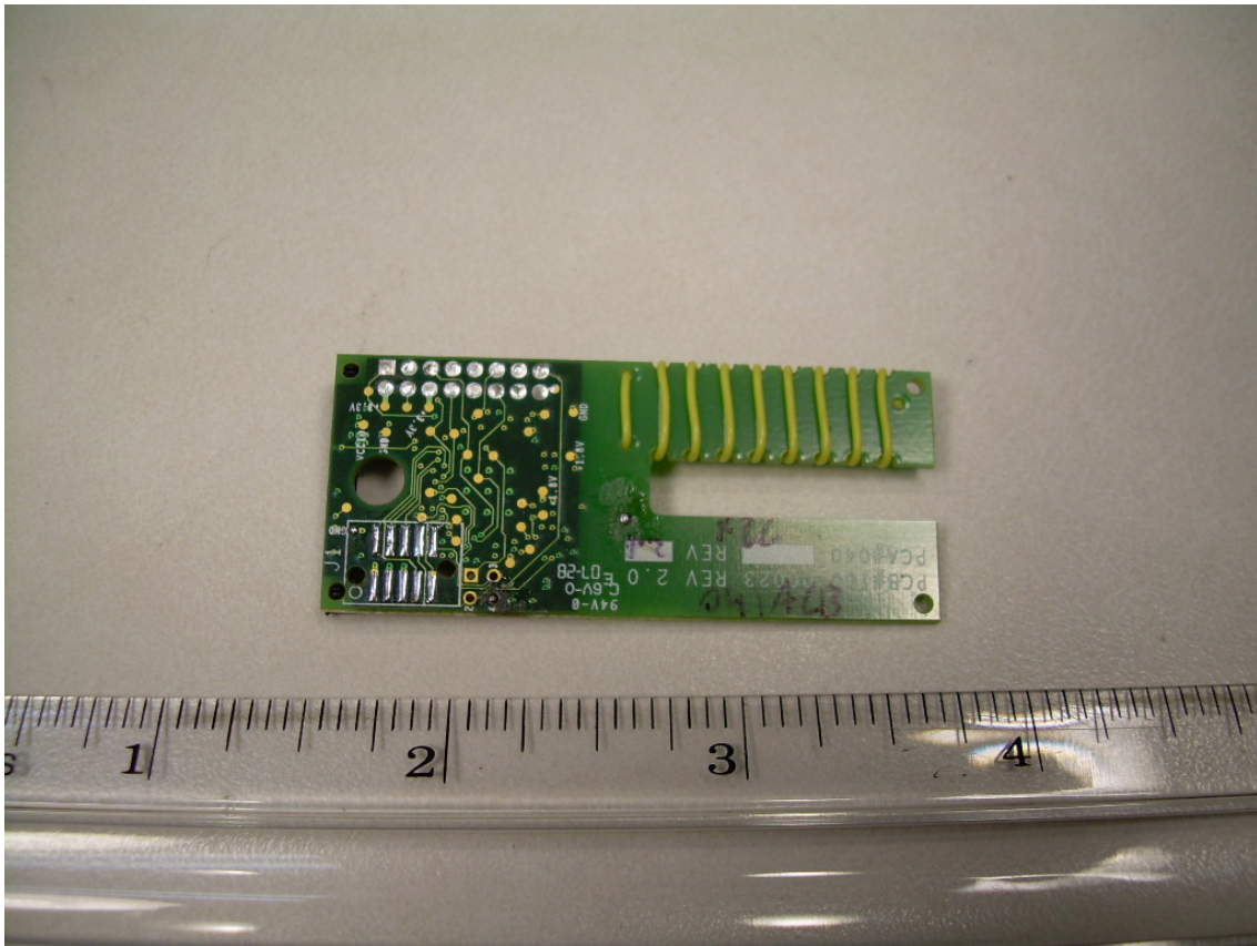
Front View of the Transceiver PCB
