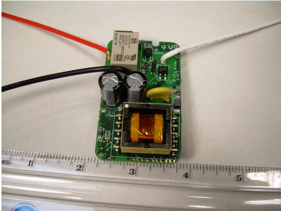
Back Side of the C4-SW101-Z-x PCB
