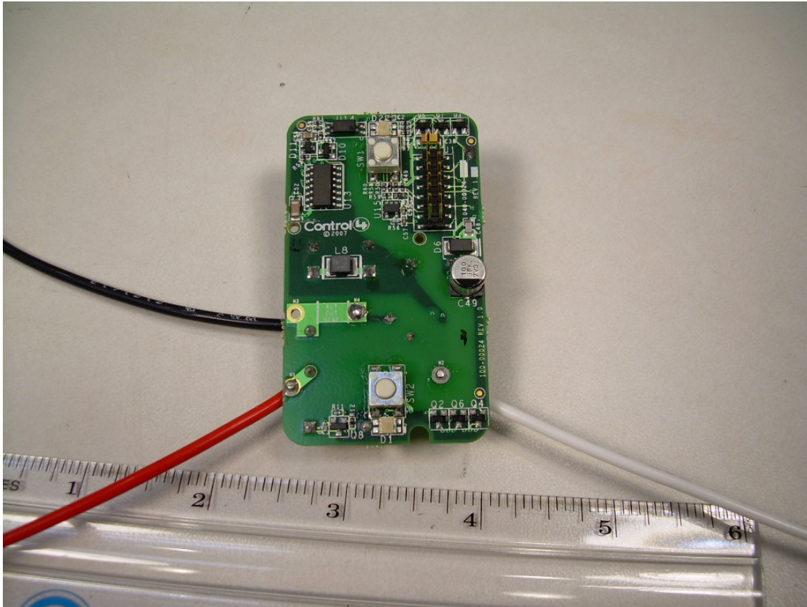
Photograph 7 - Front View of the C4-SW101-Z-x PCB
