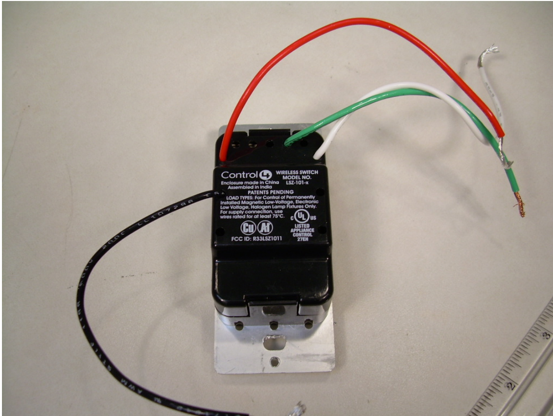
Photograph 6 - Back View of the C4-SW101-Z-x
