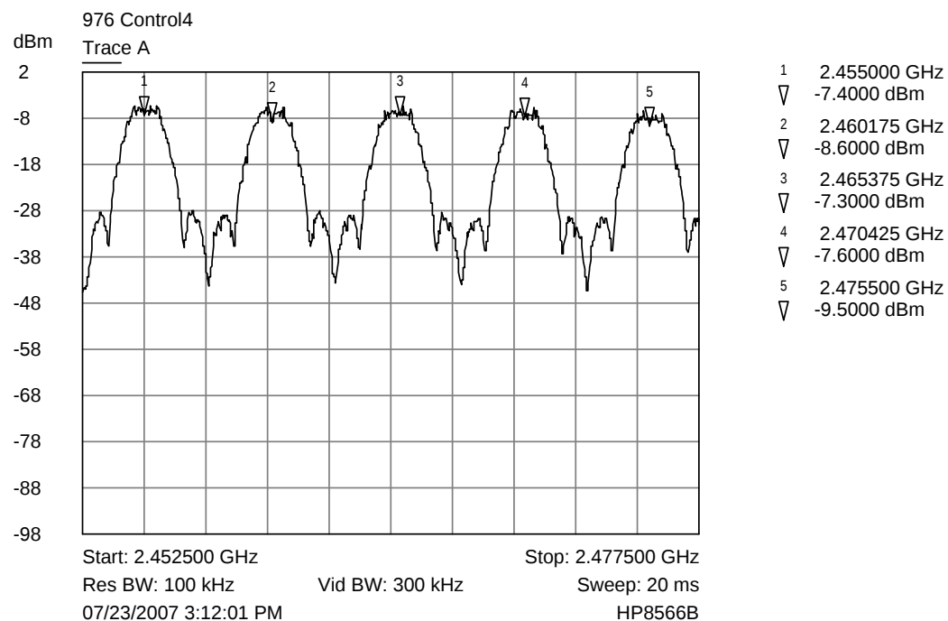
Trace A Upper 5 channel plot
