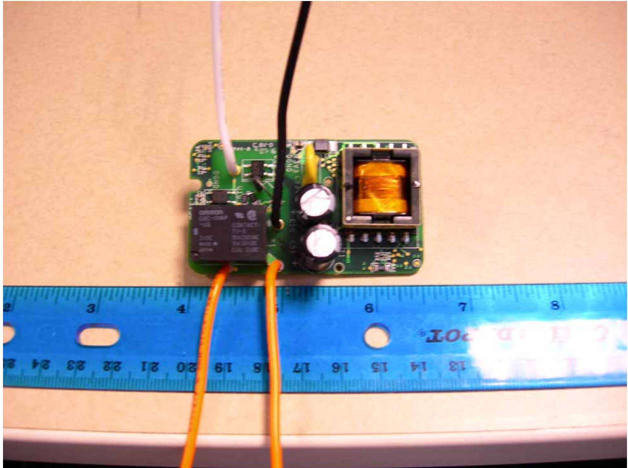
Photograph 9 - Back Side of the C4-FS101-Z-x PCB
