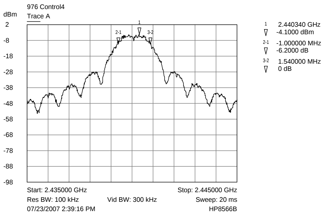
Trace A Middle channel bandwidth plot
