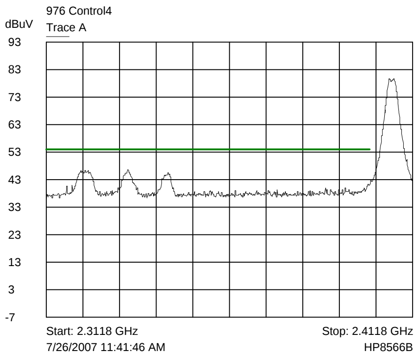
Trace A Lower band edge plot - corrected trace
