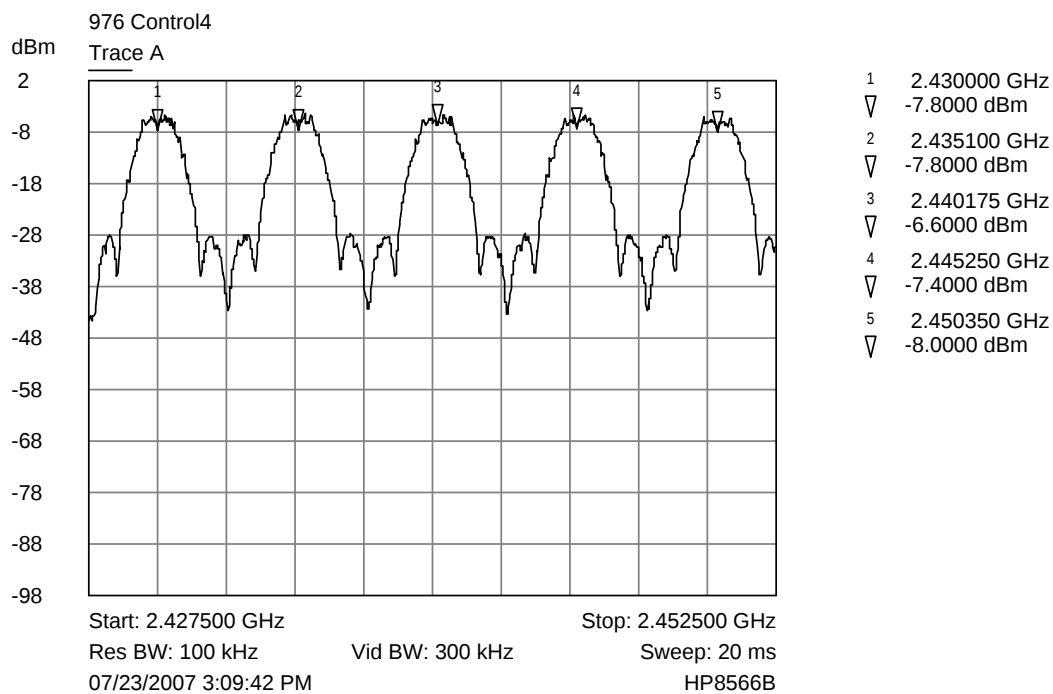
Trace A Middle 5 channel plot
