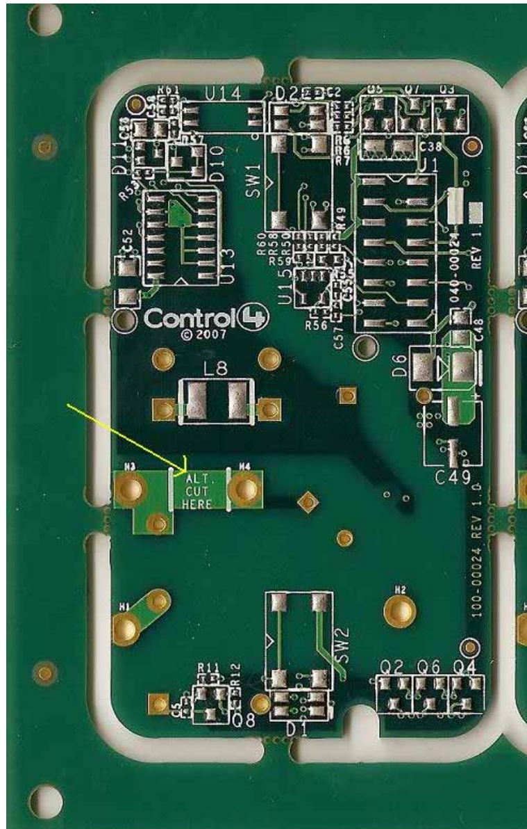
Photograph 10 - View of the Trace to be Removed on the C4-FS101-Z-x PCB
