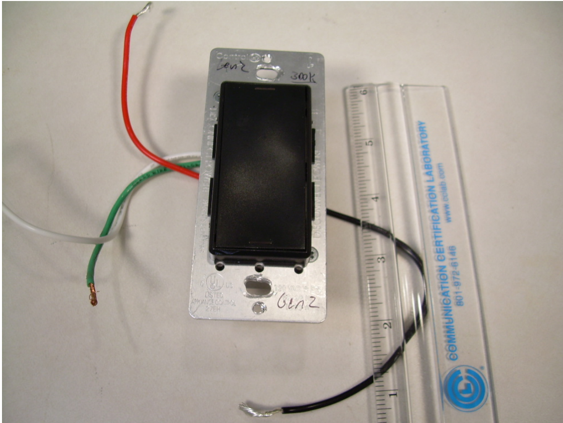
Photograph 5 - Front View of the C4-SW101-Z-x
