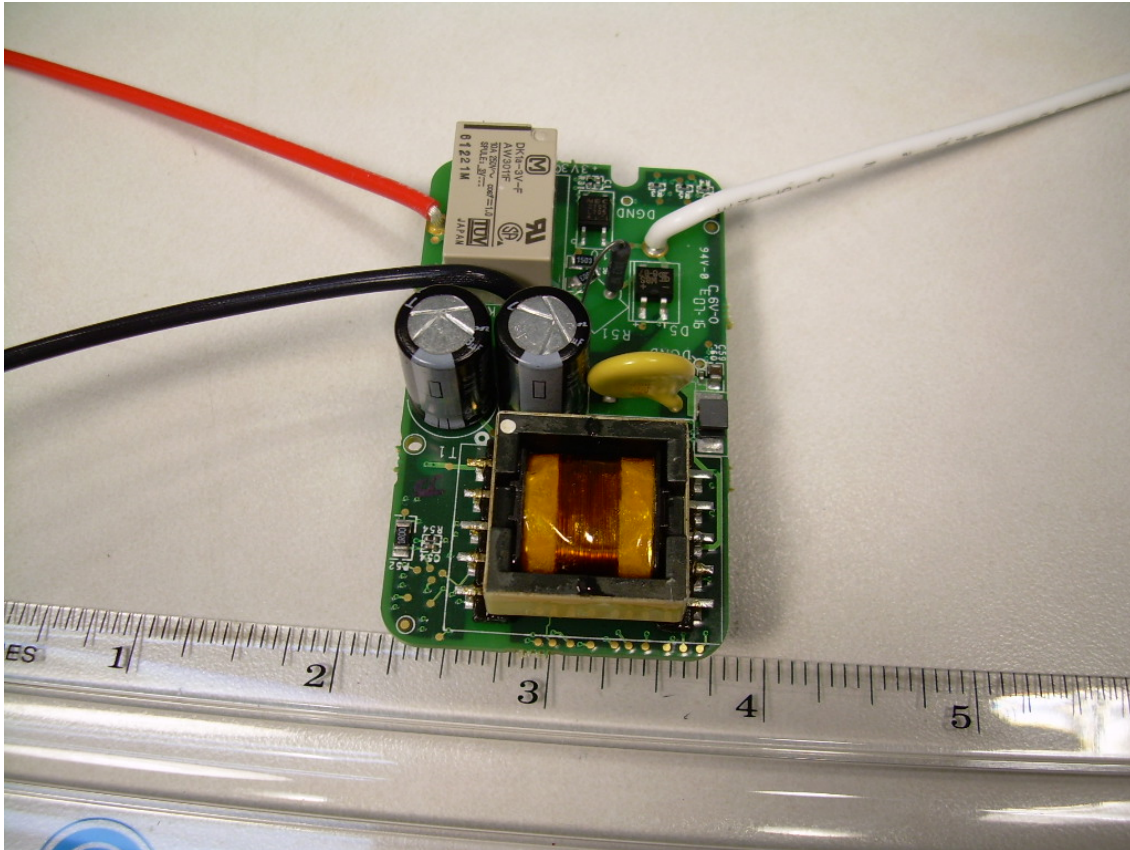
Photograph 8 - Back Side of the C4-SW101-Z-x PCB
