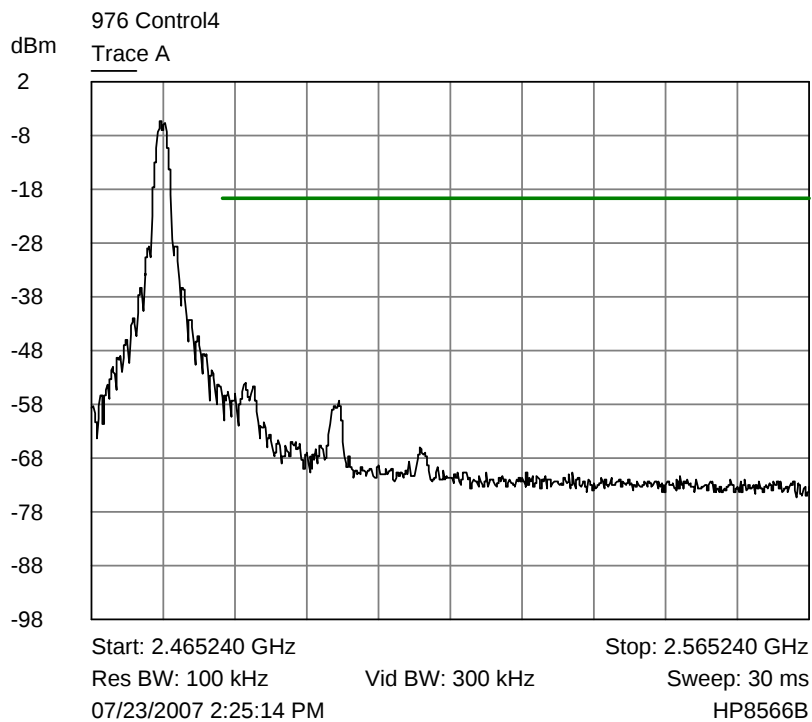
Trace A Upper channel conducted band edge plot
