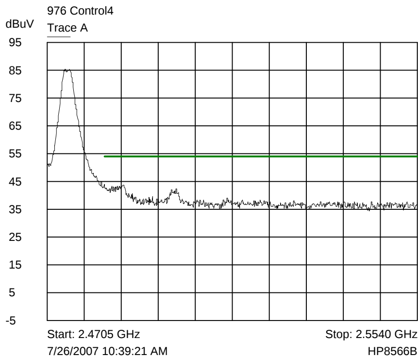
Trace A Upper band edge plot - corrected trace
