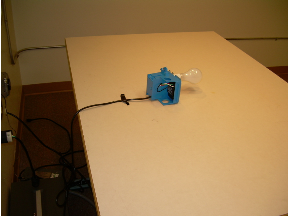
Back View Conducted Disturbance Worst Case Configuration
