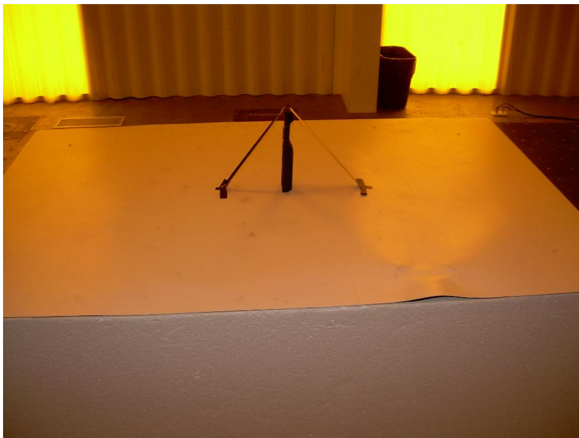
View of Radiated Emission Setup – Vertical EUT Placement
