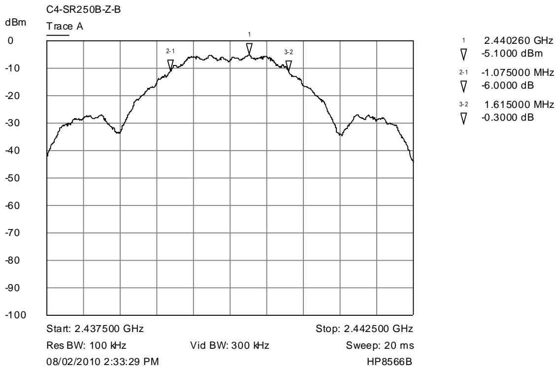
Trace A Middle channel bandwidth plot
