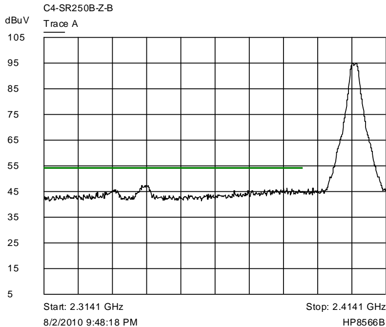
Trace A Lower band edge plot - corrected radiated trace peak detection vs average limit
