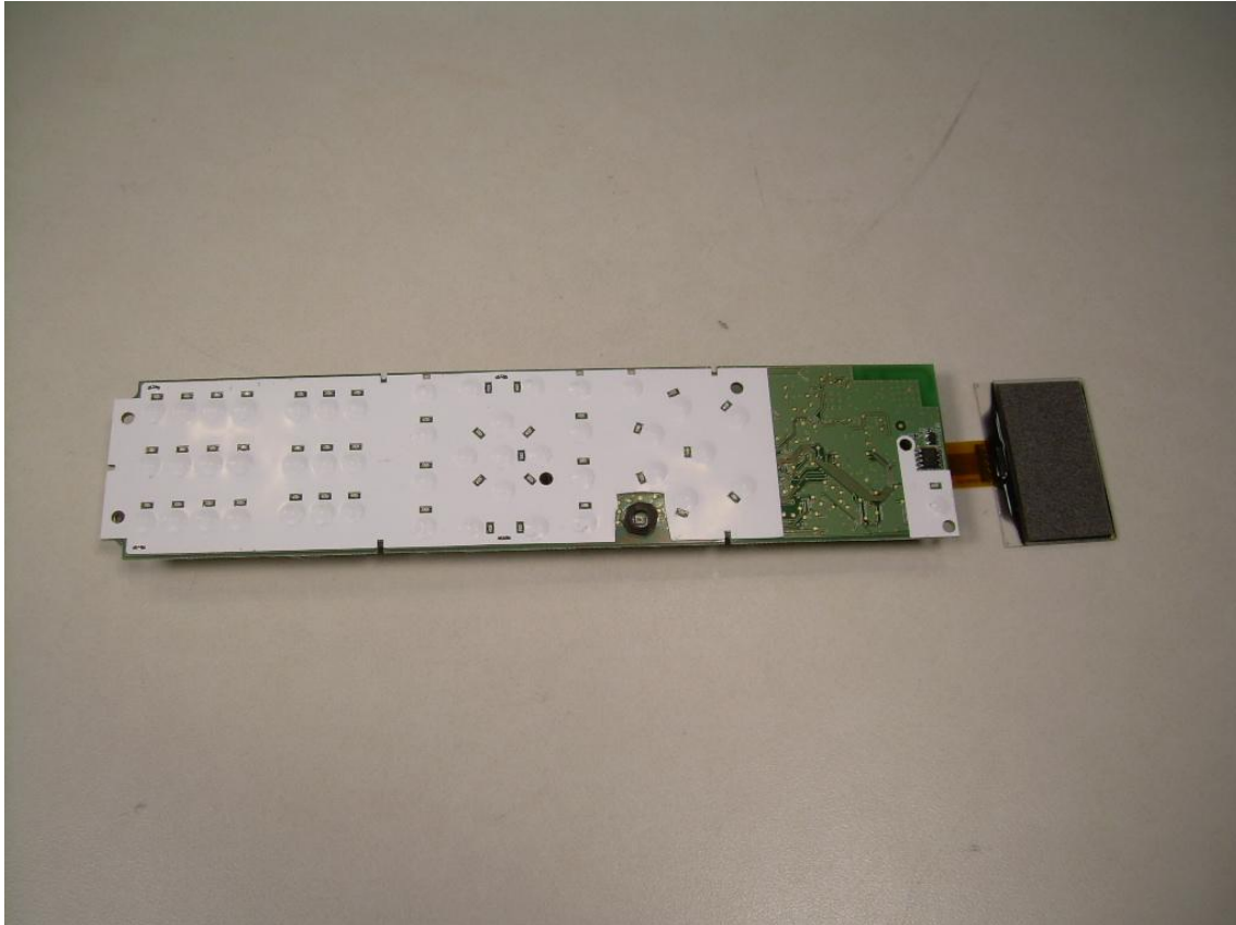
Photograph 7 – View of the Keypad Side of the EUT PCB with Display Lifted
