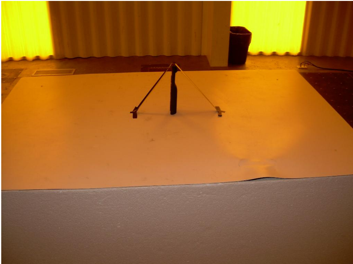
Photograph 1 – View of Radiated Emission Setup – Vertical EUT Placement
