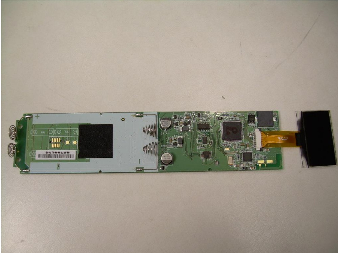
Photograph 8 – View of the Component Side of the EUT PCB
