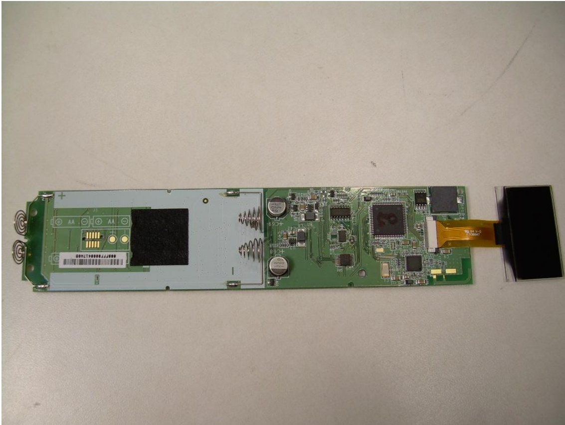
View of the Component Side of the EUT PCB
