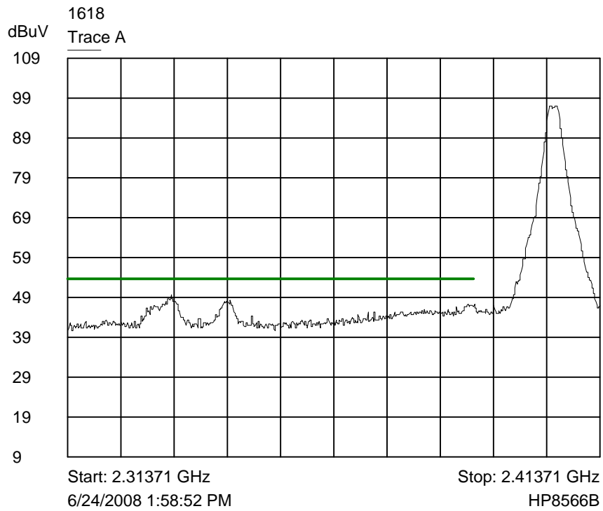
Trace A lower channel corrected peak detection band edge plot
