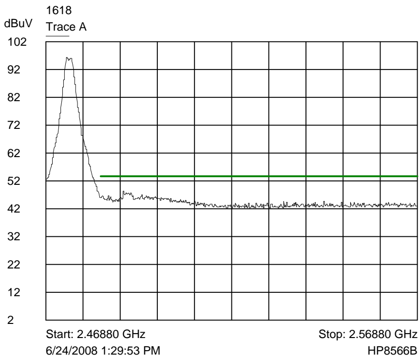
Trace A upper channel corrected peak detection band edge plot
