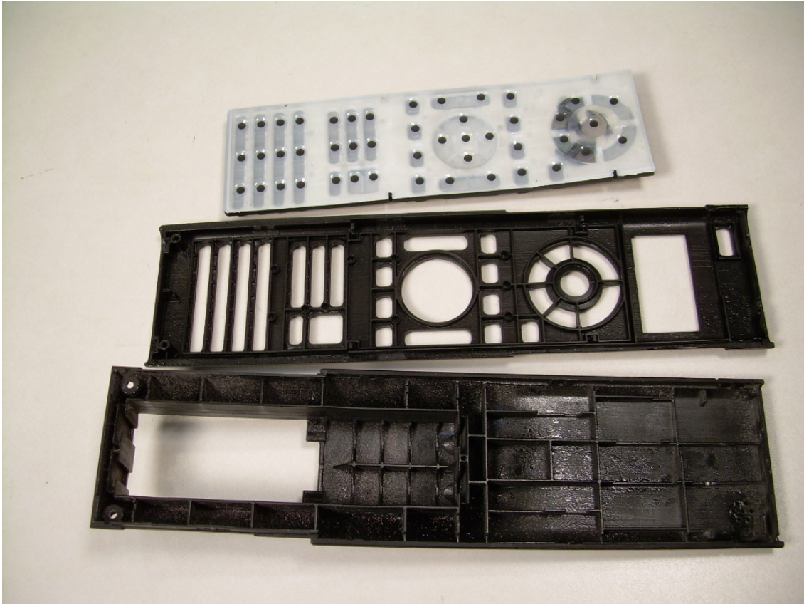
Photograph 7 - View of the Internal Side of the Housing
