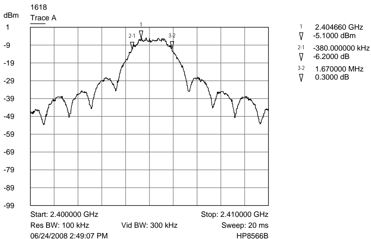
Trace A Lower channel band width plot
