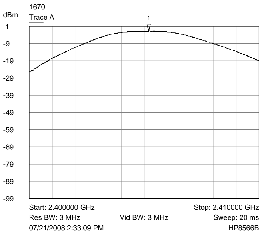
Trace A Lower channel output power plot
