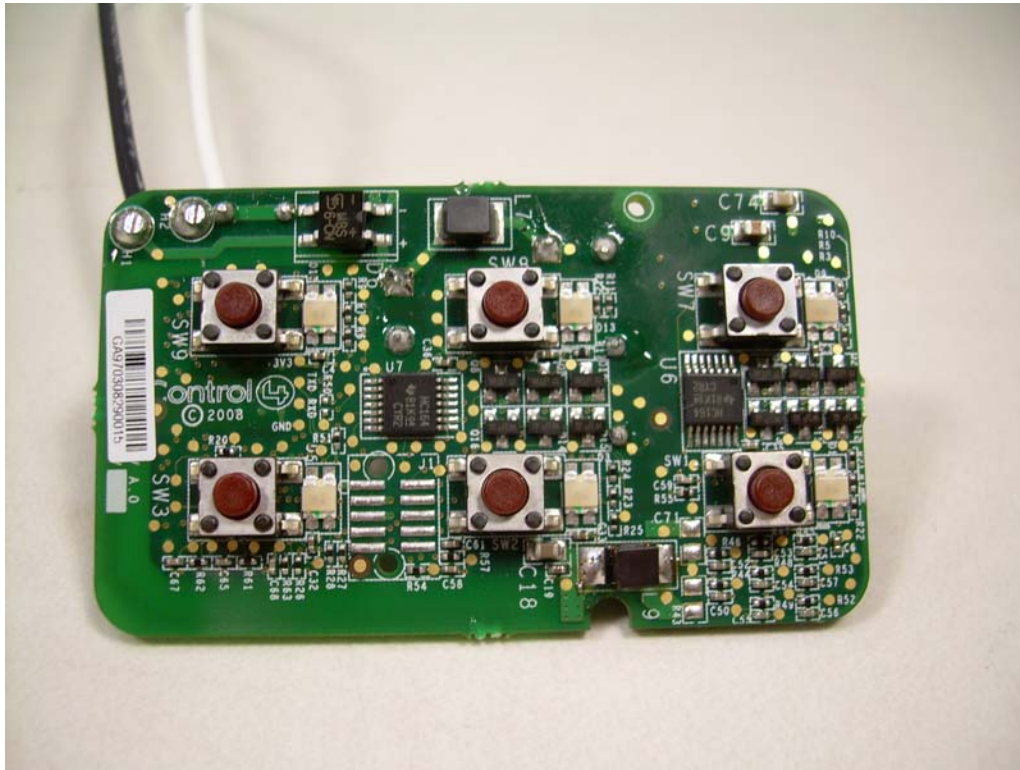
Photograph 7 - View of the Front of the EUT PCB
