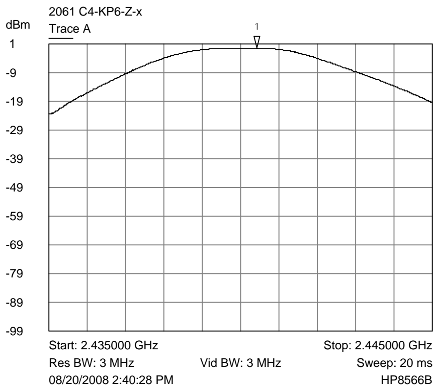
Trace A Middle channel output powre plot
