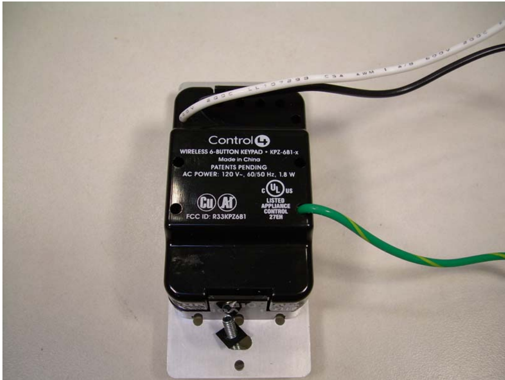
Photograph 6 - Back View of the EUT
