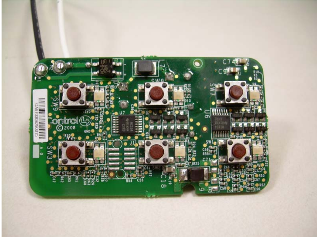
View of the Front of the EUT PCB
