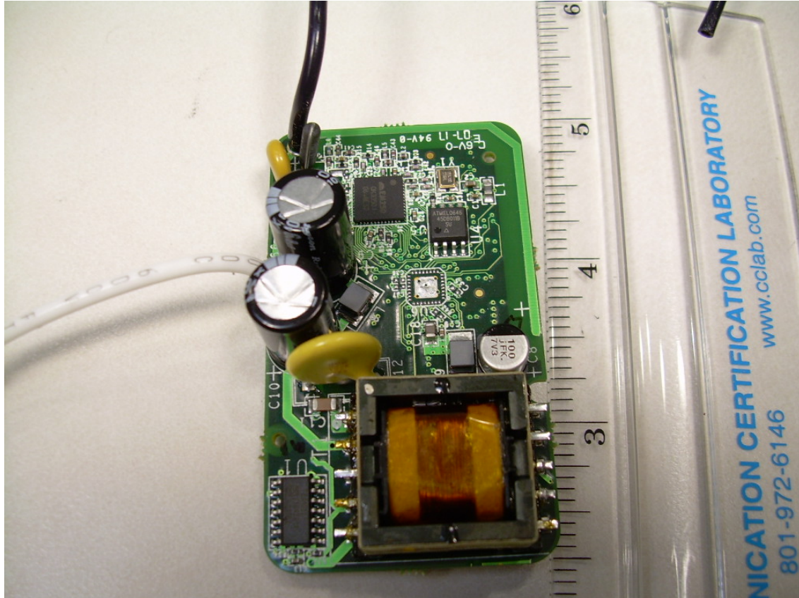
Back Side of the C4-KP3-Z-x PCB
