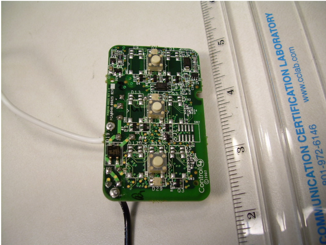
Front Side of the C4-KP3-Z-x PCB
