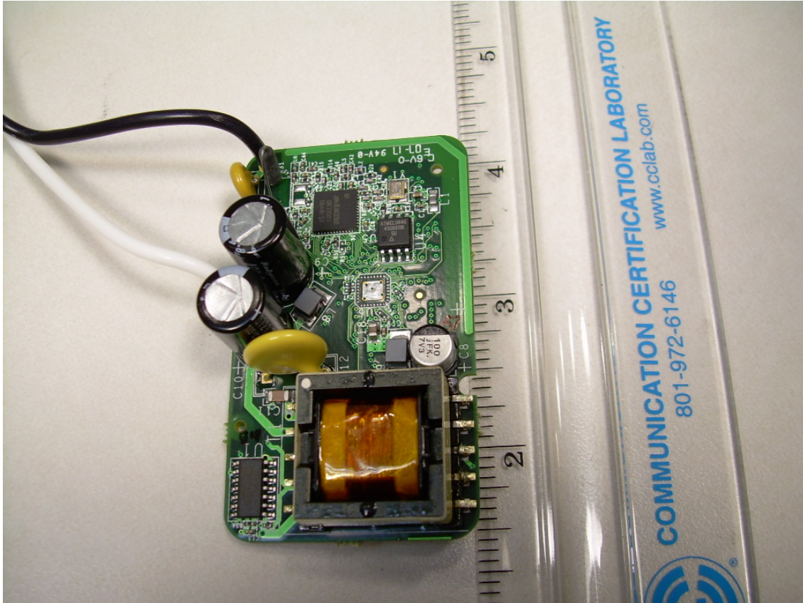
Back Side of the C4-KP2-Z-x PCB
