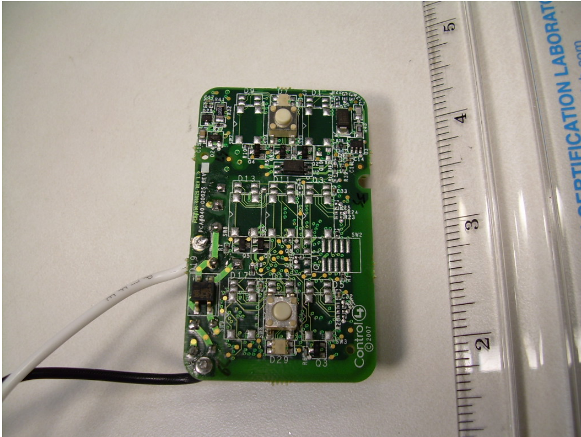
Photograph 11 - Front Side of the C4-KP2-Z-x PCB
