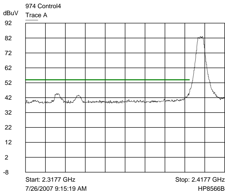
Trace A Lower band edge plot - radiated - corrected trace
