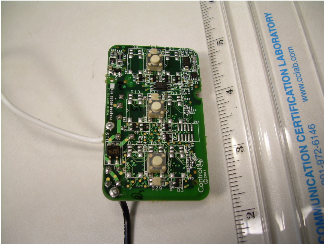
Photograph 9 - Front Side of the C4-KP3-Z-x PCB
