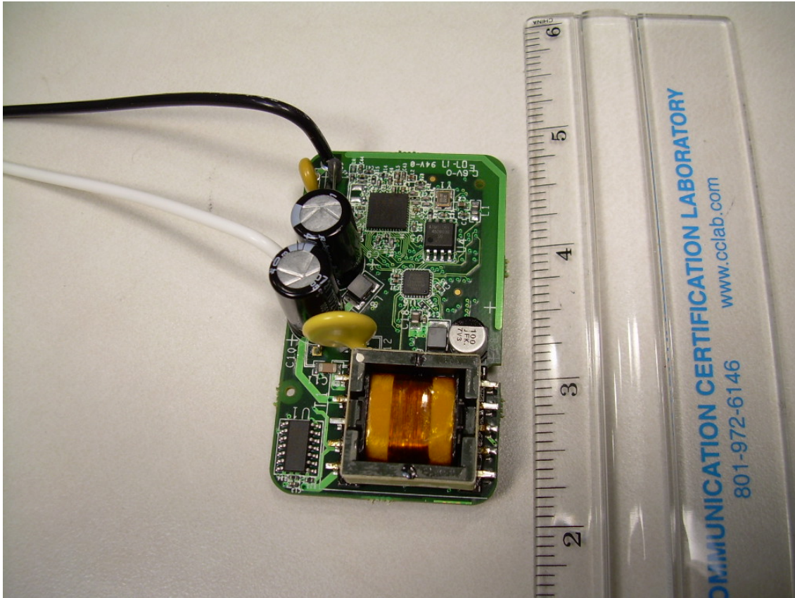
Photograph 8 - Back Side of the C4-KP6-Z-x PCB
