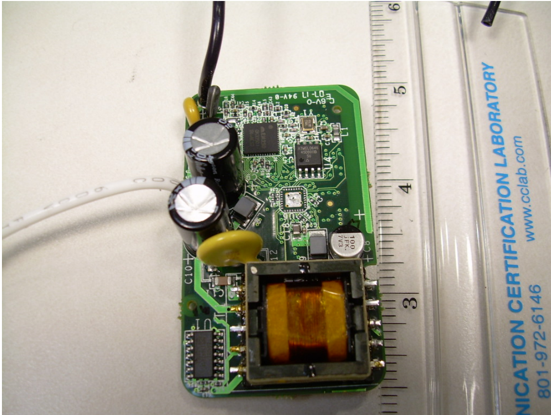
Photograph 10 - Back Side of the C4-KP3-Z-x PCB
