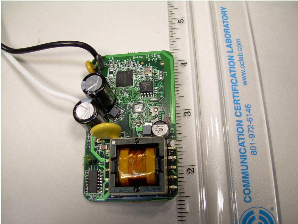
Photograph 12 - Back Side of the C4-KP2-Z-x PCB
