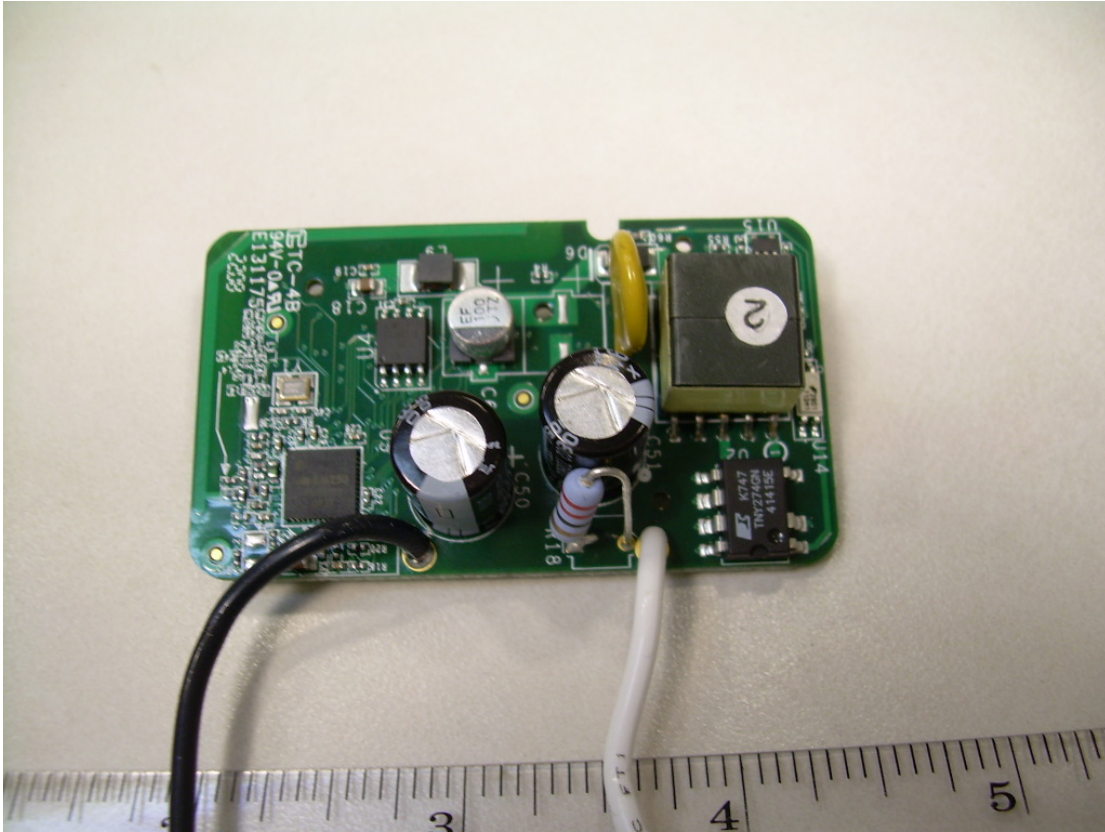
Photograph 8 - Back View of the C4-KP3-Z-x PCB
