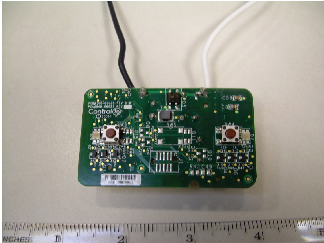
Photograph 11 - Front View of the C4-KP2-Z-x PCB
