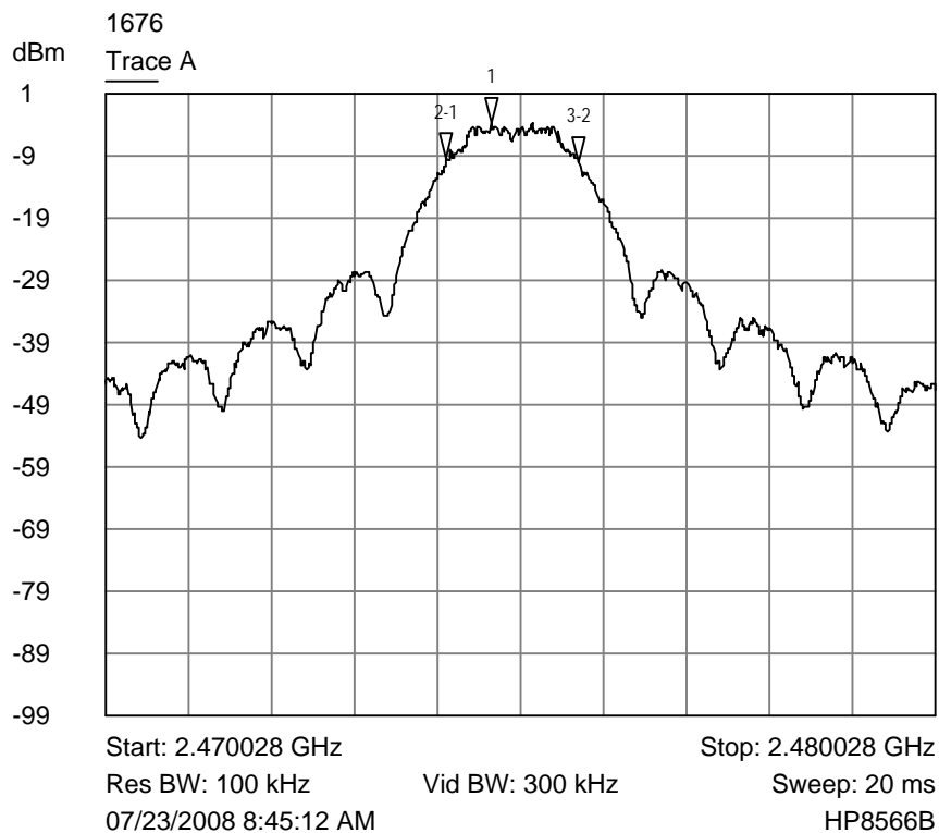
Trace A Upper channel band width plot
