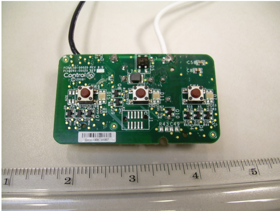
Photograph 7 - Front View of the C4-KP3-Z-x PCB
