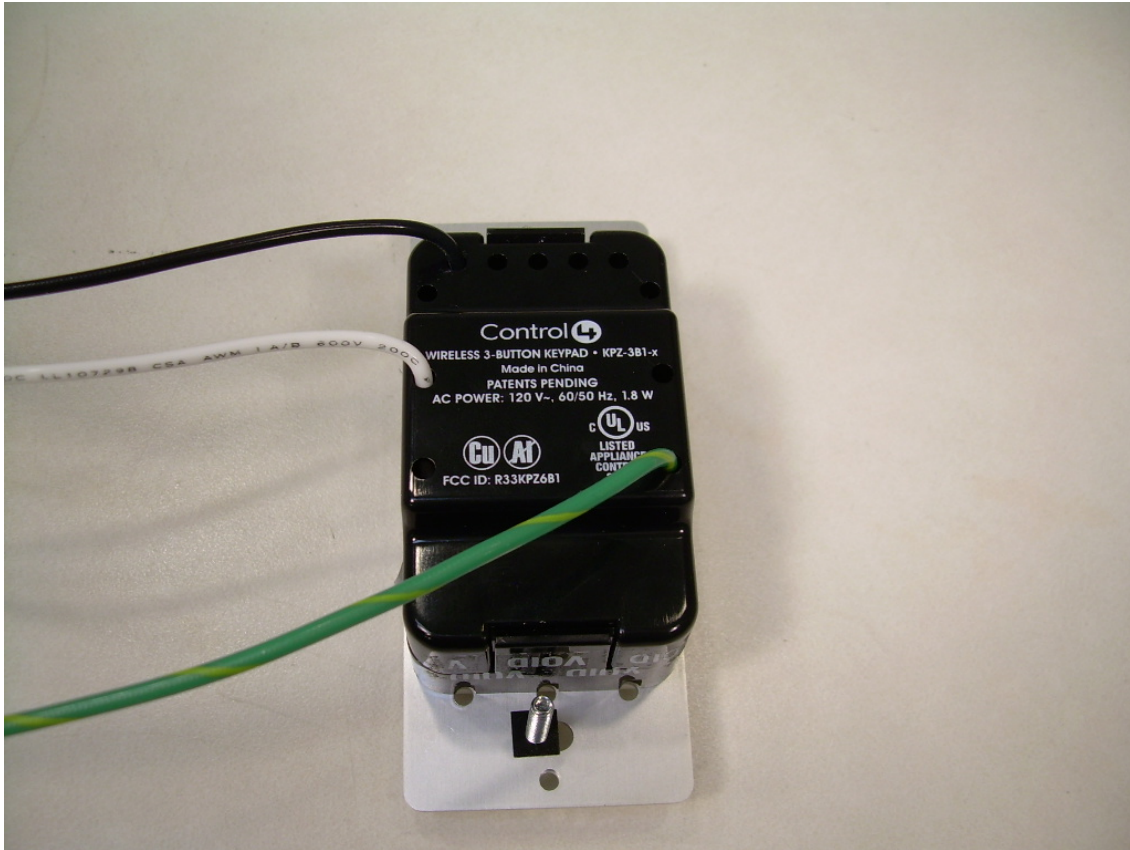
Photograph 6 - Back View of the C4-KP3-Z-x
