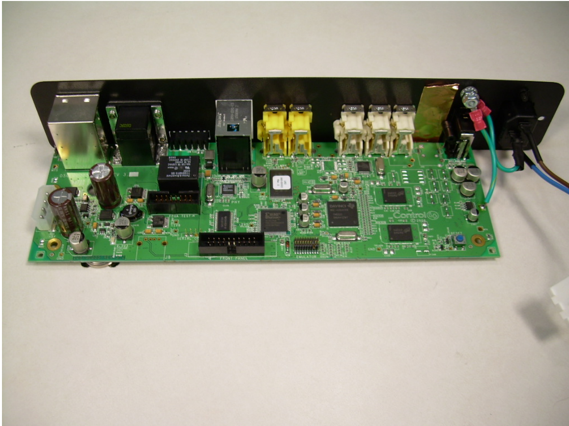
Photograph 8 - Top View of the Main PCB
