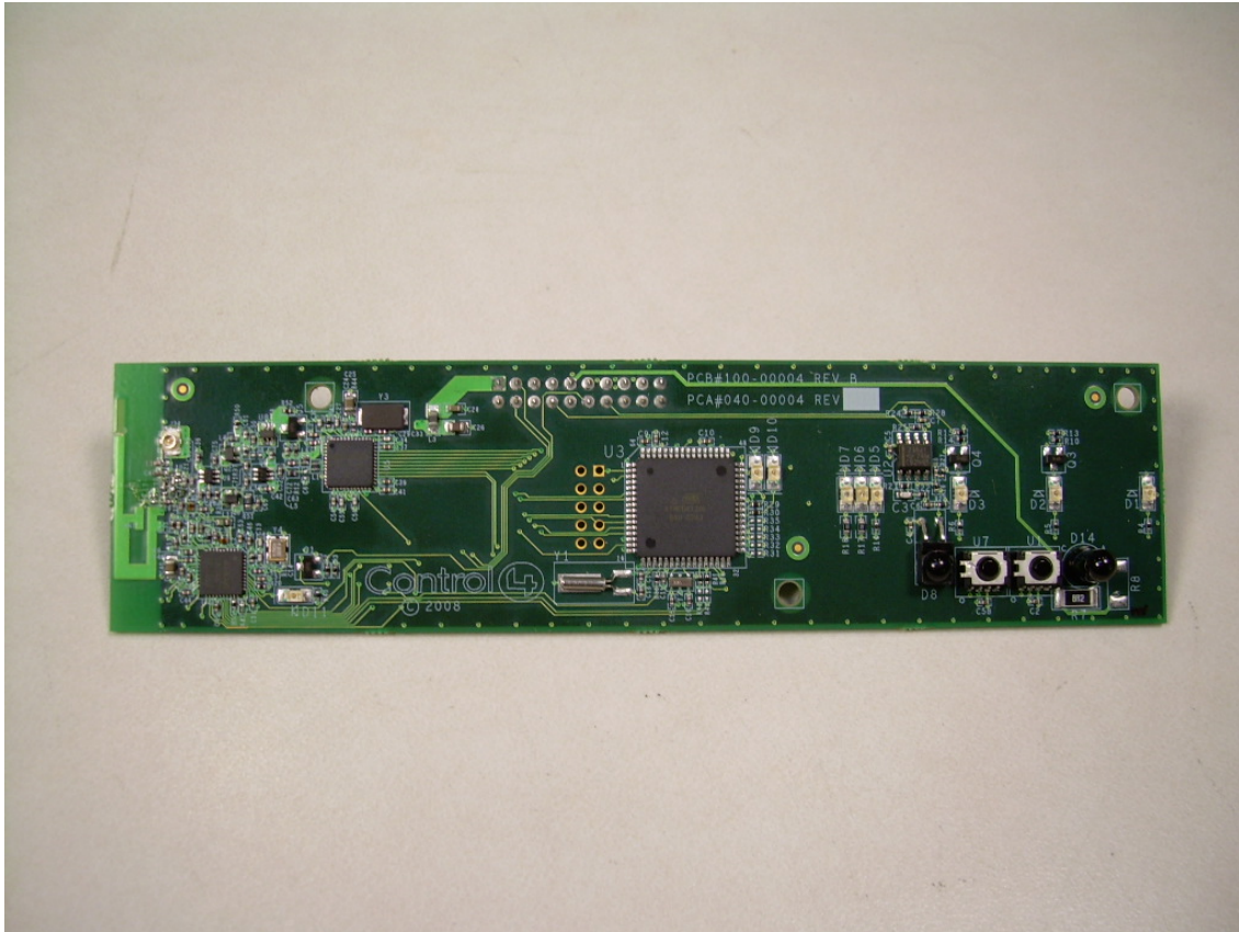
Photograph 10 - Front View of the Front Panel PCB
