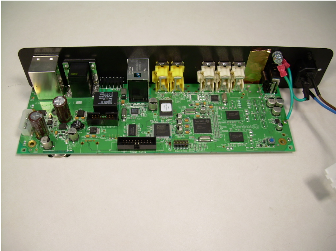
Top View of the Main PCB
