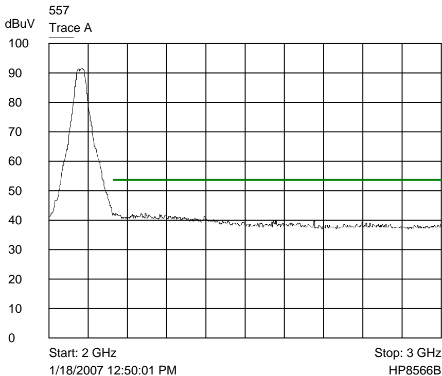
Trace A Upper band edge plot - corrected - radiated
