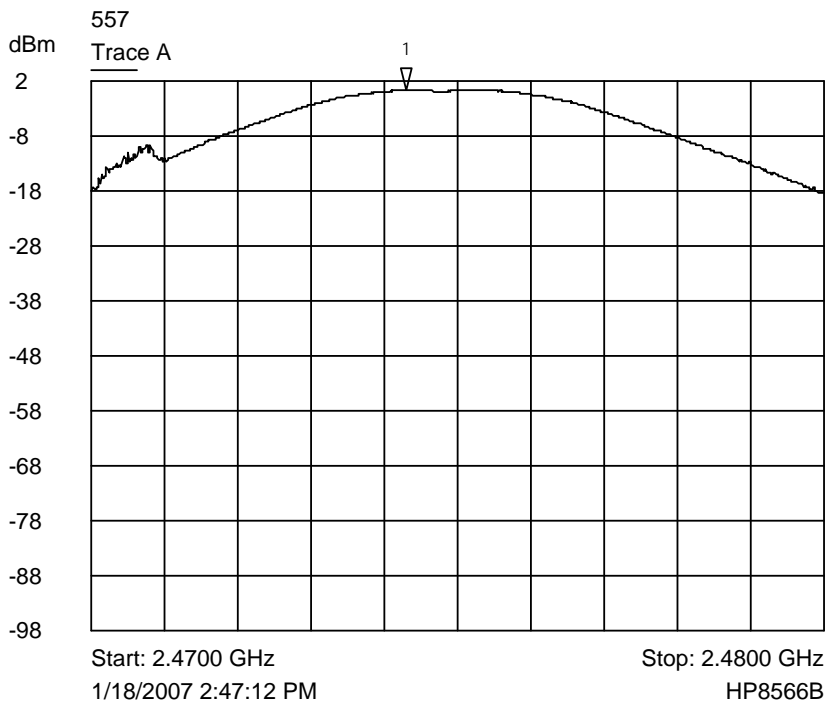
Trace A Upper channel output power
