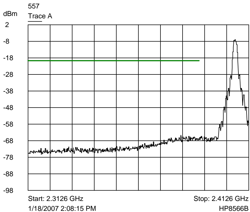
Trace A Lower band edge plot - antenna conducted
