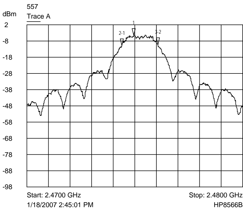
Trace A Upper channel bandwidth
