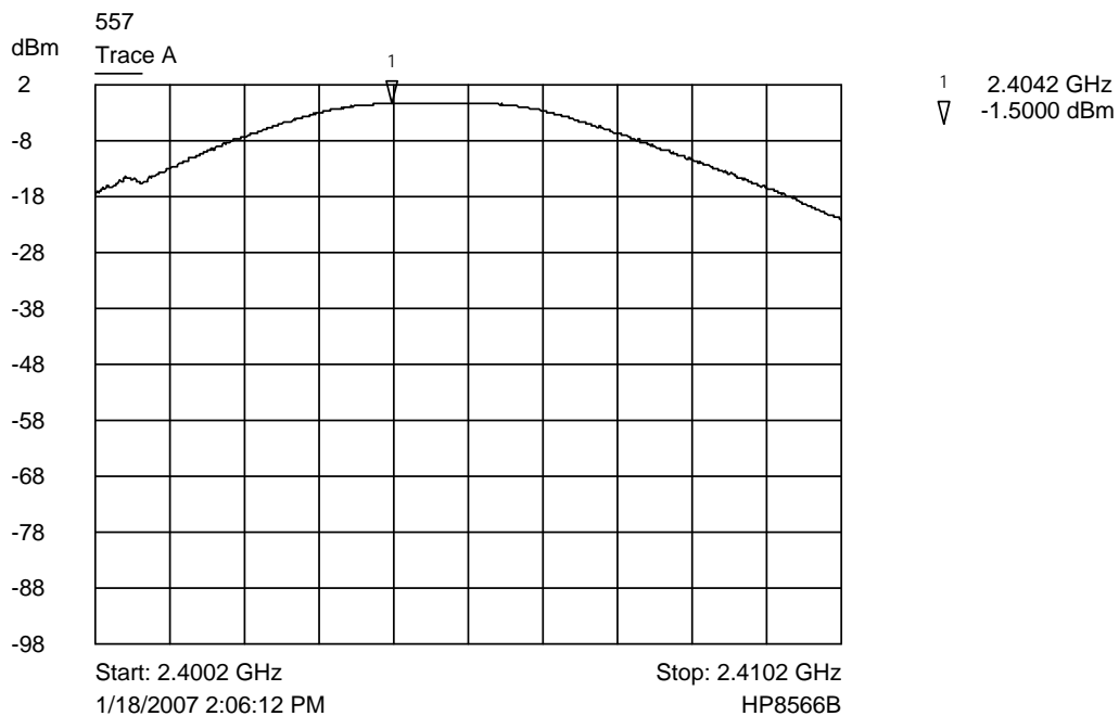
Trace A Lower channel output power plot - antenna conducted
