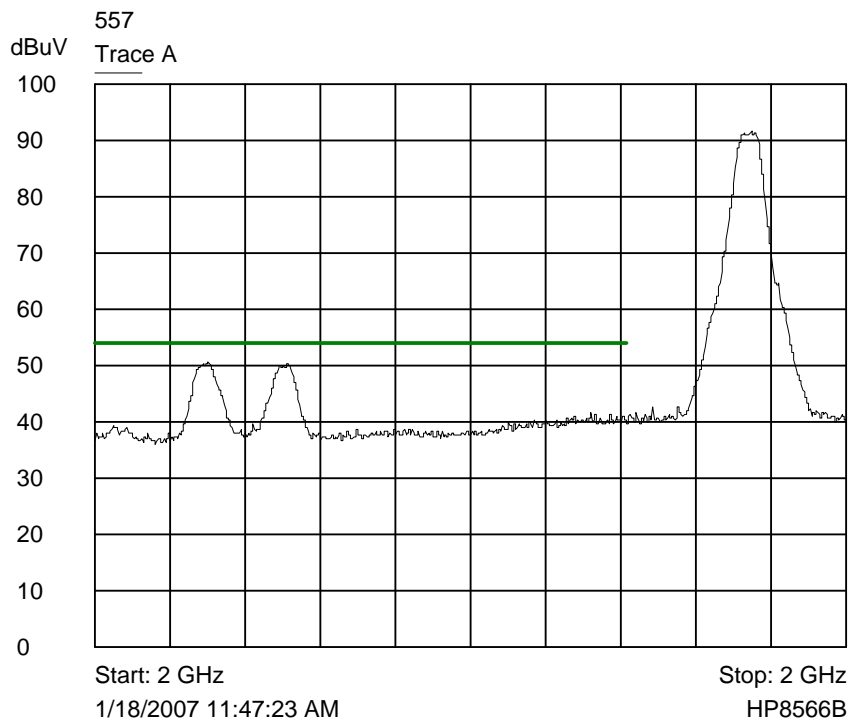
Trace A Lower band edge plot - corrected - radiated
