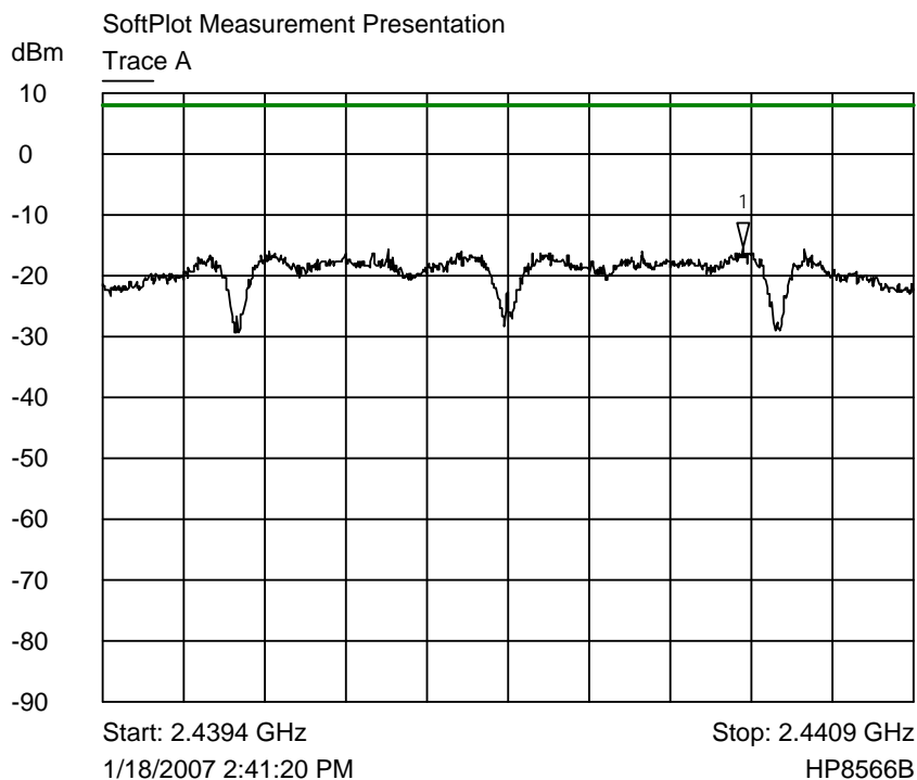
Trace A Middle channel power spectral density plot
