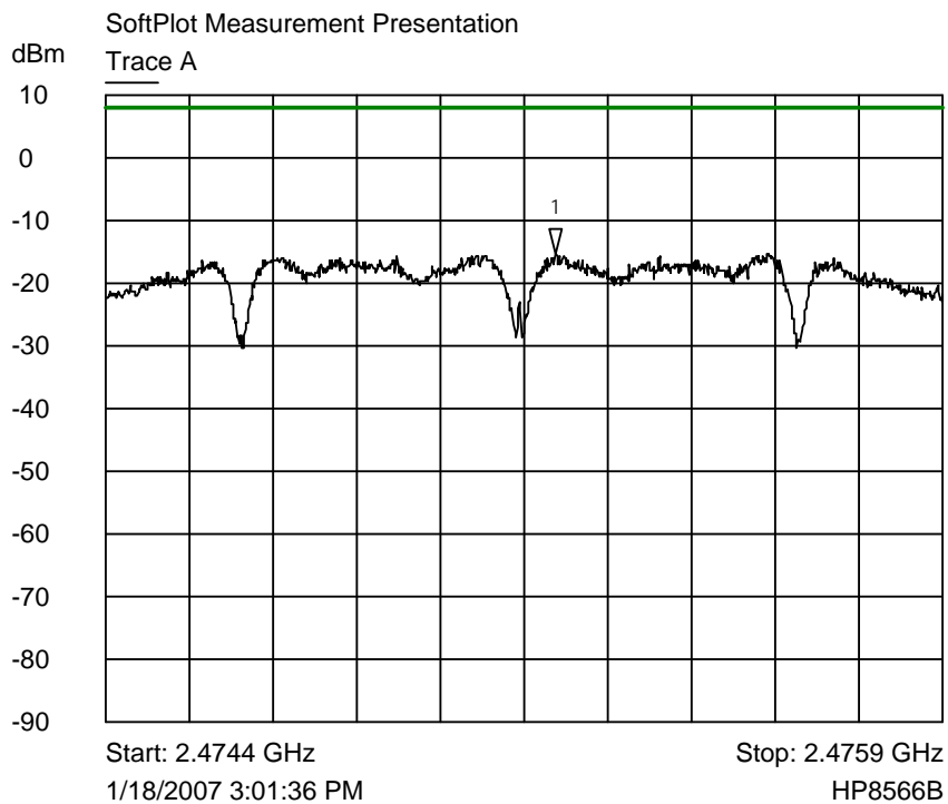
Trace A Upper channel power spectral density plot
