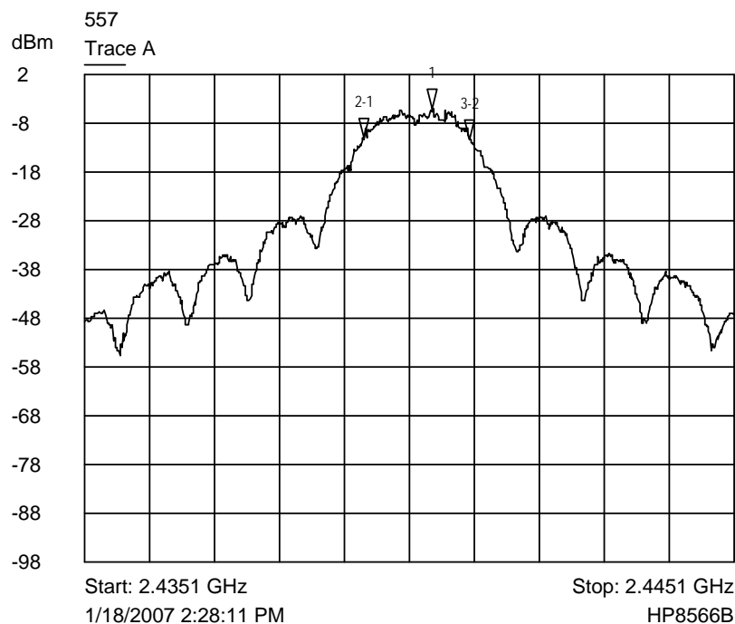
Trace A Middle channel band width plot
