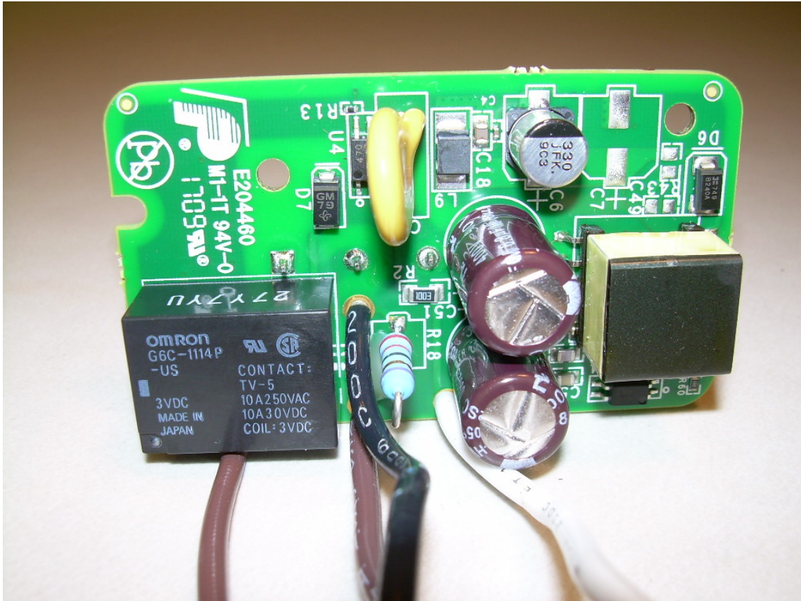
Photograph 8 - Back View of the Main PCB
