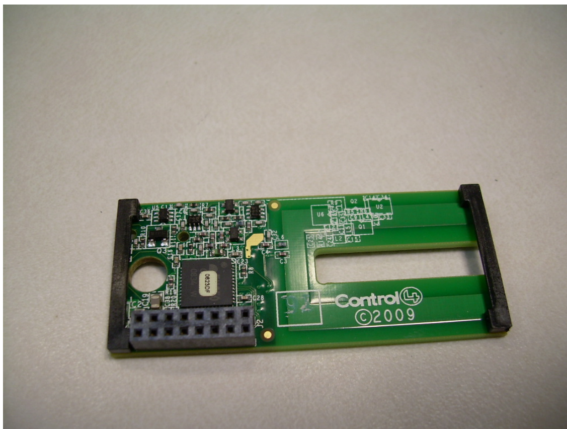
Photograph 10 - Back View of the Transceiver PCB
