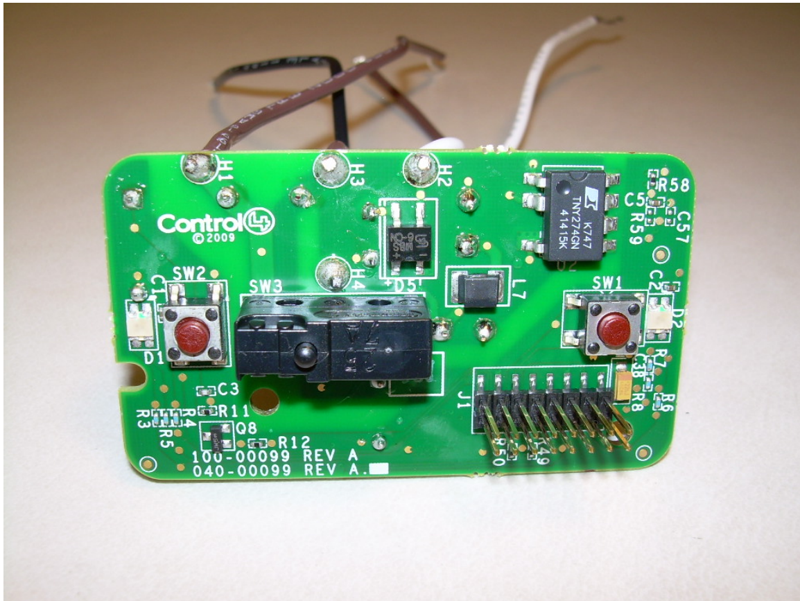
Photograph 7 - Front View of the Main PCB
