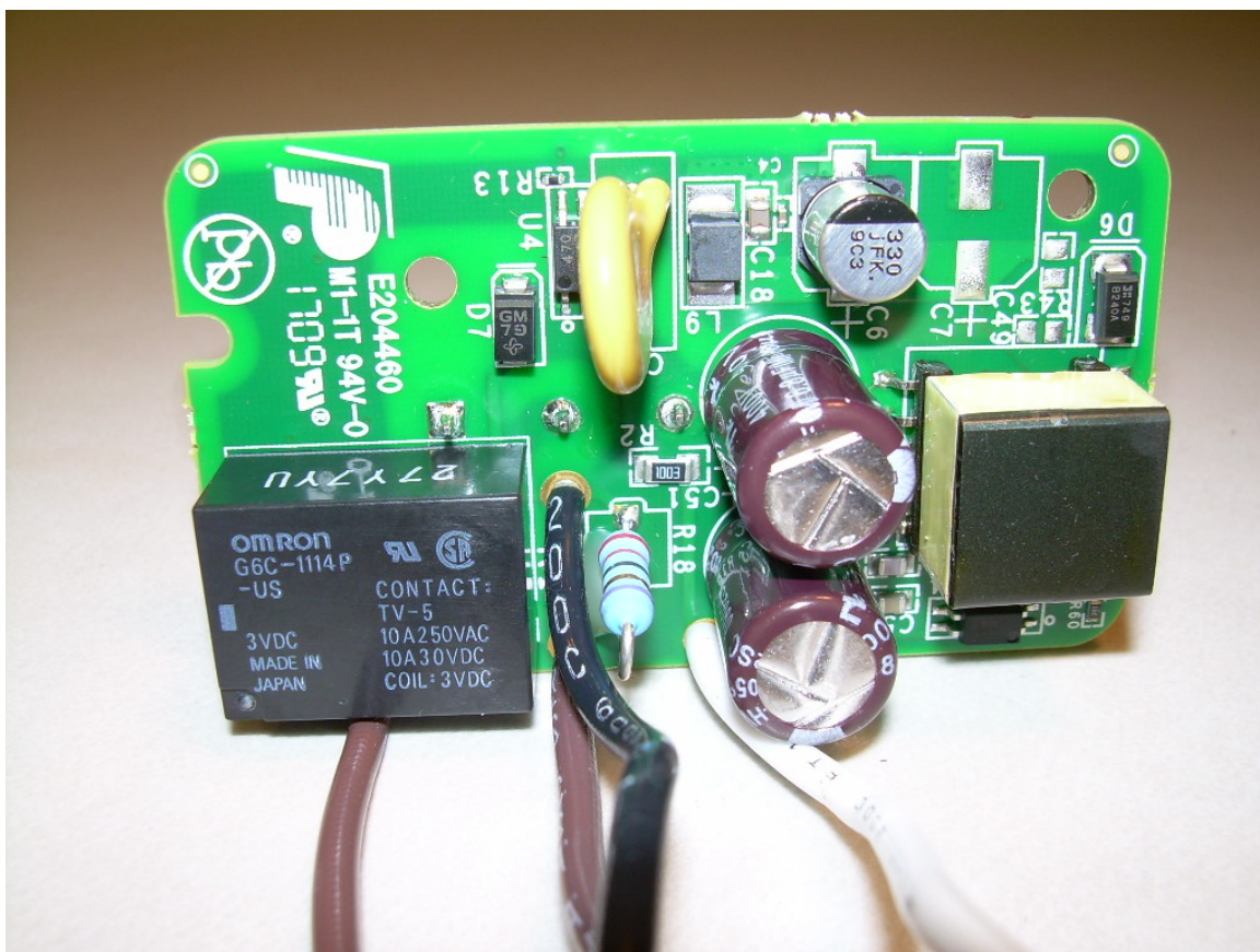
Back View of the Main PCB
