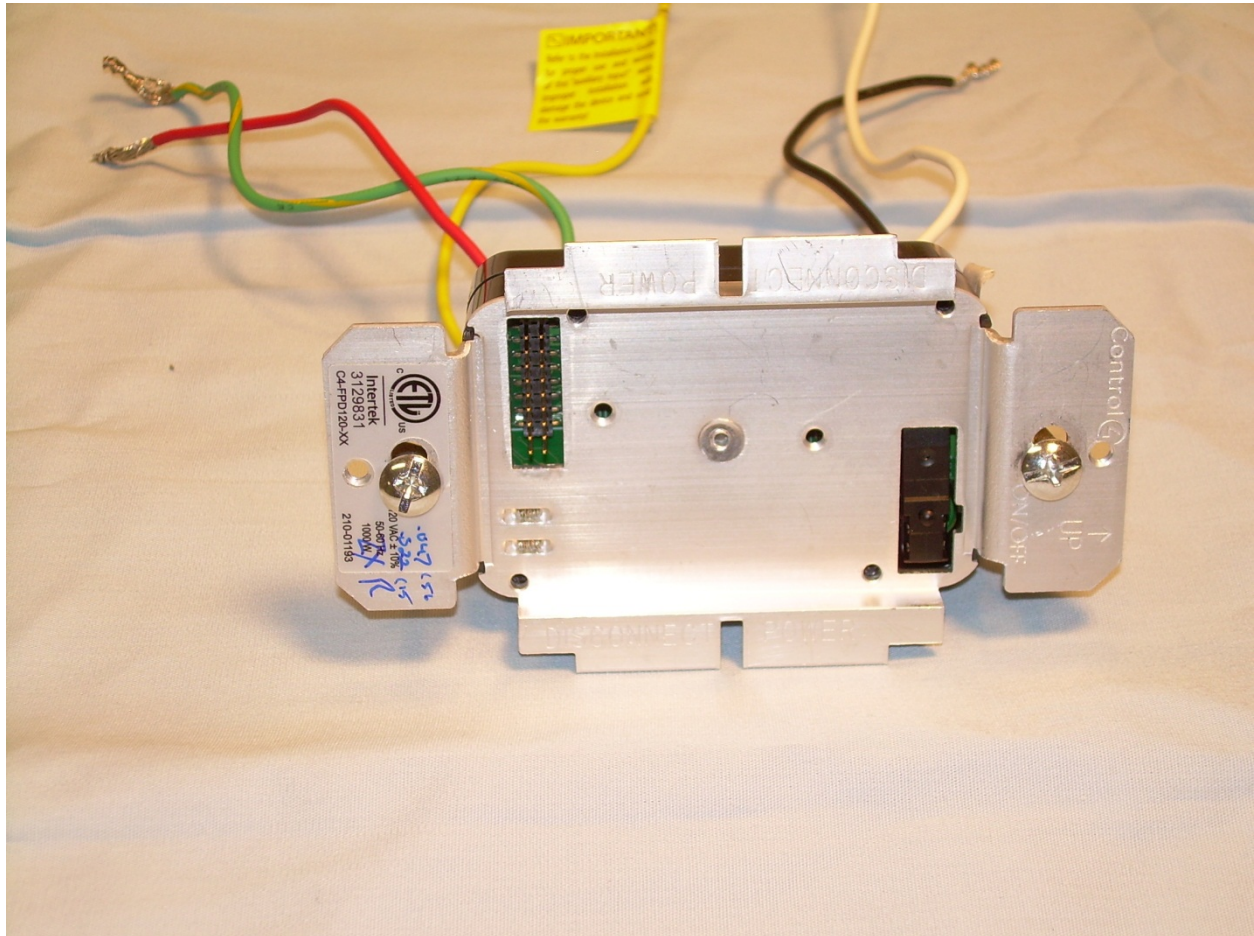
Photograph 10 – View of the C4-FPD120 with RF PCB and Insulator Removed
