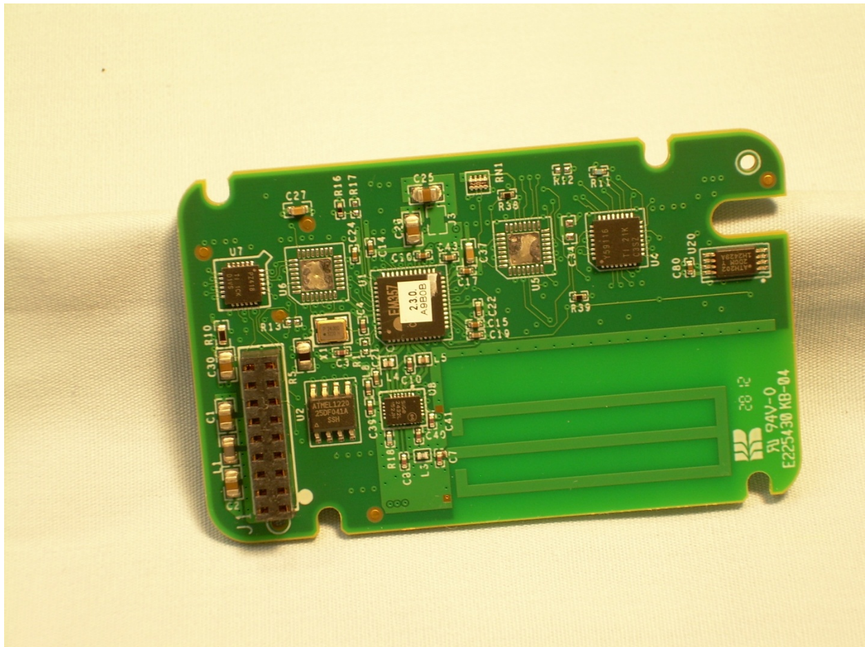
Photograph 14 – View of the Back Side of the C4-FPD120 RF PCB
