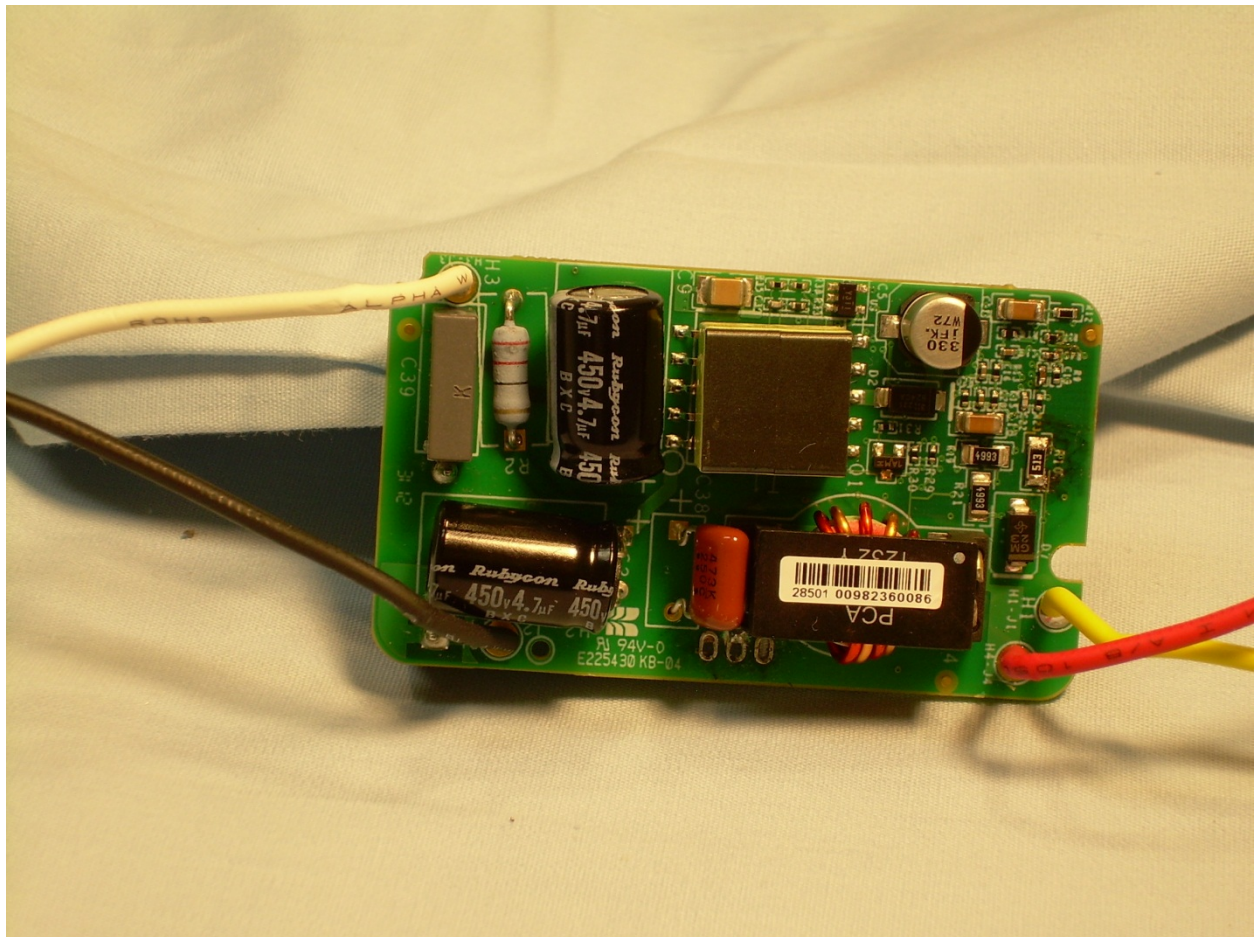
Photograph 16 – View of the Back Side of the C4-FPD120 Main PCB
