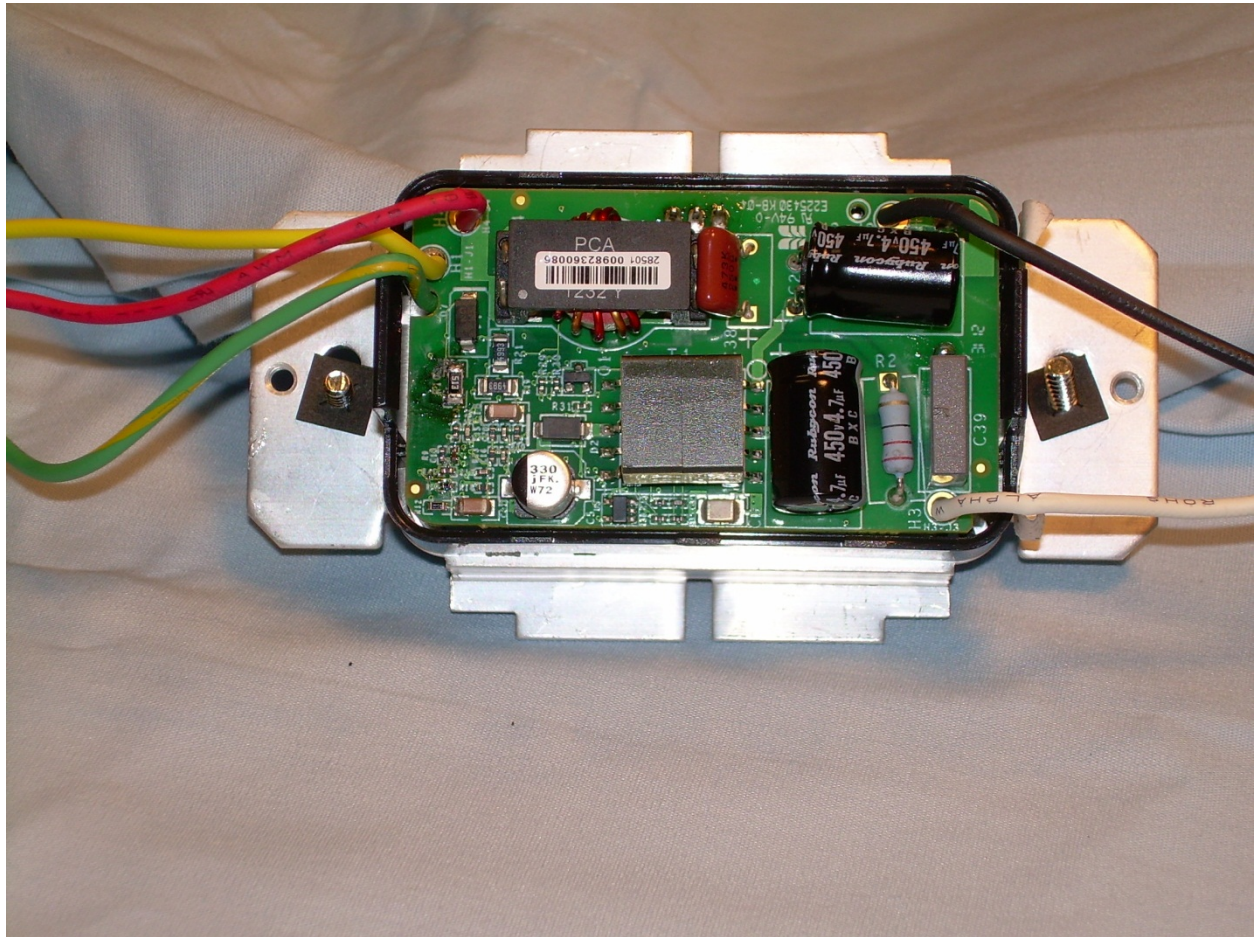
Photograph 11 – View of the C4-FPD120 with Back Cover Removed
