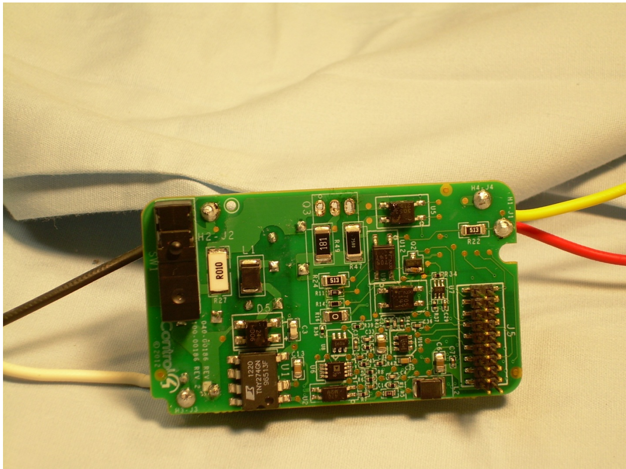
Photograph 15 – View of the Front Side of the C4-FPD120 Main PCB
