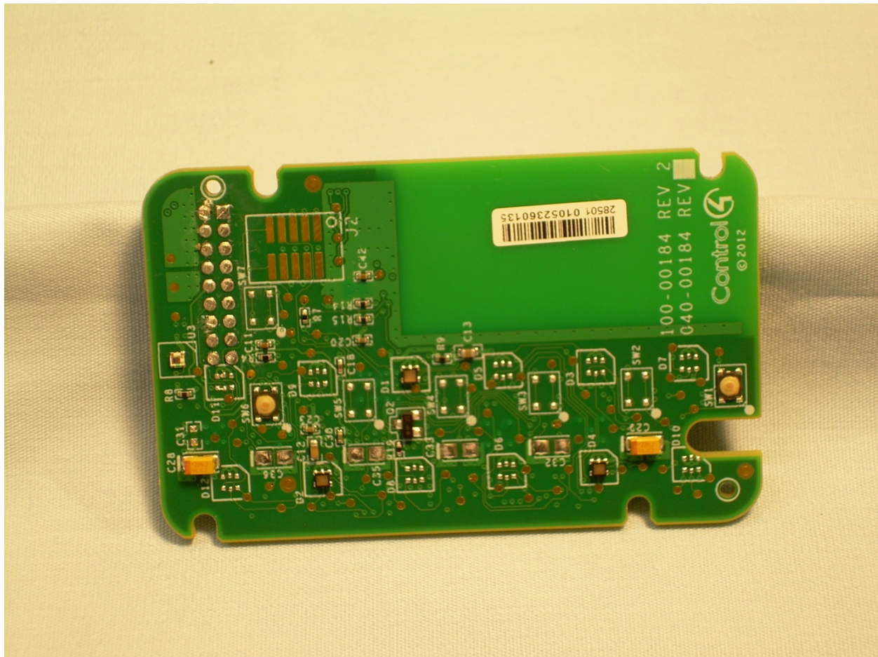
Photograph 13 – View of the Front Side of the C4-FPD120 RF PCB
