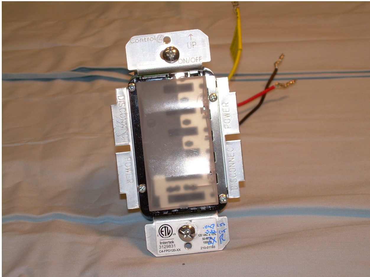
Photograph 5 – Front View of the C4-FPD120
