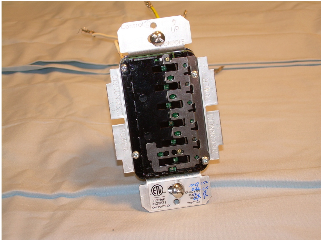
Photograph 7 – View of the C4-PPD120 with Front Cover Removed
