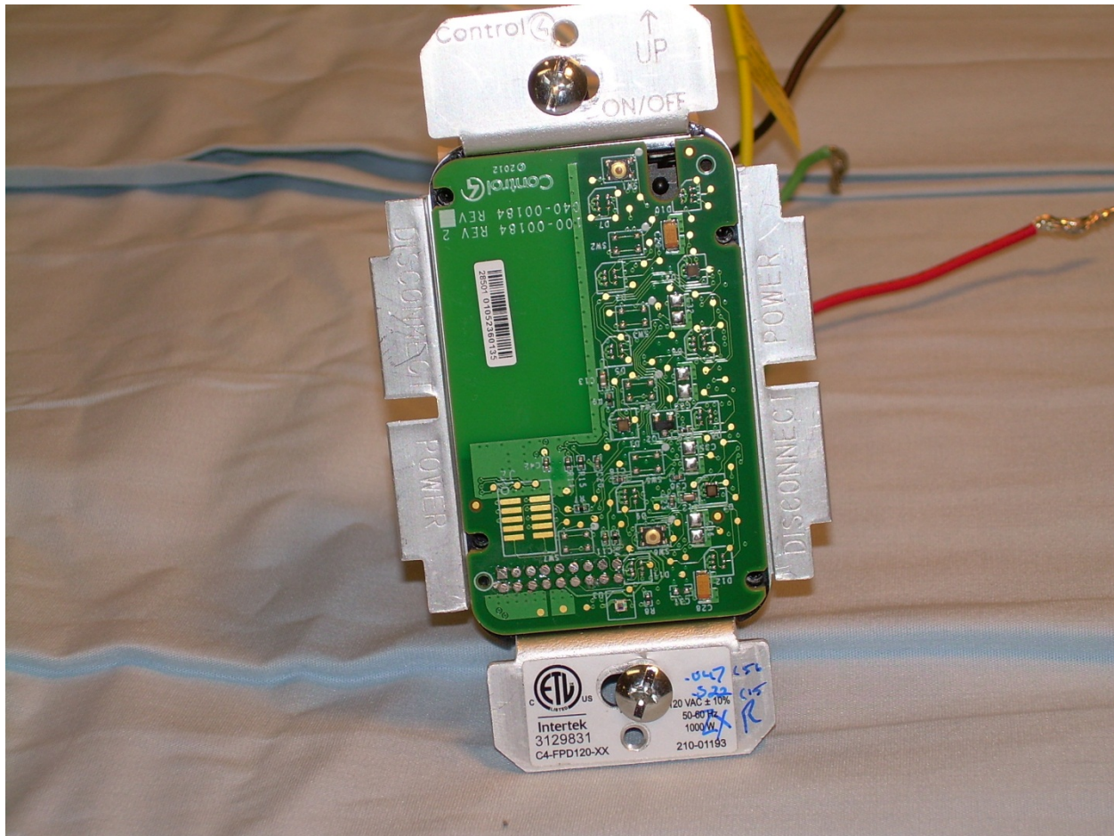
Photograph 8 – View of the C4-FPD120 with Front Panel Removed
