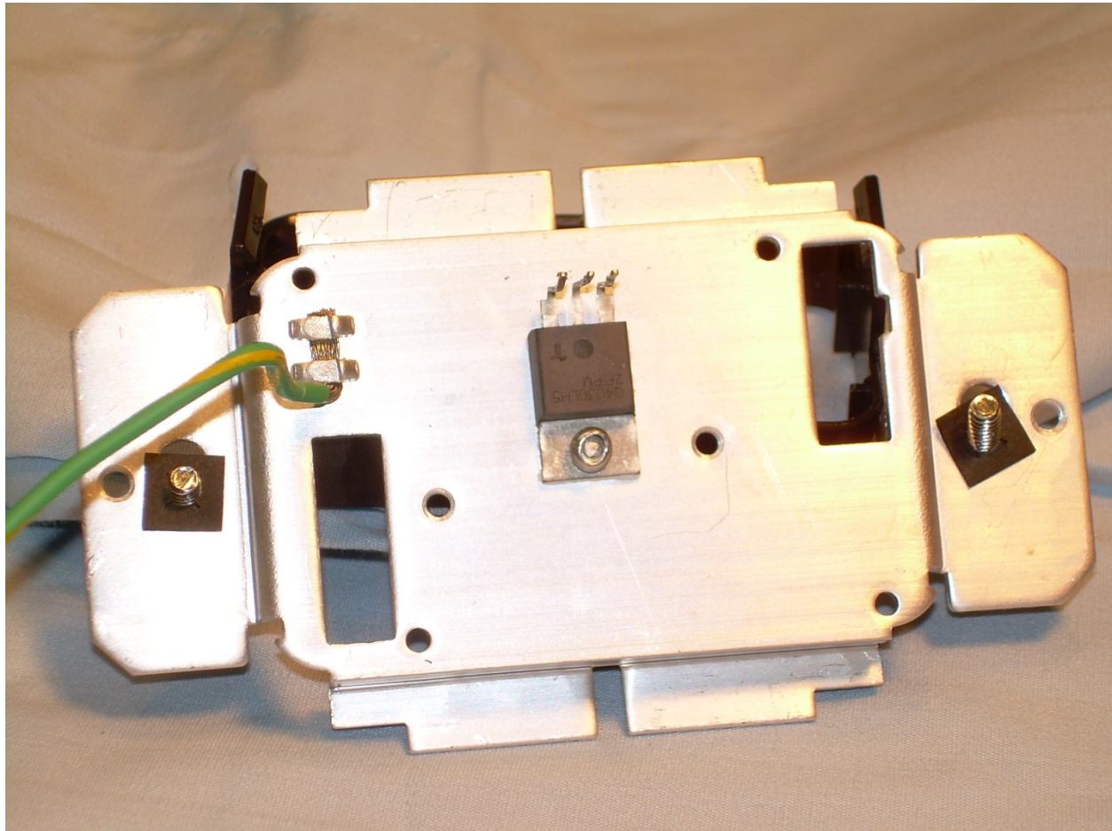
Photograph 12 – View of the C4-FPD120 with Main PCB Removed Showing Triac
