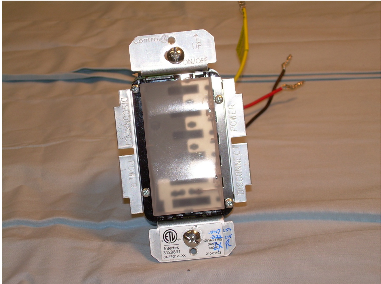
Front View of the C4-FPD120
