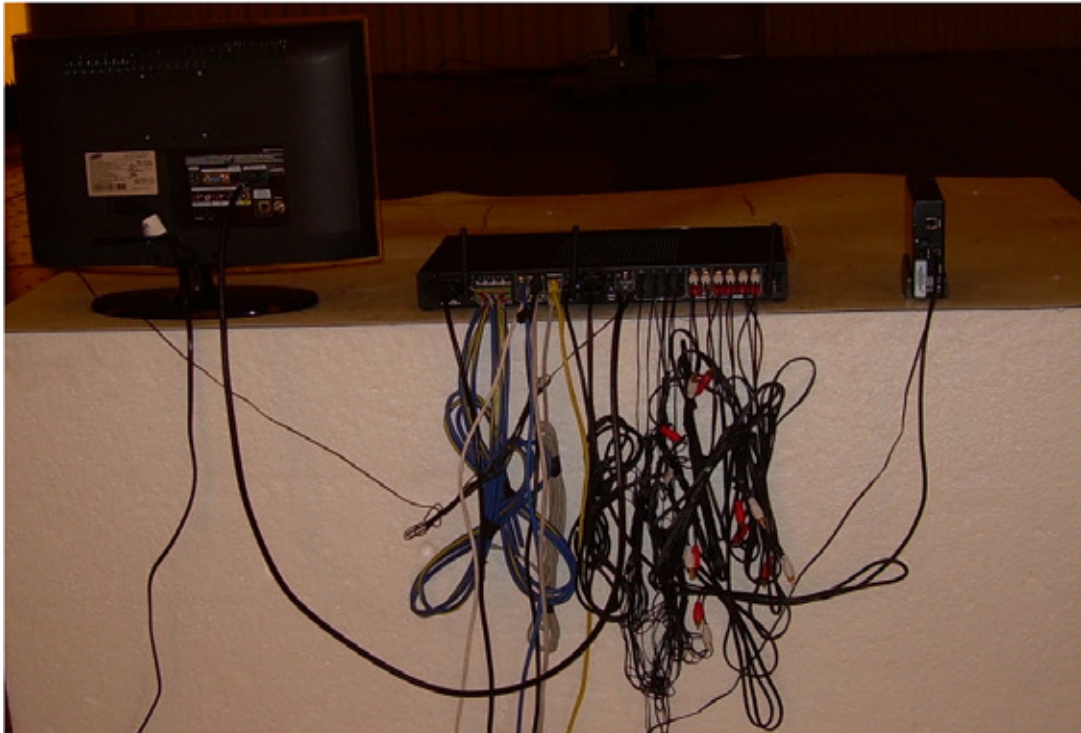
Photograph 2 – Back View of the Radiated Emission Setup
