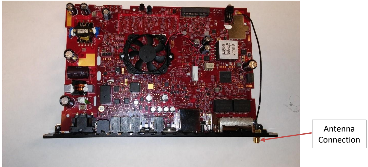
Photograph 1 – Top View of the PCB with Shield
