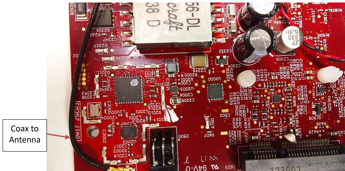
Photograph 2 – Circuitry Under RF Shield
