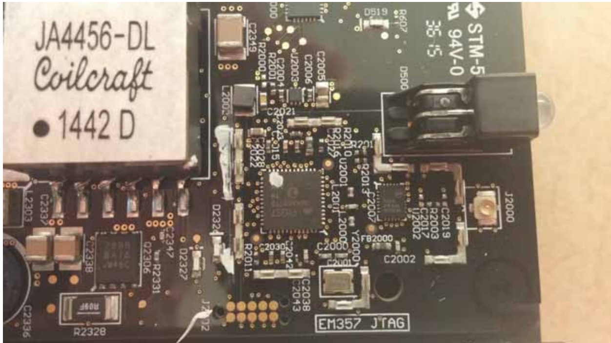
Photograph 10 – View of the Circuitry of the 802.15.4 Transceiver with RF Shield Removed
