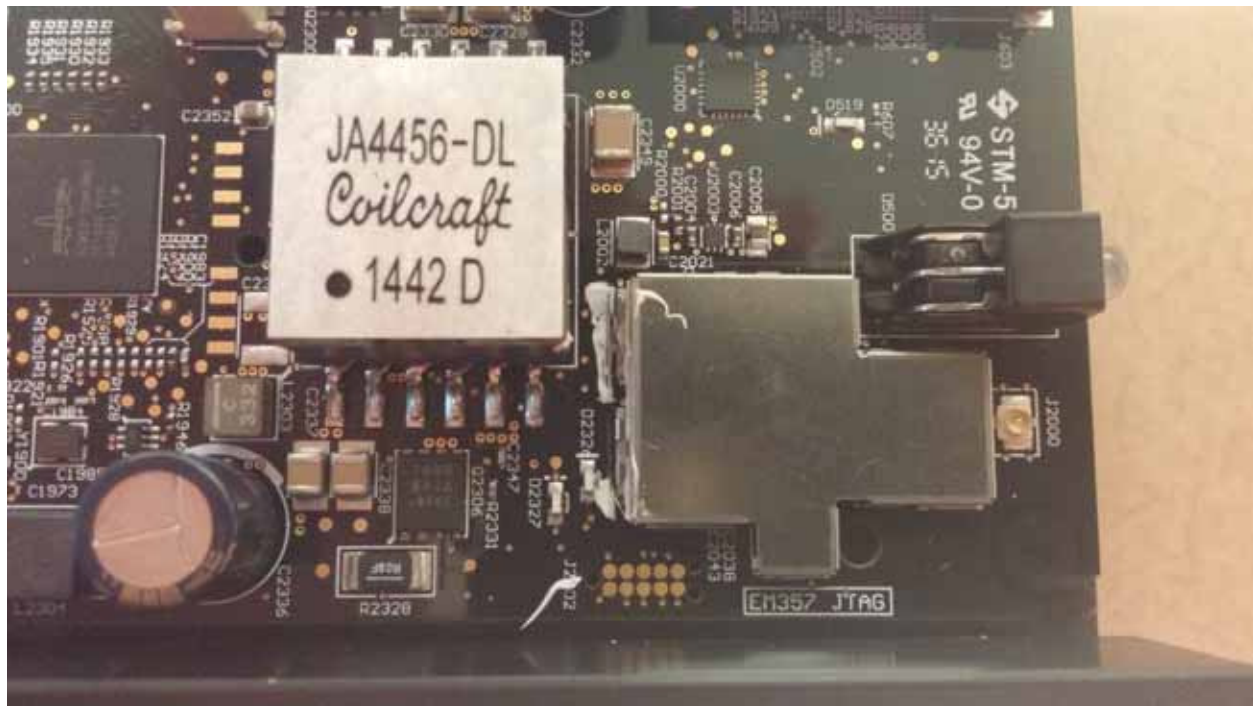
Photograph 9 – View of the 802.15.4 Transceiver Circuitry with RF Shield
