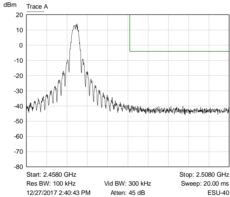
Graph 10: Upper Band Edge Plot (2470 MHz)
