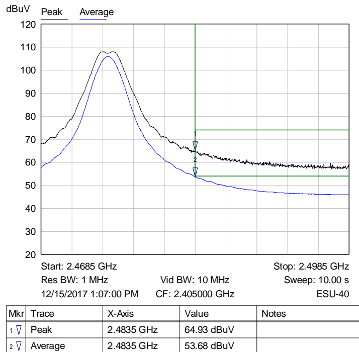
Graph 14: Radiated Upper Band Edge Plot (2475 MHz)
