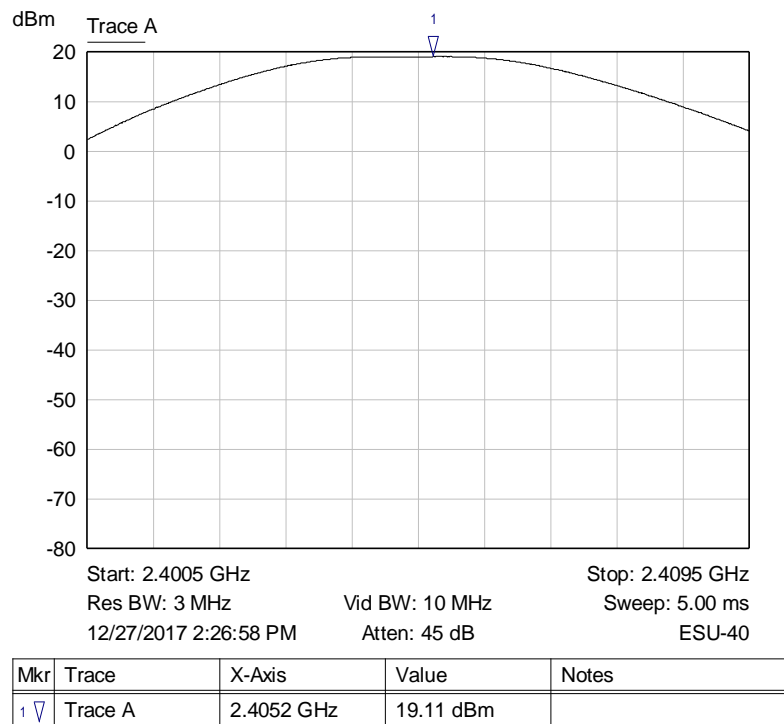
Graph 5: Lowest Channel Output Power Plot (2405 MHz)
