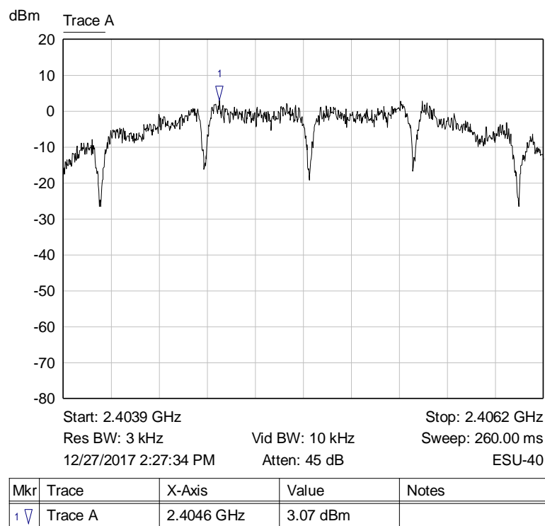
Graph 15: Lowest Channel 3 kHz PSD Plot (2405 MHz)
