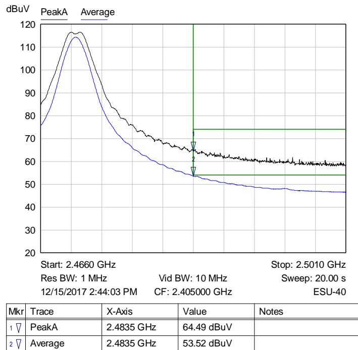
Graph 13: Radiated Upper Band Edge Plot (2470 MHz)
