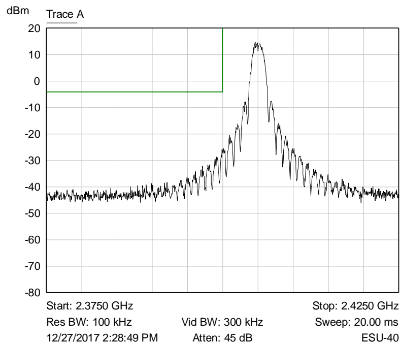
Graph 9: Lower Band Edge Plot (2405 MHz)
