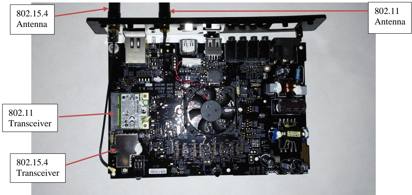
Photograph 10 – Top View of the PCB
