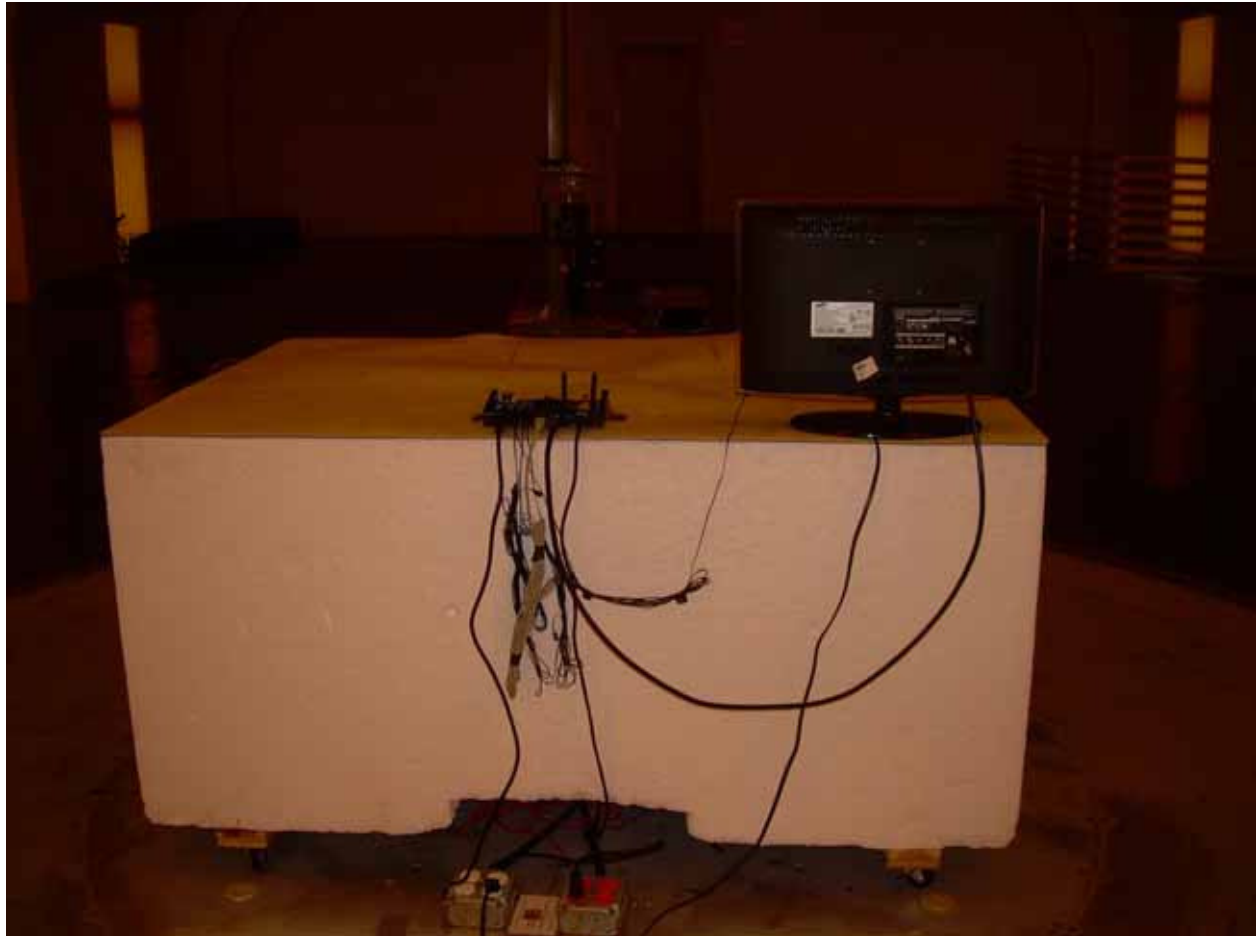
Photograph 2 – Back View Radiated Disturbance Configuration – Oxford TEC Antenna
