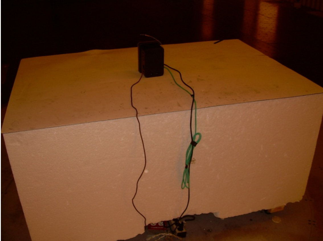
Photograph 2 – Back View Radiated Disturbance Worst Case Configuration – DC Powered
