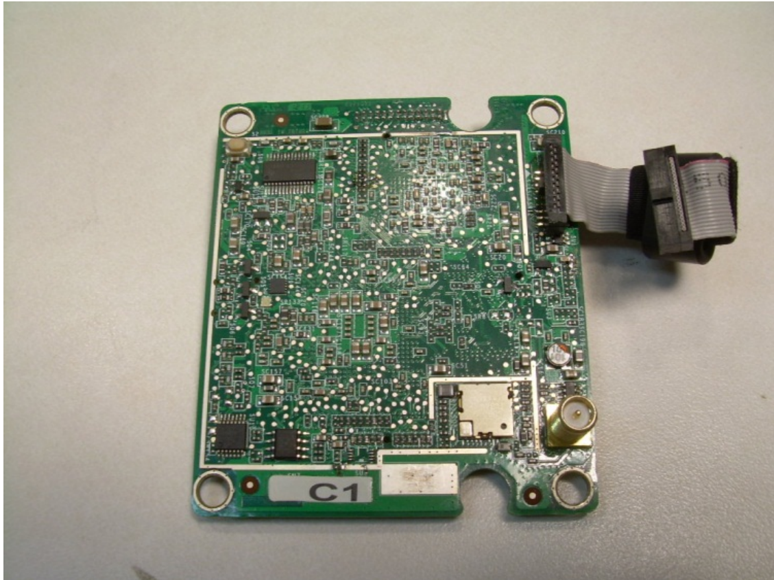
Photograph 23 – View of the Trace Side of the Main/RF PCB
