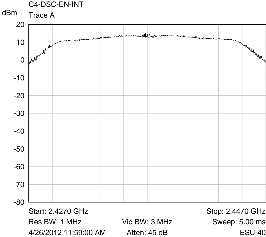
Trace A Output power
