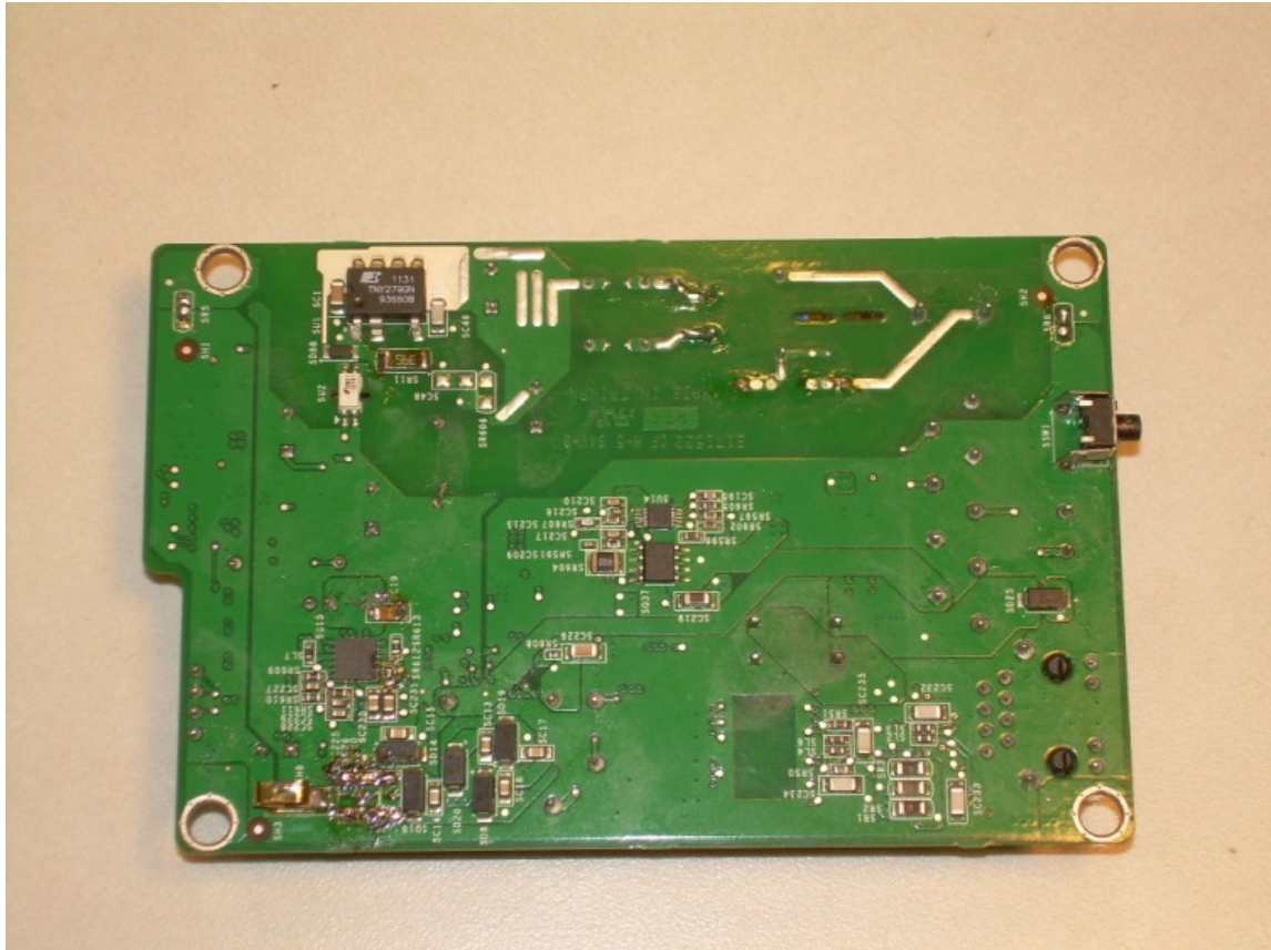
Photograph 20 – View of the Trace Side of the Power PCB
