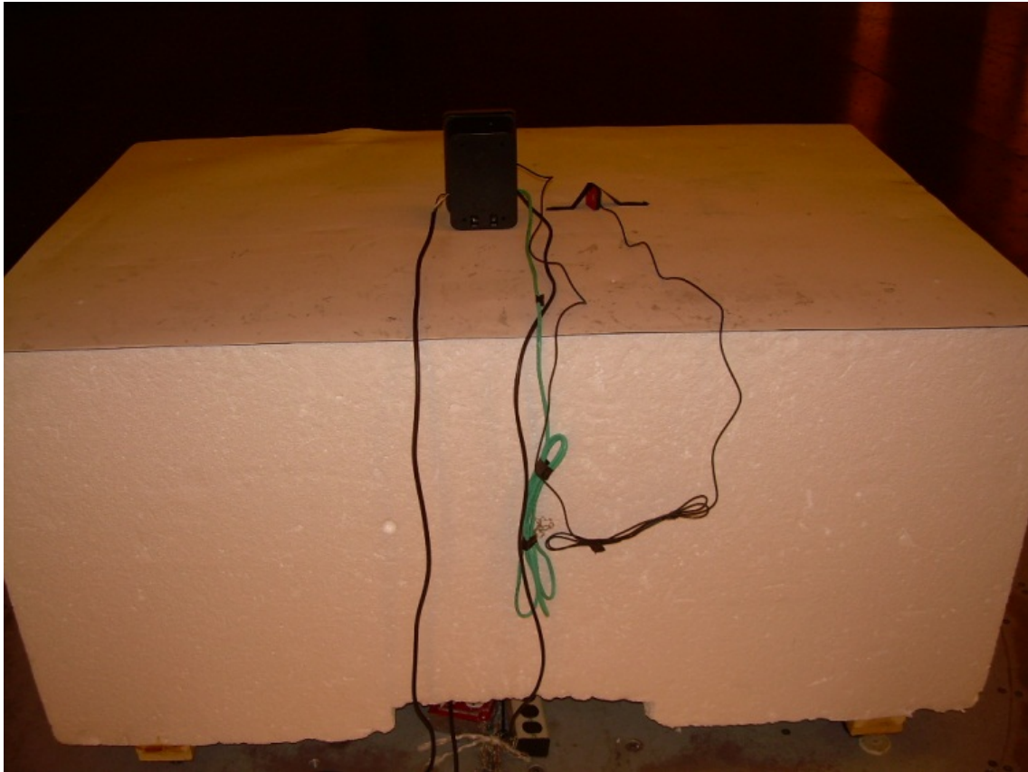
Photograph 7 – Back View Showing Worst-Case Patch Antenna Placement
