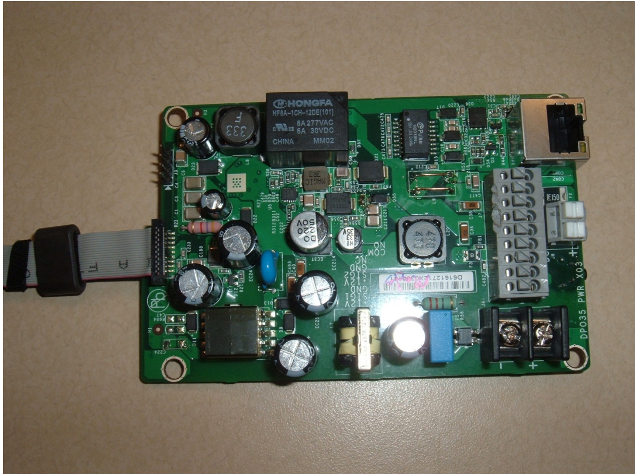
Photograph 19 – View of the Component Side of the Power PCB
