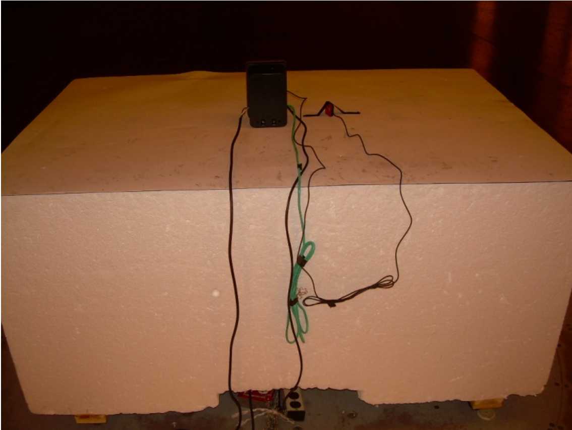
View Showing Worst-Case Patch Antenna Placement
