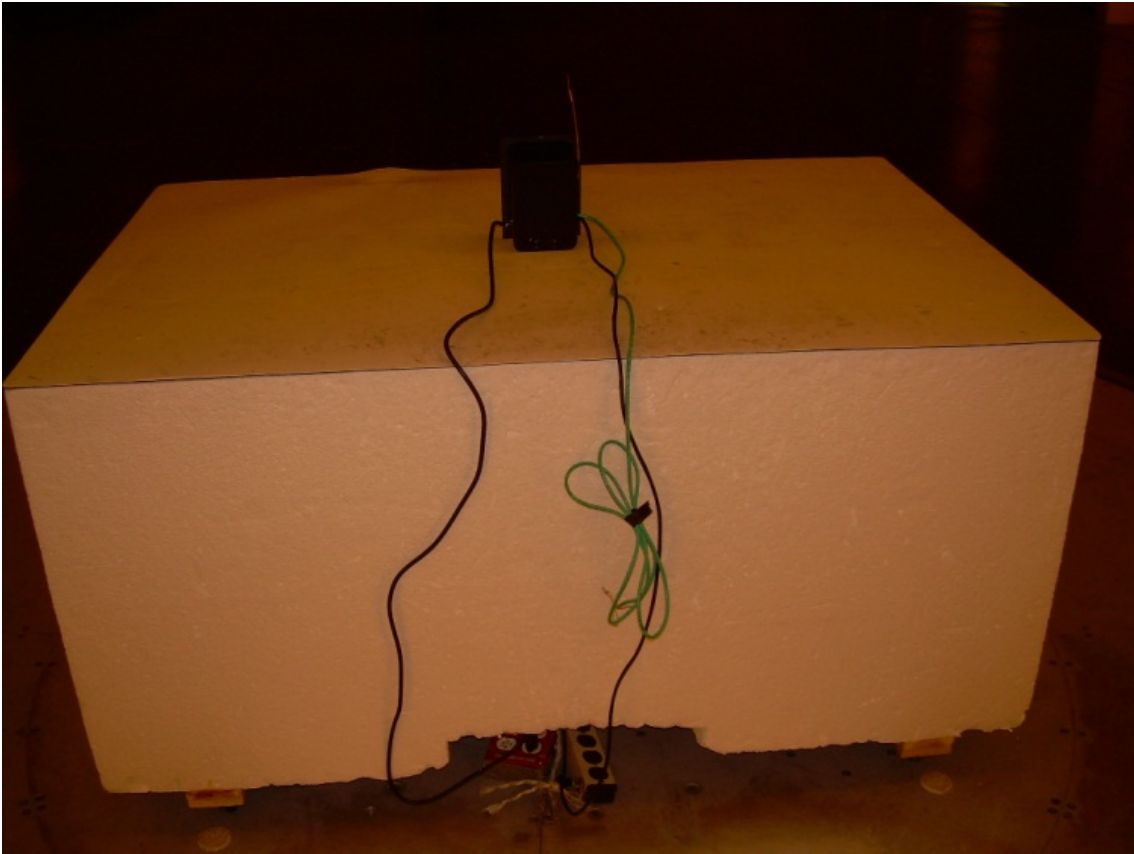
Back View Radiated Disturbance – AC Power
