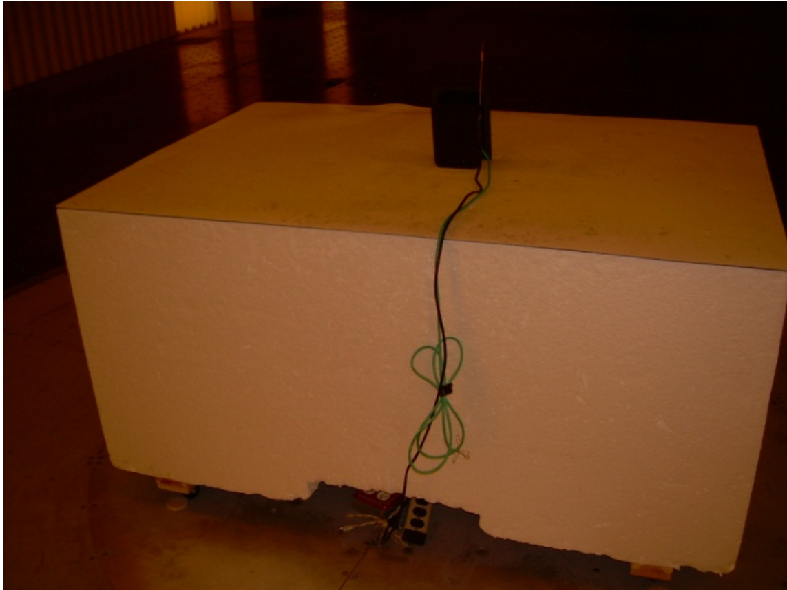
Back View Radiated Disturbance Worst Case Configuration – POE Power
