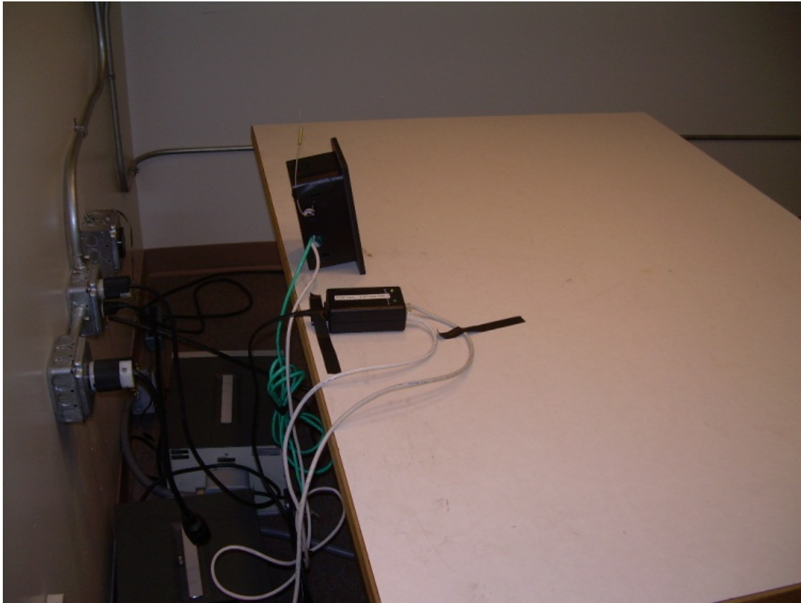
Back View Conducted Disturbance Worst Case Configuration – POE Power
