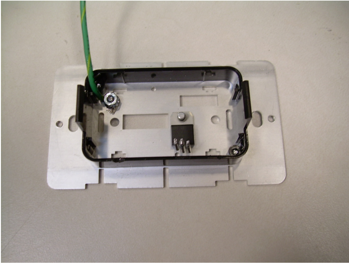
View of the Triac Mounting
