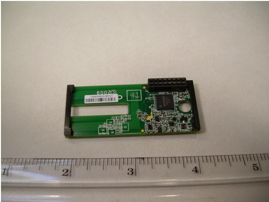
Back View of the Transceiver PCB
