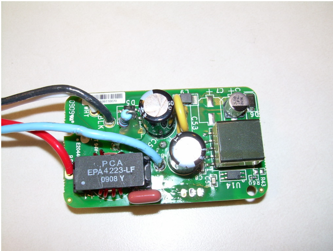
View of the Back of the Main Dimmer PCB
