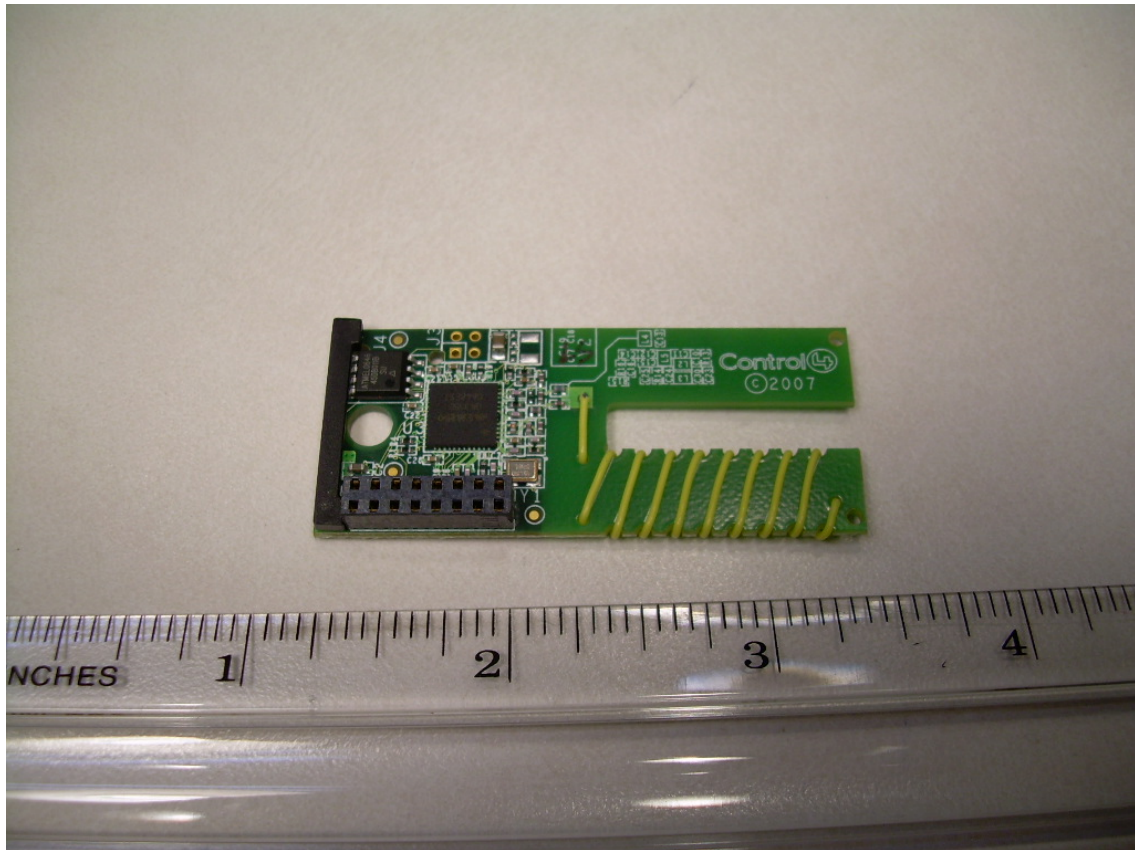
Back Side of the Transceiver PCB
