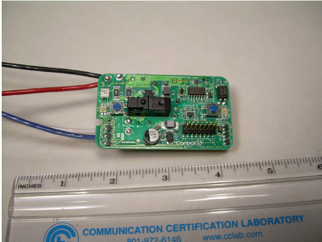
Trace Side of the Dimmer PCB
