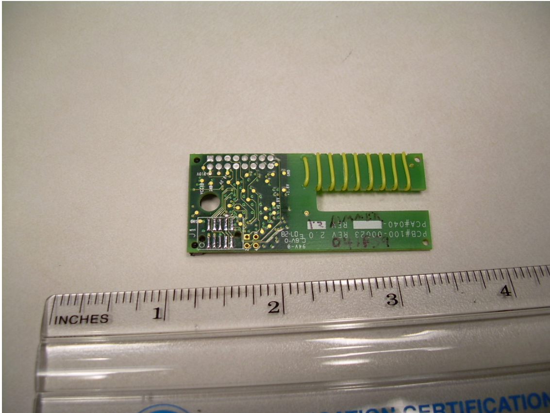
Front Side of the Transceiver PCB
