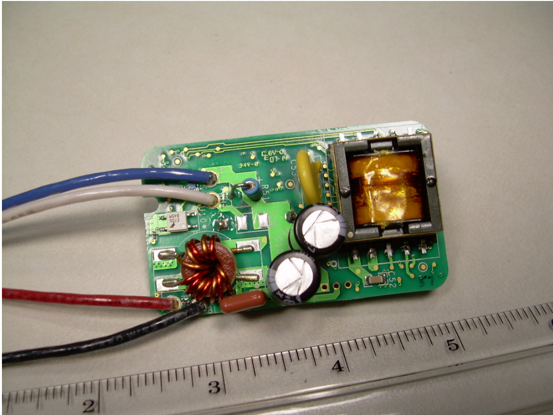
Component Side of the Dimmer PCB
