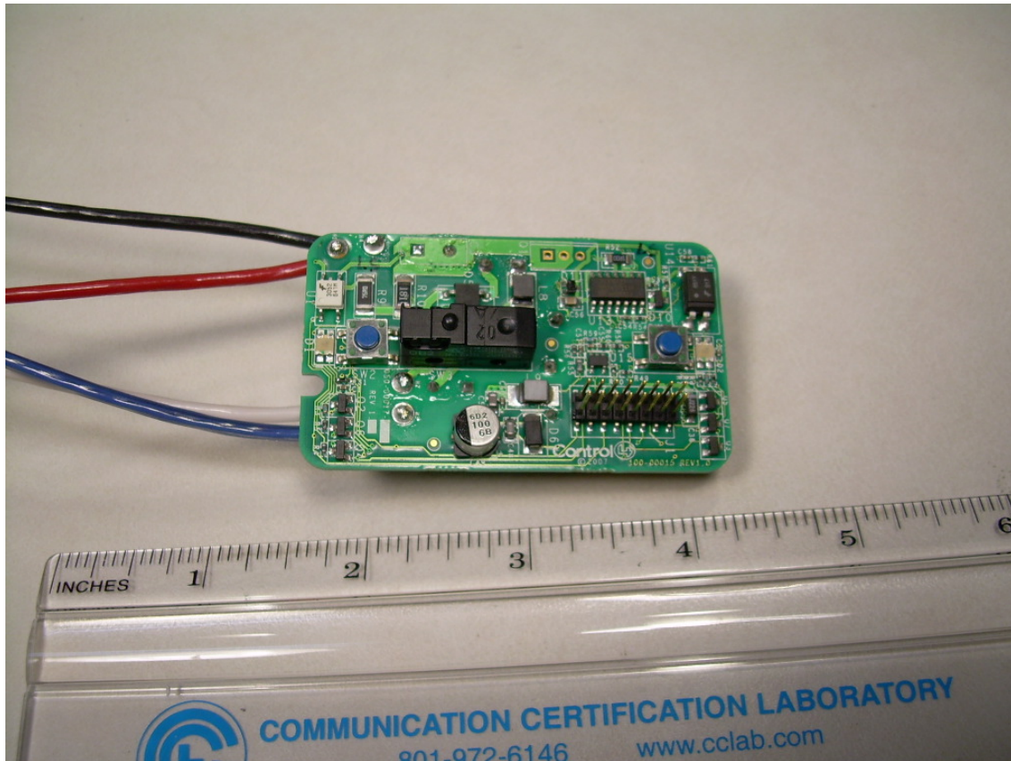
Photograph 8 - Trace Side of the Dimmer PCB
