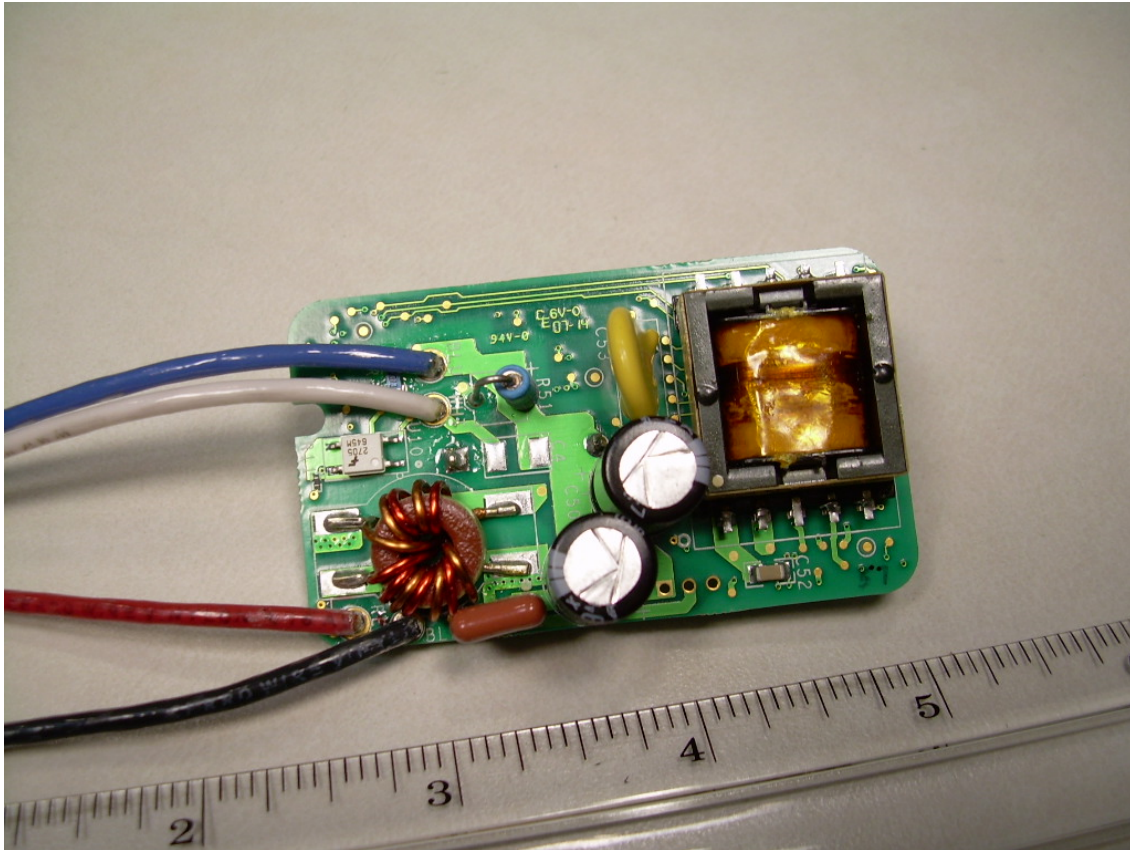
Photograph 7 - Component Side of the Dimmer PCB
