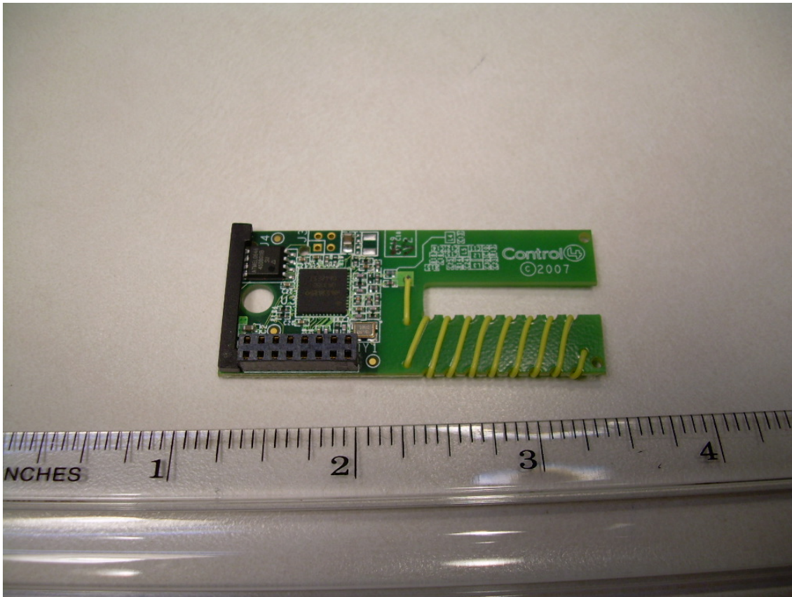
Photograph 10 - Back Side of the Transceiver PCB
