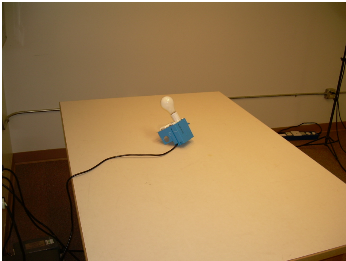
Back View Conducted Disturbance Configuration
